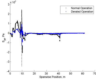
Figure 5: Stress results for \sigma_{yz} along the bond line for the baseline model during normal operation and derated to 50% power level.
