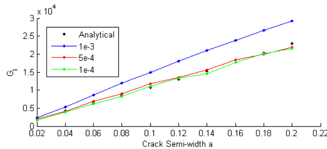
Figure 2: VCCT results for rectangular sample with horizontal mid-plane crack.
