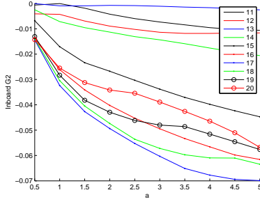
Figure 10: SERR for Mode II fracture of the inner crack tip for various starting positions (11 – 20 m) and crack lengths (0.5 – 5 m), normal operation, rated windspeed.
