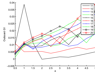
Figure 9: SERR for Mode I fracture of outer crack tip for various starting positions (11 – 20 m) and crack lengths (0.5 – 5 m), normal operation, rated windspeed.
