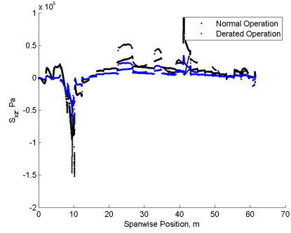
Figure 6: Stress results for \sigma_{xz} along the bond line for the baseline model during normal operation and derated to 50% power level.
