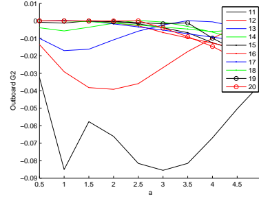
Figure 11: SERR for Mode II fracture of the outer crack tip for various starting positions (11 – 20 m) and crack lengths (0.5 – 5 m), normal operation, rated windspeed.
