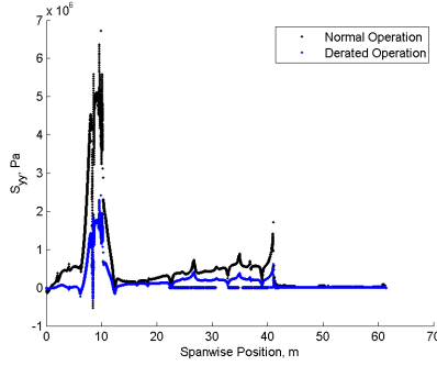
Figure 3: Stress results for \sigma_{yy} along the bond line for the baseline model during normal operation and derated to 50% power level.
