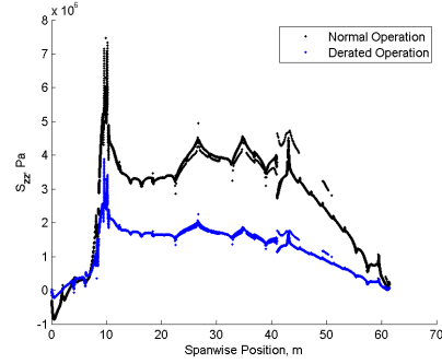
Figure 4: Stress results for \sigma_{zz} along the bond line for the baseline model during normal operation and derated to 50% power level.
