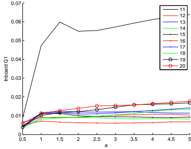
Figure 8: SERR for Mode I fracture of the inner crack tip for various starting positions (11 – 20 m) and crack lengths (0.5 – 5 m), normal operation, rated windspeed.
