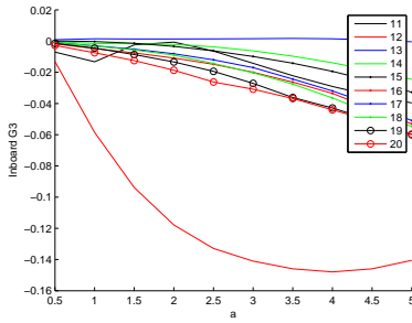
Figure 12: SERR for Mode III fracture of the inner crack tip for various starting positions (11 – 20 m) and crack lengths (0.5 – 5 m), normal operation, rated windspeed.
