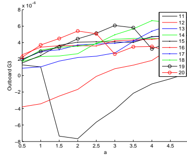
Figure 13: SERR for Mode III fracture of the outer crack tip for various starting positions (11 – 20 m) and crack lengths (0.5 – 5 m), normal operation, rated windspeed.
