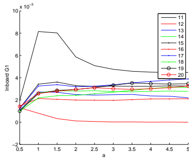
Figure 14: SERR for Mode I fracture of the inner crack tip for various starting positions (11 – 20 m) and crack lengths (0.5 – 5 m), derated operation, rated windspeed.
