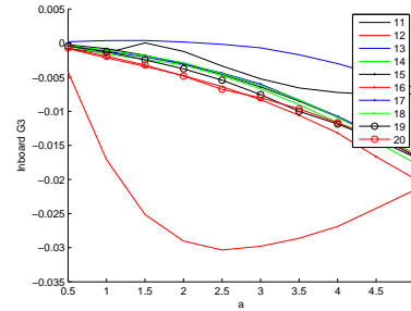
Figure 15: SERR for Mode III fracture of the inner crack tip for various starting positions (11 – 20 m) and crack lengths (0.5 – 5 m), derated operation, rated windspeed.
