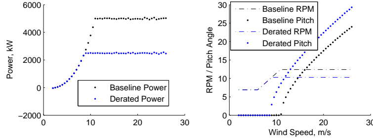
Figure 1: Derated (50% power level) power production, control scheduling, and root bending moment compared with normal/baseline operation.
