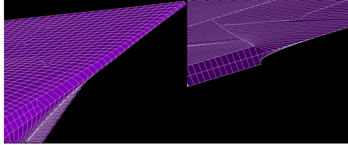
Figure 7: Geometry transitions from circular cross sections to airfoil sections with blunt trailing edges (left) and transition from blunt trailing edges to sharp trailing edges (right).
