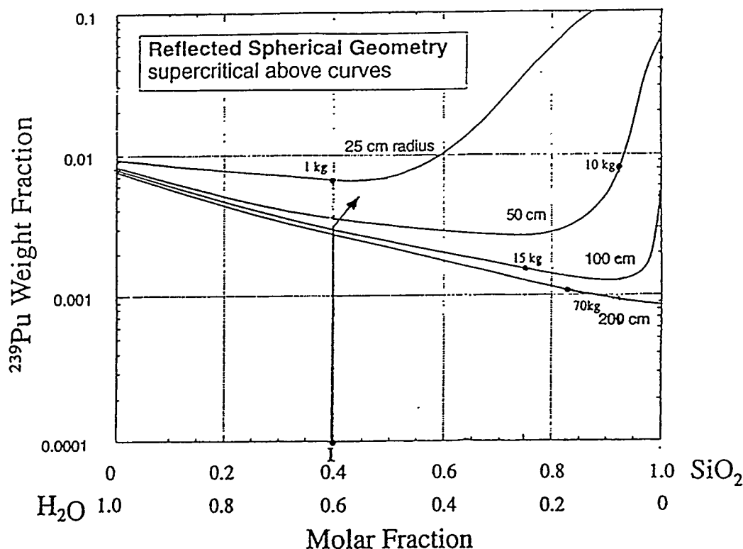
Figure 1. Criticality curves for spheres of Pu239 diluted with water and silicon dioxide and surrounded by silicon dioxide [Bowman and Venneri 1994]. The line "T" illustrates how a critical assembly can be created inside a comet by implantation of Pu239, and the arrow extending from the end of the line shows qualitatively how the resulting autocatalytic assembly would subsequently evolve.
