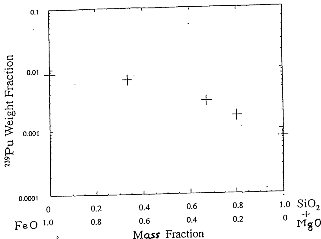
Figure 2. Criticality curve for a 2 meter radius sphere of Pu239 diluted with a mixture of iron oxide, magnesium oxide, and silicon dioxide and surrounded by silicon dioxide.
