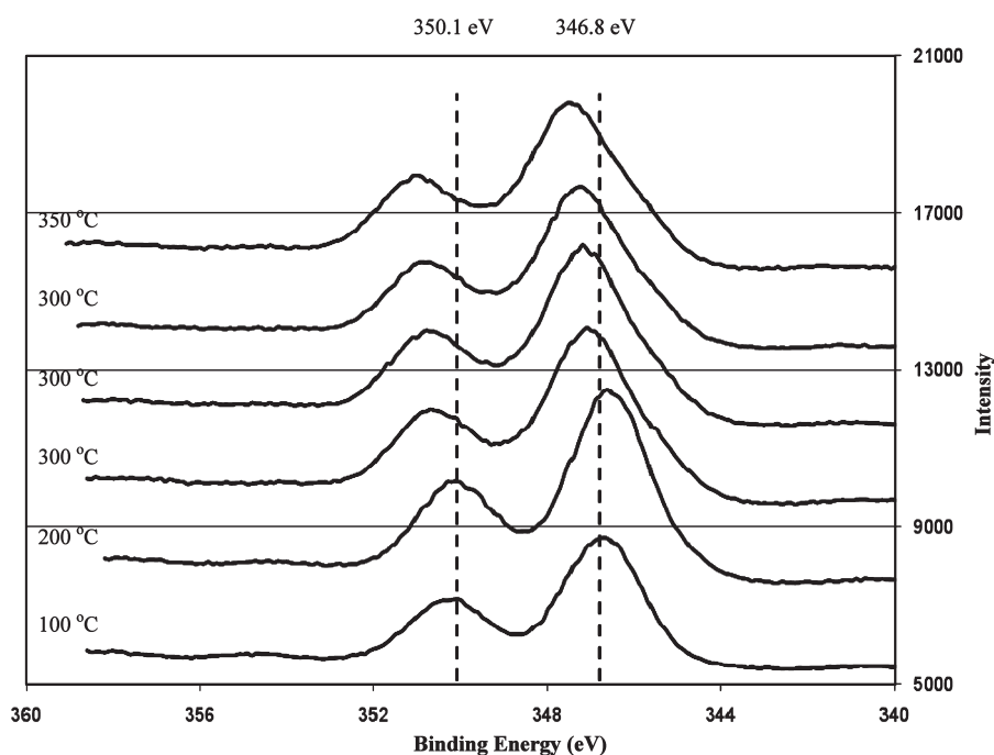
Figure 11. Ca 2p region of the \text{Na}_2\text{CO}_3/\text{CaO} (1:3) system during heating.
