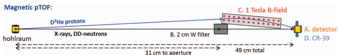
FIG. 2. A schematic of the MagPTOF diagnostic on the NIF. The diagnostic includes four main components: (A) CVD-diamond detector, (B) x-ray shielding (tungsten, configurable in units of 0.5 cm up to 4 cm) to shield the detector from hohlraum x-ray background, (C) a permanent dipole magnet with 1 T peak field to deflect protons around the shielding and onto the detector, and (D) optional annular piece of CR-39 around the CVD-diamond, to confirm proton fluence and energy on each shot. The MagPTOF detector, cables, and electronics are identical to the existing ones for the pTOF.
