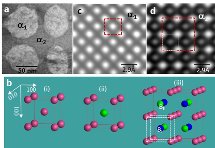
Figure 1 | (a) HAADF image of alnico alloy showing composite structure consisting of isolated Fe-Co-rich ( \alpha_1 ) phase (lighter contrast) embedded in continuous Al-Co-Ni-rich ( \alpha_2 ) phase; (b) models of three crystal structures: (i) BCC; (ii) B2 and (iii) L 21 ; and (c) and (d): high-resolution HAADF image of \alpha_1 and \alpha_2 phase, in [001] direction, respectively. In the model of the L 21 structure, there are two kinds of B sites, i.e. blue and green atoms, marked as B I and B II , respectively.
