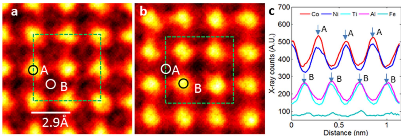
Figure 3 | (a) EDS map of combined Co K_{\alpha} and Ni K_{\alpha} ; (b) EDS map of combined Al K_{\alpha} , Ti K_{\alpha} and Fe K_{\alpha} ; and (c) line profiles of Co K_{\alpha} , Ni K_{\alpha} , Al K_{\alpha} , Ti K_{\alpha} and Fe K_{\alpha} along [100] direction. The maps are obtained from \alpha_2 phase in [001] direction. Line-profiles in (c) indicate Co and Ni atoms at A-sites and Al, Ti and Fe at B-sites, or B_I and B_{II} sites, which overlap in [001] direction. Lattice site positions (A, B) along [100] direction are marked by arrows in (c). Dashed squares in (a) and (b) mark size of L2_1 unit cell in [001] projection, and circles in (a) and (b) mark positions of A-sites and B-sites (or B_I and B_{II} sites, overlapped).
