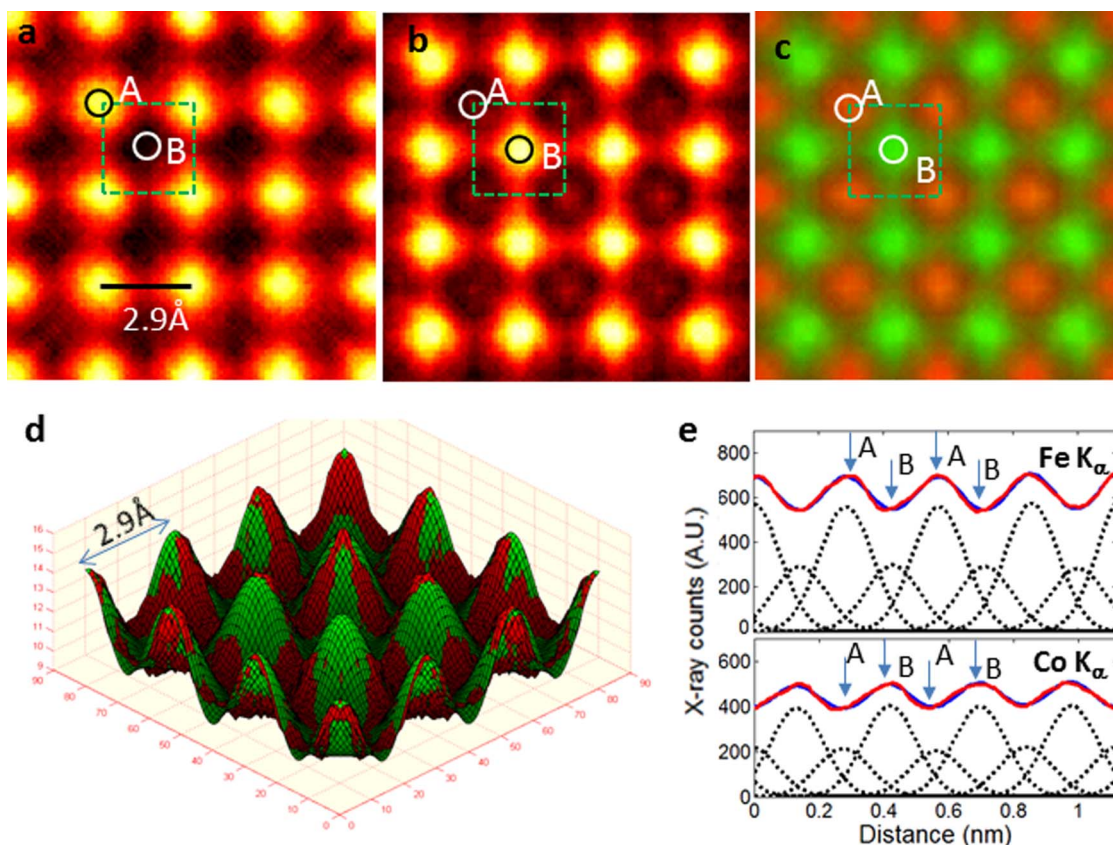
Figure 2 | (a) EDS map of Fe K_{\alpha} ; (b) EDS map of Co K_{\alpha} ; (c) composite color map of Fe K_{\alpha} (red) and Co K_{\alpha} (green); (d) surface-plot of experimental (red) and the least-square Gaussian-fitted (green) Fe K_{\alpha} map; and (e) line profiles of EDS X-ray counts for Fe K_{\alpha} and Co K_{\alpha} along [100] direction. Maps obtained from \alpha_1 phase in [001] direction. In (e), the solid blue line is the experimental data; the solid red line is from the least-square Gaussian-fitting; the individual Gaussian peaks at the lattice positions from the fitting are shown as dashed black lines; and arrows marked A and B indicate positions of A- and B- sites along [100] direction. Lattice site positions (A, B) and size of unit cell in [001] projection are also marked by circles and dashed square in EDS maps in (a), (b) and (c).
