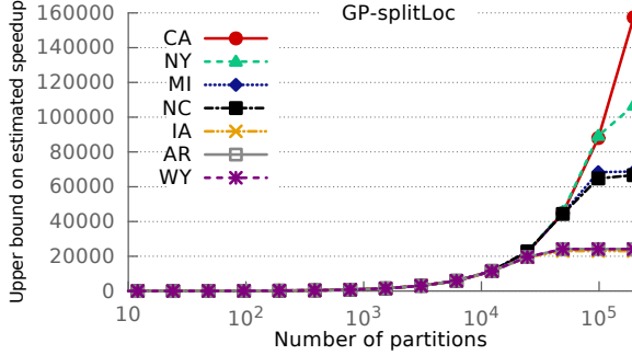
Figure 8. The estimated speedup evaluated identically as in Figure 4 after application-specific decomposition. (GP-splitLoc)
