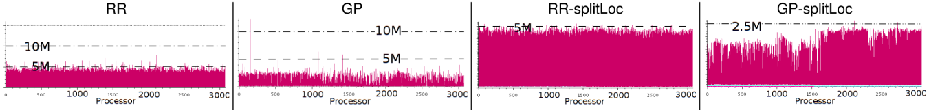
Figure 11. Amount of data received per PE in MB over six iterations using MI data and 4K core modules. GP has the highest maximum communication volume while GP-SPLITLOC has the lowest. Both have smaller average communication volume than RR and RR-SPLITLOC.
