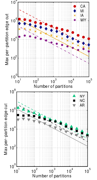
Figure 14. The maximum per-partition edge cut (GP-splitLoc).
