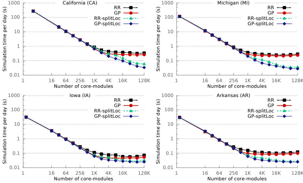
Figure 13. Strong scaling performance of EPISIMDEMICS for selected states on Blue Waters
