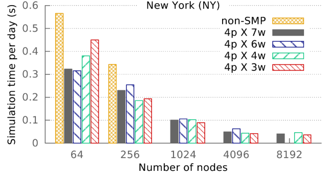
Figure 9. Identifying the best Charm++ SMP configuration on Blue Waters (RR-splitLoc). np \times mw denotes the case where there are n smp processes per compute node and m worker threads per process.
