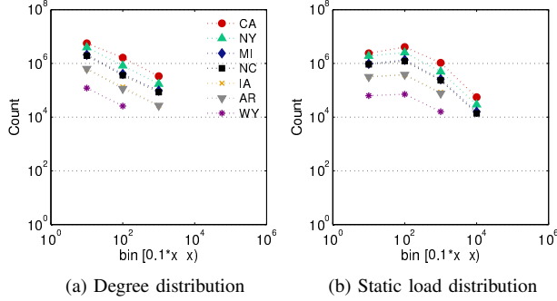
Figure 7. Degree distribution and load distribution after graph modification. (GP-splitLoc)
