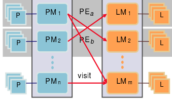
Figure 1. EPI-SIMDEMICs implemented in CHARM++
