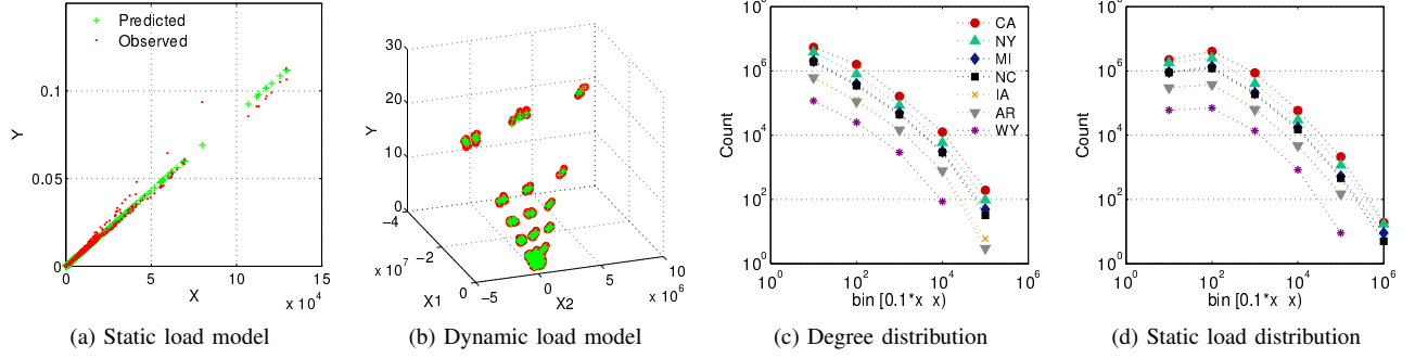
Figure 3. The load estimation model estimates the load of each location work unit on Blue Waters based on the node degree.
