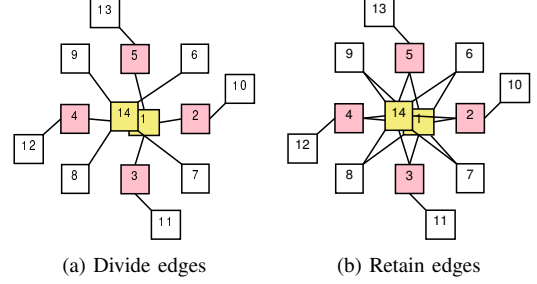
Figure 6. Two methods to split a heavily loaded node depending on available extra parallelism
