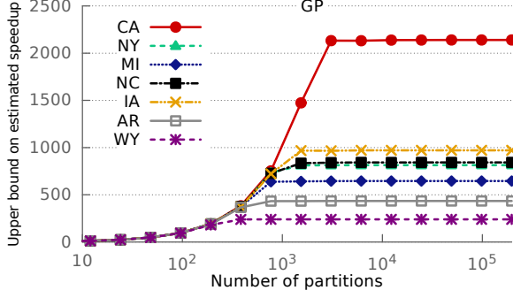
Figure 4. The estimated speedup for location computation based on the load distribution across data partitions. It is evaluated for each of seven states over various number of partitions between 12 and 196,608. (GP)
