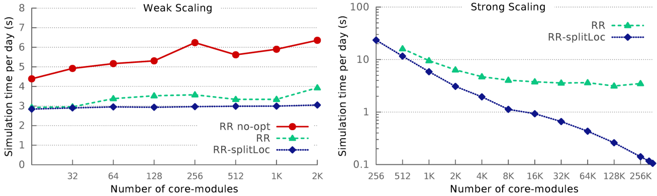
Figure 12. Weak and strong scaling performance of EPISIMDEMICS on Blue Waters. For weak scaling, we choose a subset of the continuous US by state such that the number of people per processor remains approximately constant. With the largest dataset fixed, we demonstrate weak scalability by using less than 1/4 of the available memory, which allows us to run up to 2k core modules. For strong scaling, we use data for the whole continental US.
