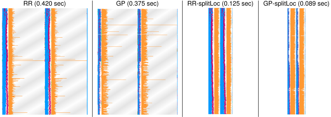
Figure 10. Timeline plots of two iterations of EPISIMDEMICS using MI data and 4K core modules on Blue Waters (sampled to show 384 compute PEs). The blue component shows the person computation, the red shows the receiver side message handling, and the orange shows the location computation. The time above the plot shows the average time taken over the two iterations while running the CHARM++ Projections visual analysis tool.
