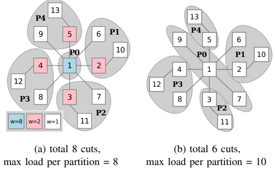
Figure 2. The optimal 5-way partitioning result for minimizing (a) load imbalance and (b) edge cut. Node 1 has weight 8, and Nodes 7 and 9 have weight 1 each.
