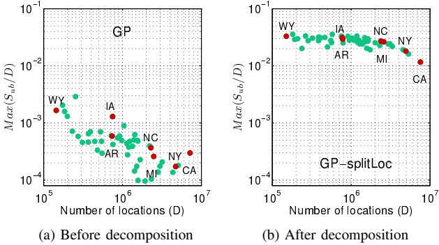
Figure 5. The maximum of the estimated speedup per location ( S_{ub}/D ) over the various number of partitions between 12 and 98304. Each dot represents one of 48 contiguous US states and DC.
