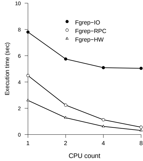
Figure 4.1: The execution time comparison with increasing CPU count for Fgrep-IO, Fgrep-RPC and Fgrep-HW (File size 8 GB).
