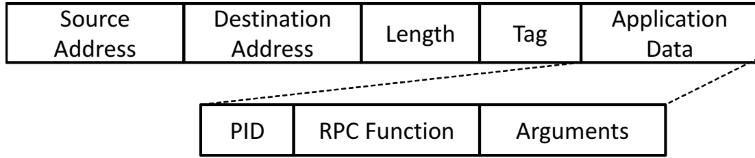
Figure 3.5: XSSD RPC packet structure to communicate with the SPU.
