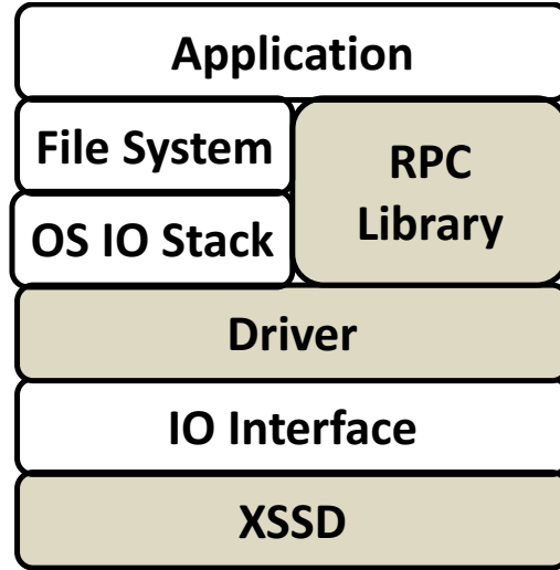
Figure 1.2: The system storage hierarchy for XSSD XSSD (gray boxes) extends the hardware and software to support application-specific processing close to the storage.
