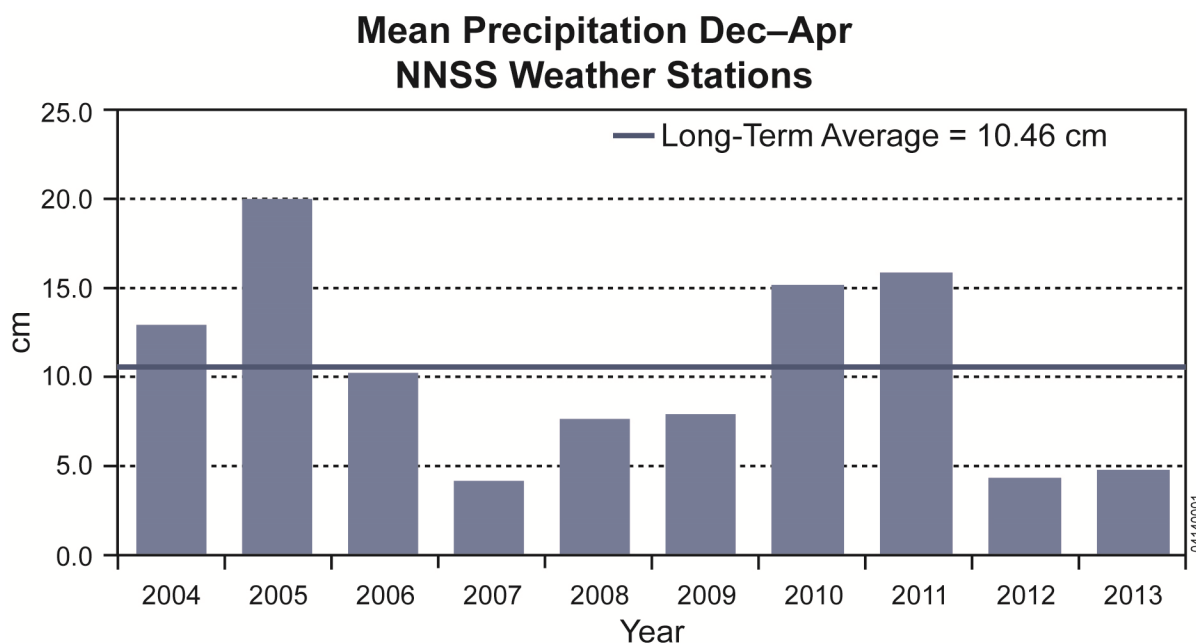
Figure 4-2. Average precipitation from December (previous year) through April for the years 2004 through 2013
