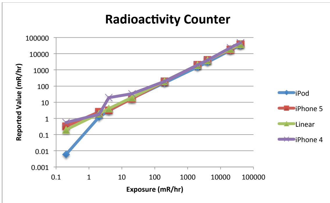
Figure 7: Radioactivity Counter performance plot
