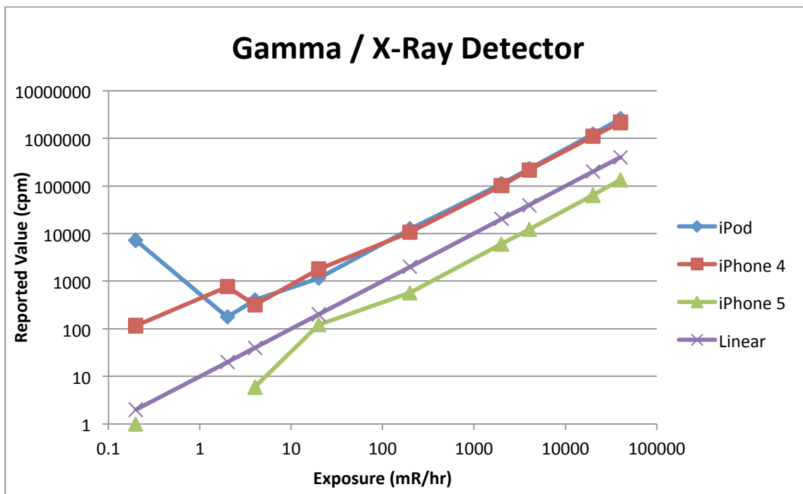
Figure 3: Gamma / X-Ray performance plot
