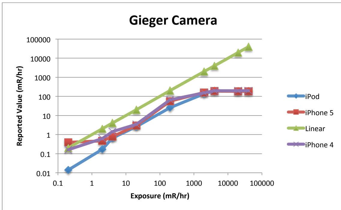
Figure 5: Geiger Camera performance plot
