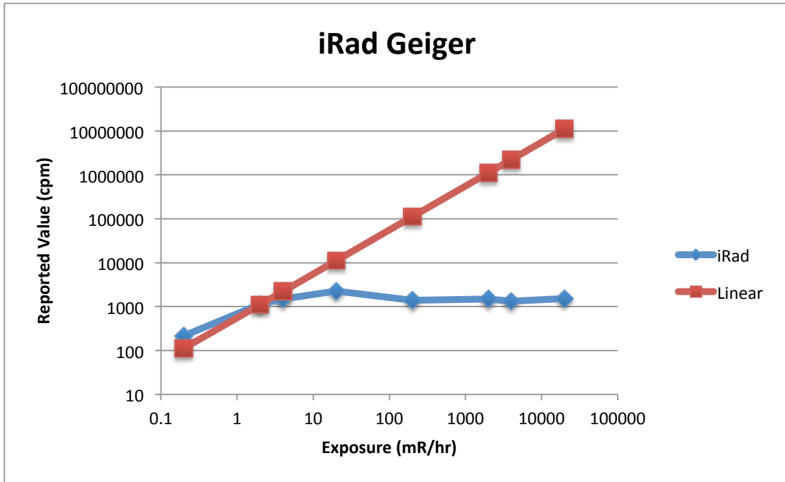
Figure 12: iRad Geiger Tube performance plot
