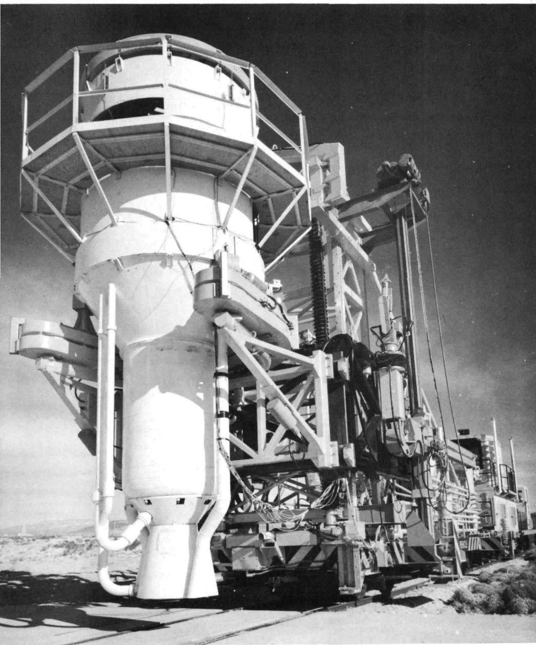
The Engine Installation Vehicle (EIV) carrying an engineering model of the NERVA engine. The shielded Manned Control Car (MCC), rear, propels the EIV along the NRDS railroad tracks.
