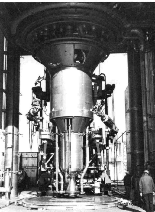
The Xe installed in ETS-1 in Nevada. The XE has been the engine closest to actual flight configuration.
