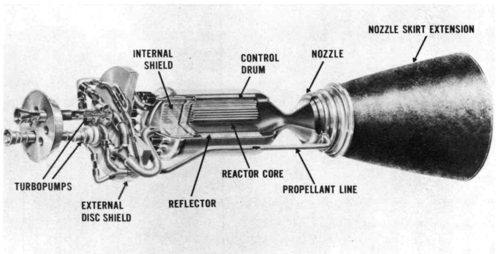
Drawing of the complete NERVA engine.
