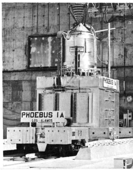
The Phoebus-1A reactor after arrival on its special railroad car at the test cell.
