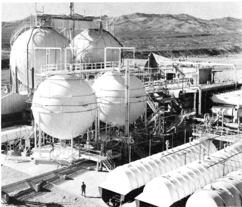
Giant dewars containing liquid hydrogen and liquid oxygen and a maze of pipes, valves, and other equipment are needed for the reactor tests. This is Test Cell C at NRDS.
