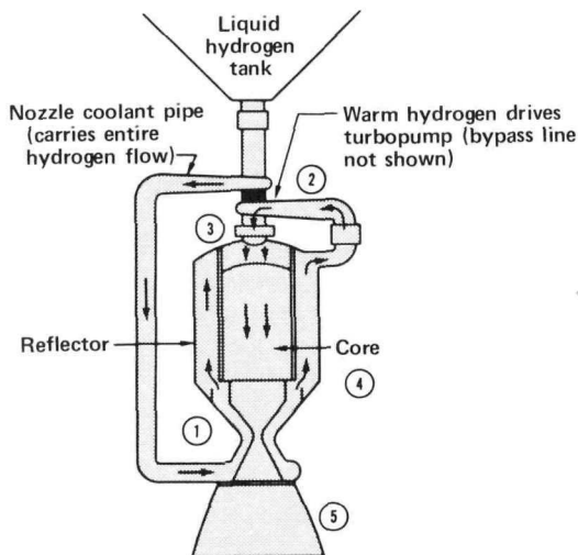
Hydrogen flow diagram in the full-flow cycle. The numbers refer to the description of the operation of this cycle on page 36.
