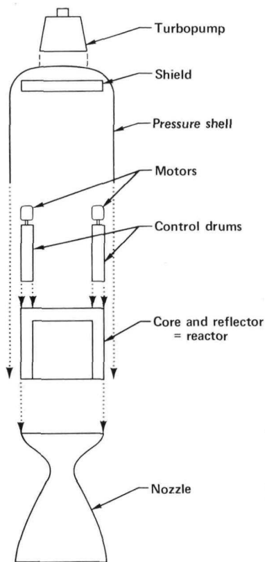
Exploded view of a nuclear rocket engine. Control drums fit in the reflector, the reactor inside the pressure shell, and the turbopump and nozzle go at top and bottom, respectively.
