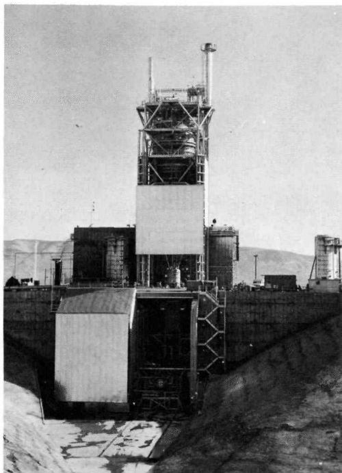
Engine Test Stand 1, from a different vantage that shows the exhaust deflector "canyon", foreground, incised in the desert floor to permit escape of burning hydrogen. Note upright semi-cylindrical shields on either side (near left, far right), which are moved around the engine while test is in progress.
