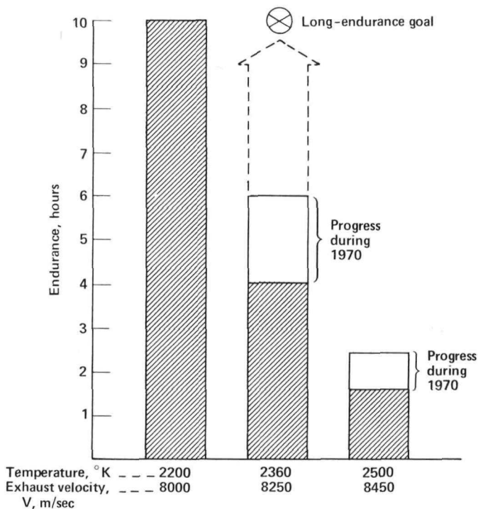
Lifetimes of NERVA fuel elements at different hydrogen temperatures.
