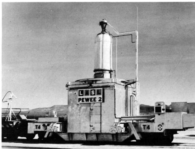
The Pewee-2 reactor on railroad car at NRDS in Nevada. Pewee-2 is a reactor in which fuel elements can be tested at conditions very close to (or even worse than) those encountered in an actual nuclear rocket engine.
