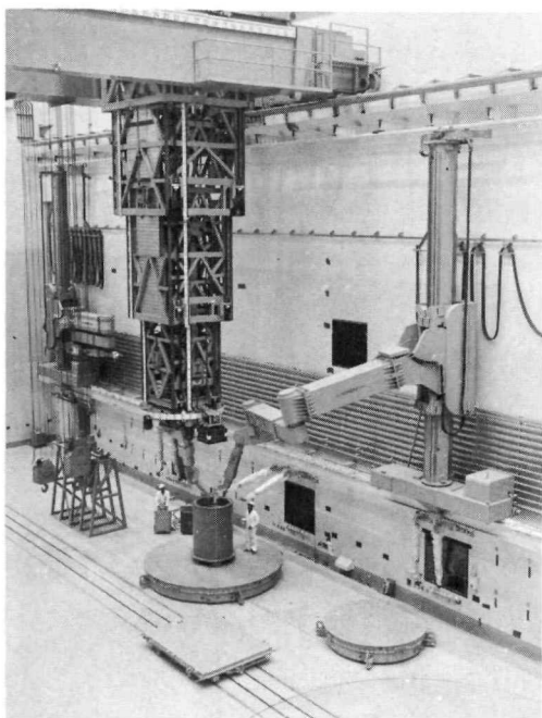
Interior of the E-MAD Building, showing the huge overhead and wall-mounted manipulators used for disassembling radioactive nuclear rocket engines. When in actual use, no workmen would be present in this portion of the building, because of the high radiation levels.
