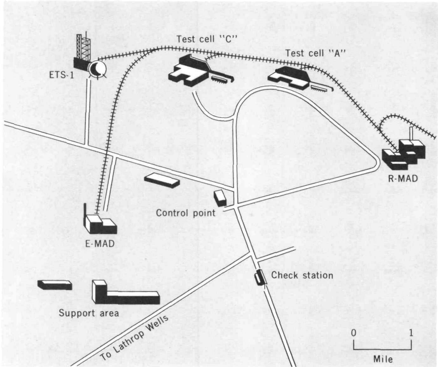
Arrangement of facilities at the Nuclear Rocket Development Station, Nevada.
