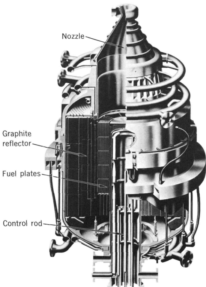
Cutaway drawing of a Kiwi-A reactor, showing the basic design of the graphite core.
