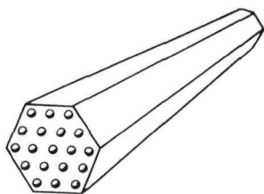
Sketch of a NERVA fuel element. The hexagon measures 0.75 inch (1.8 cm) across the flats (the sides of the element). Each hole is 0.1 inch (0.25 cm) in diameter.
