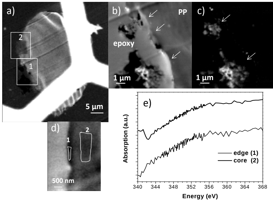
336 Fig. 9: (a) An OD image of a PP fiber from a crushed piece of composite paste where the 337 ROI indicates the areas where an image map and a Ca image stack were obtained; (b) an 338 OD image at Ca L edge, at a strong energy absorption (349.1 eV); (c) an image map 339 obtained from the same area as (b); and (d) an absorption image from the image stack from 340 ROI-2 where two absorption spectra were extracted and shown in (e).
