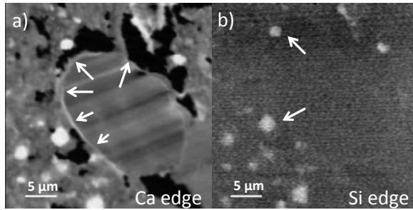
Fig. 5: Optical density (OD) images of a hybrid fiber in HCP embedded in epoxy (a) at Ca peak (at 349.1 eV), and (b) at Si peak, (at 1847.7 eV). The arrows on (a) indicate the sheath area around the fiber core containing traces of Ca, while on (b) they indicate the unhydrated cement particles rich in Si.
