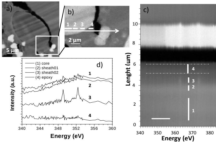
288 Fig. 6: (a) an OD image showing the area where a line scan at Ca L edge was performed; 289 (b) a zoomed in image showing the line scan position and the four regions where the 290 NEXAFS spectra were extracted; (c) a line scan image showing the four regions where the 291 spectra was extracted; and (d) the four extracted NEXAFS spectra.
