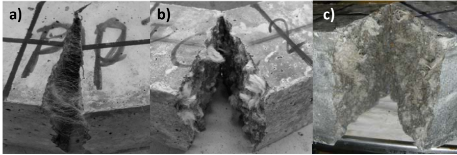
Fig. 15: Composite beams after completing the flexure tests: (a) PP fiber, (b) hybrid fiber, and (c) pre-dispersed hybrid fibers.
