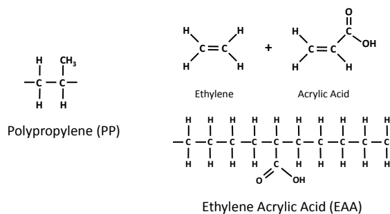
Fig. 1: Molecular structure of PP, EAA, and monomers ethylene and acrylic acid.
