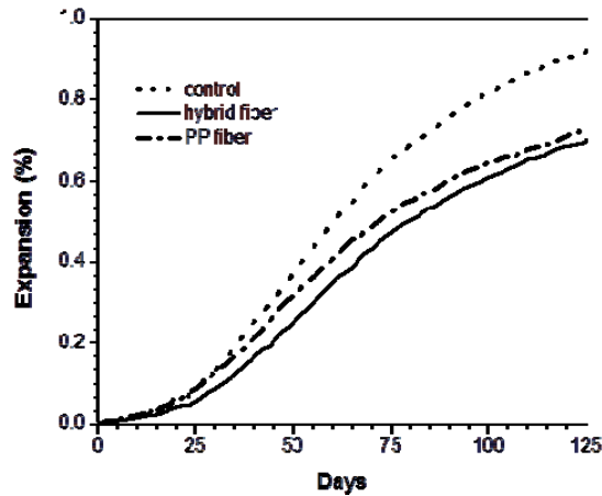
Fig. 11: Expansion of mortar bars due to ASR for three types of specimens: the control sample without fibers, the sample containing PP, and the sample containing hybrid fibers.
