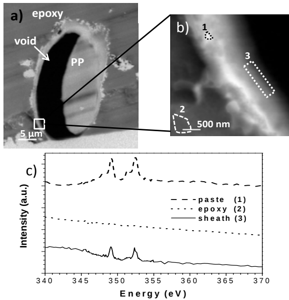
Fig. 8: (a) an OD image showing a hybrid fiber obtained from a crushed piece of composite paste where the ROI indicates the location from which a Ca L edge image stack was obtained; (b) the OD image extracted from the image stack (at 349.1 eV) showing the three areas where the NEXAFS spectra was extracted; and (c) NEXAFS spectra extracted for the three areas representing the Ca rich particle (1) from the HCP paste, the epoxy (2), and the EAA sheath (3).
