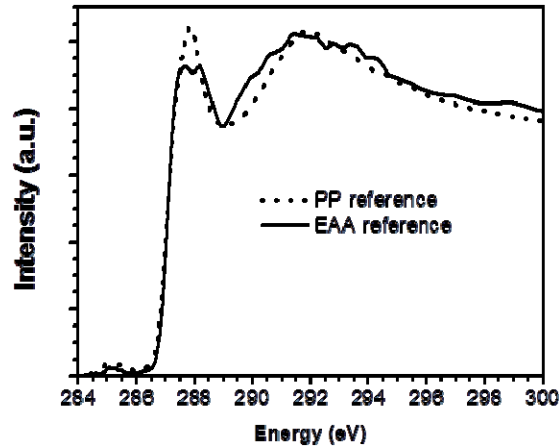
Fig. 2: C K-edge NEXAFS spectrum from the different polymer materials analyzed under STXM.
