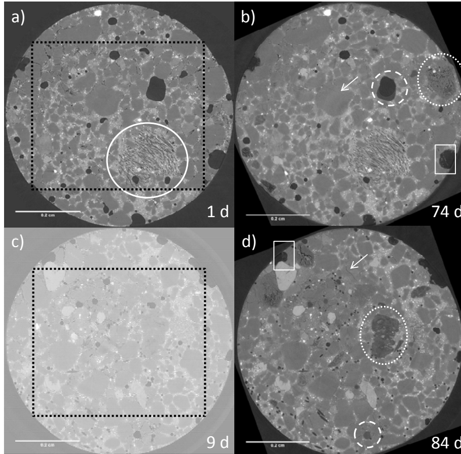
Fig. 12: Tomographic images taken from the PP and hybrid mortar composite cylinders after being immersed in 1M NaOH solution. Images (a) and (b) correspond to the hybrid fibers, while images (c) and (d) correspond to the PP cylinder. Scale bar represents 2mm.
