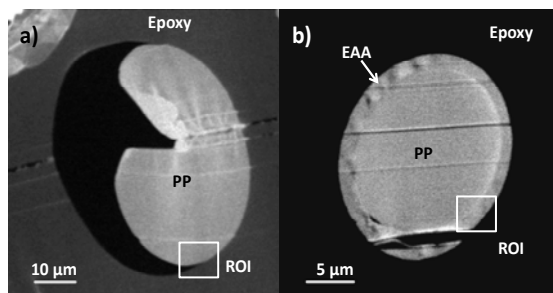
Fig. 3: STXM OD images of (a) the PP fiber taken at 287.7 eV and (b) the hybrid fiber taken at 288.2 eV.
