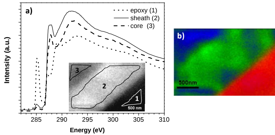
Fig. 4: (a) Spectrum of the three different components extracted C K-edge image stack from the ROI depicted in Fig. 3b (see inset): epoxy (dotted line), EAA sheath (solid line), and PP core (dashed line); and (b) the RGB composite image map showing the differentiation of the polymers, PP core (blue), EAA sheath (green), and epoxy (red).
