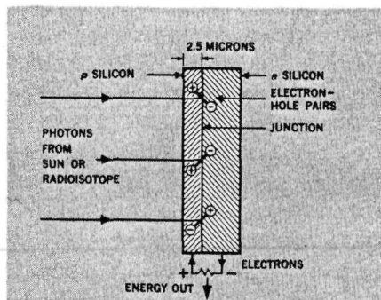
Figure 12 The photograph shows the solar cell in use on a satellite. The spherical, radioisotope, thermoelectric generator at the bottom of the satellite is used to supplement the solar cells. In the solar cell, hole-electron pairs are created by solar photons in the vicinity of a p-n junction. Courtesy U. S. Air Force and National Aeronautics and Space Administration.
