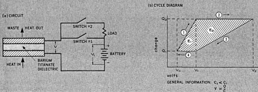
Figure 14 The ferroelectric converter is really an electrical capacitor whose capacitance is changed by temperature. When heat is added, capacitance drops, voltage rises, and the capacitor is made to discharge through the load. CYCLE: ① Switch #1 closed, #2 open. Condenser charges from battery to charge Q_2 at voltage V_1 with capacity C_1 . ② All switches open. Heat added, capacity changes from C_1 to C_2 , charge remains constant, so voltage changes from V_1 to V_2 . ③ Switch #2 closed, #1 open. Condenser discharges through load and battery to charge Q_1 at voltage V_1 with capacity C_2 . ④ All switches open. Heat rejected, capacity changes from C_2 to C_1 , charge remains constant, so voltage changes from V_1 to V_0 . CYCLE THEN REPEATS. Energy supplied from battery each cycle is E_1 . Energy delivered to load and battery each cycle is E_2 . Net energy converted is then E_2 - E_1 , the difference in the shaded areas.
