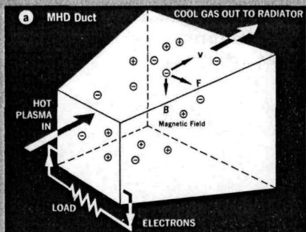
Figure 9 In the MHD duct (a), the electrons in the hot plasma move to the right under influence of force F in the magnetic field B . The electrons collected by the right-hand side of the duct are carried to the load. In a wire in the armature of a conventional generator (b) the electrons are forced to the right by the magnetic field.
