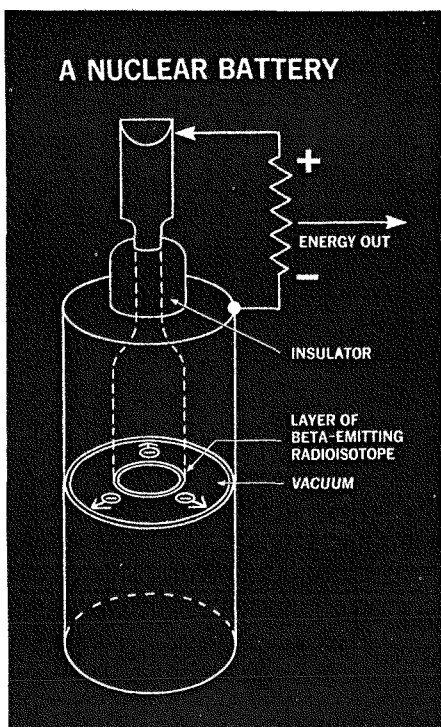
Figure 13 The nuclear battery depends upon the emission of charged particles from a surface coated with a radioisotope. The particles are collected on another surface.
