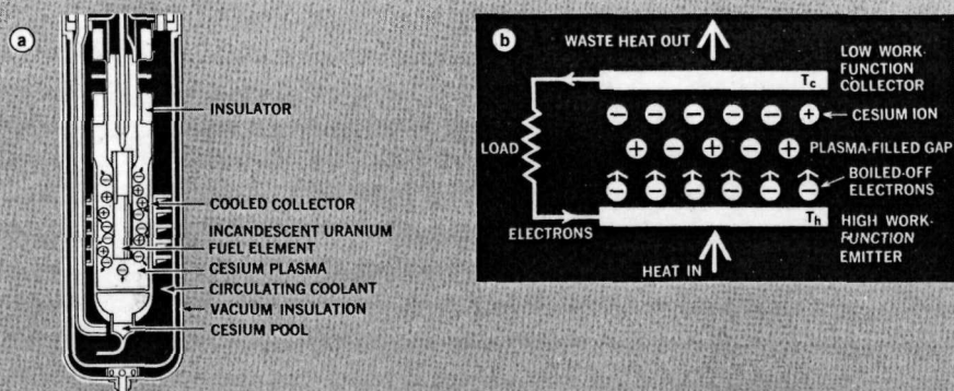
Figure 8 Thermionic converters may be flat-plate types or cylindrical types. The cylindrical converter (a) is an experimental type for ultimate use in nuclear reactors.
