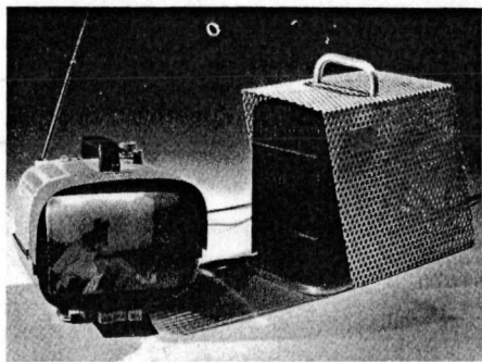
Figure 6 Commercially available thermoelectric generators using propane fuel can provide more than enough electrical power to operate a portable TV set. Courtesy Minnesota Mining & Manufacturing Company.
