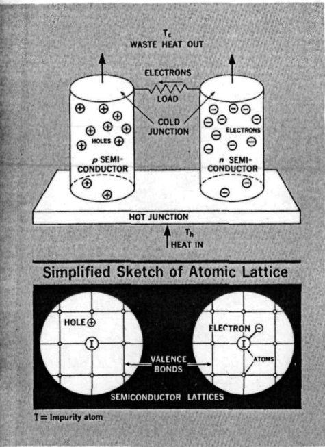
Figure 5 Top: thermoelectric couple made from p- and n-type semiconductors. Bottom: the impurity atoms (I) are different in each leg and contribute an excess or deficiency of valence electrons. Heat drives both holes and electrons toward the cold junction.
