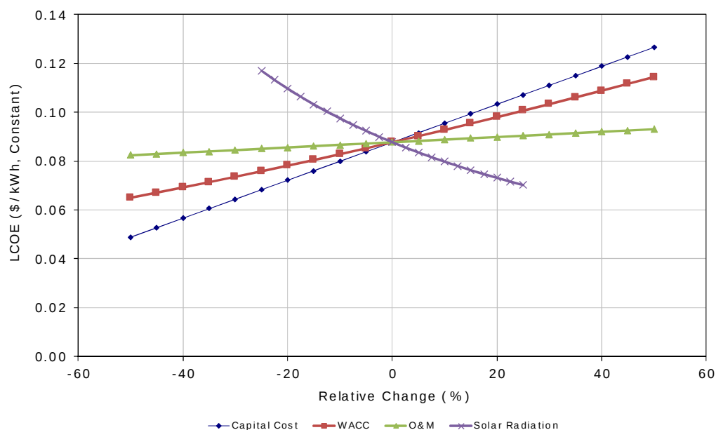
Exhibit 2. LCOE Sensitivity Analysis for Option 4B (Lone Butte Substation, 1-X tracking)
