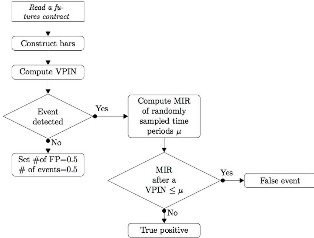
Figure 3 Flowchart of how a VPIN event is classified (Wu, Bethel, Gu, Leinweber, Rüebel 2013)
