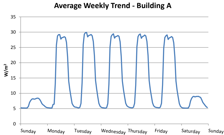
Figure 8: Building A average weekly energy consumption trend
