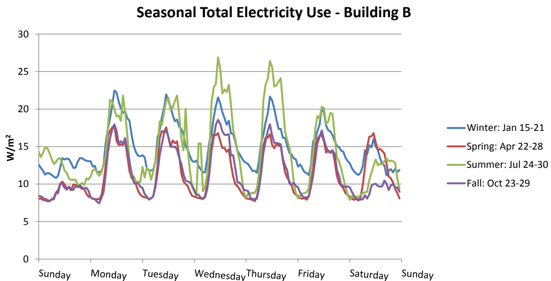
Figure 20: Building B seasonal differences in energy consumption
