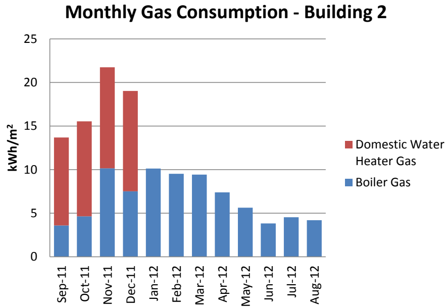
Figure 48 Building 2 monthly gas consumption
