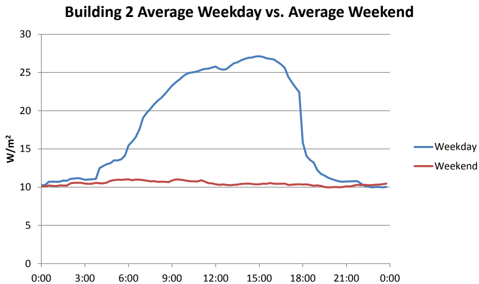
Figure 46 Building 2 average weekday versus weekend total energy consumption
