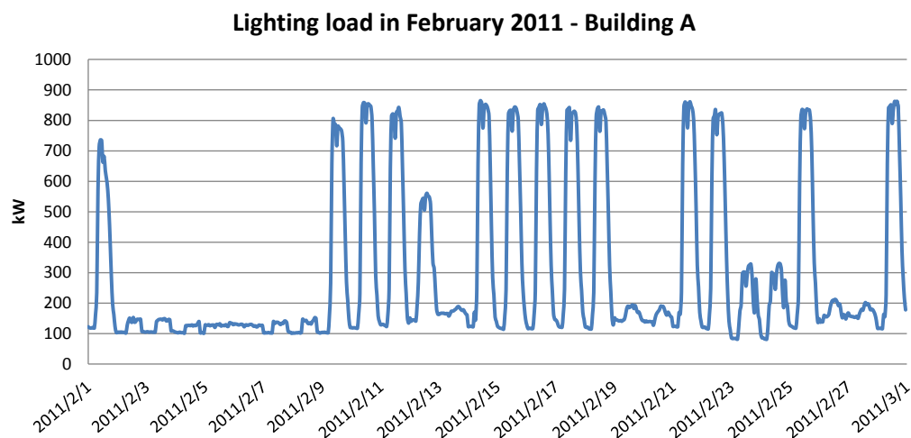
Figure 6: Building A's lighting load in February 2011
