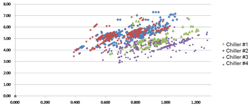
Figure 13: Scatter plot of chiller COPs
