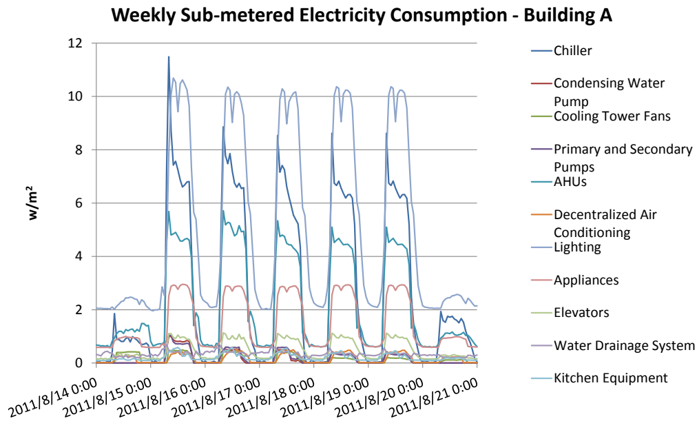
Figure 7: Building A weekly sub-metered energy consumption
