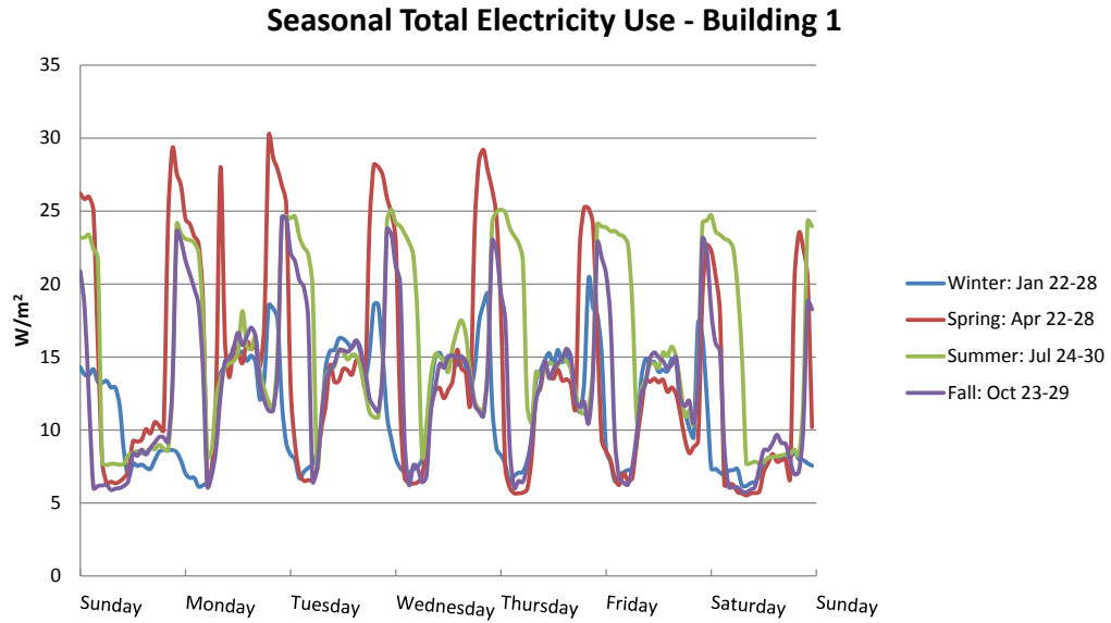
Figure 29: Building 1 seasonal differences in energy consumption
