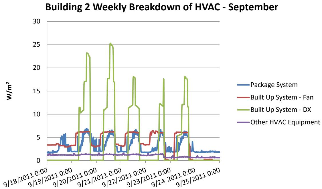
Figure 39 Building 2 weekly breakdown of HVAC in September
