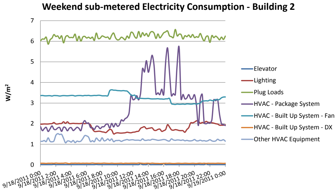
Figure 45 Building 2 typical weekend electricity consumption trend
