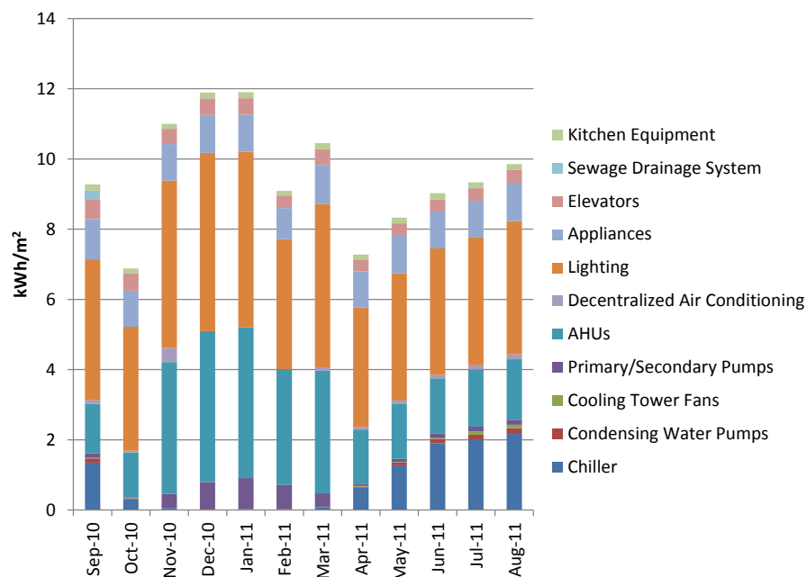
Figure 5: Building A monthly electricity breakdown from September 2010-August 2011
