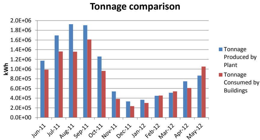
Figure 23: Tonnage comparison between chilled water produced by the plant chiller and chilled water consumed by all buildings on campus
