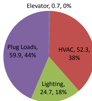
Annual Breakdown of Total Electricity Consumption - Building 2 kWh/m 2
