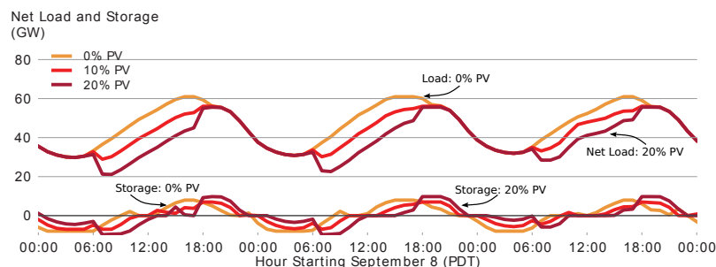
Figure 15: Net load (load less PV) and storage generation on peak days with increasing PV penetration.
