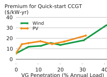
Figure 26: Change in the short-run profit premium for a quick-start CCGT relative to a CCGT without quick start.
