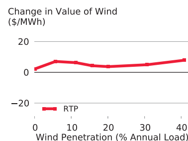
Figure 16: Change in the marginal economic value of wind with RTP and price-responsive demand relative to Reference scenario.
