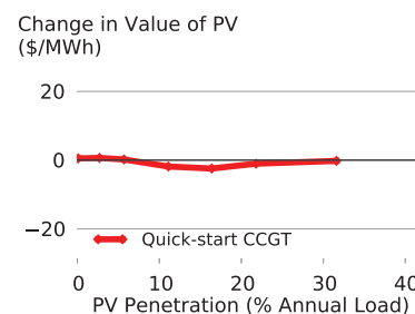
Figure 12: Change in the marginal economic value of PV with all new CCGTs having quick-start capabilities relative to the Reference scenario.
