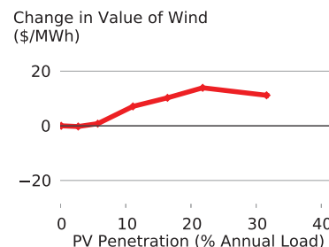
Figure 21: Change in the marginal economic value of wind at 0% penetration with increasing penetration of PV.
