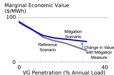
Figure 2: As shown here, change in the value of VG after implementation of a mitigation measure is defined in relation to the value in the Reference scenario from the valuation report.
