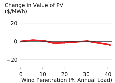
Figure 23: Change in the marginal economic value of PV at 0% penetration with increasing penetration of wind.
