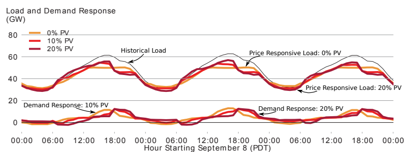
Figure 18: Historical load (thin line), price-responsive load, and effective demand response on peak days with increasing PV penetration.
