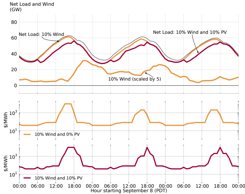
Figure 8: Historical load (thin line), net load, wind generation profile (scaled by a factor of 5 for clarity), and resulting RT price on three peak load days with and without 10% PV penetration.
