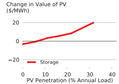
Figure 14: Change in the marginal economic value of PV with low-cost PHS relative to the Reference scenario.
