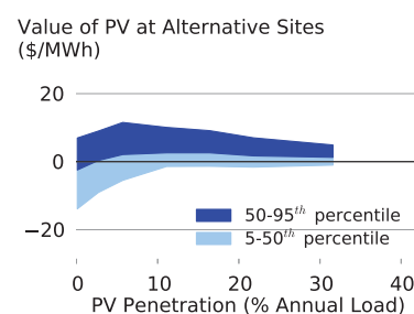
Figure 20: Difference between the marginal value of PV at alternative PV sites relative to the value of PV at sites used in the Reference scenario.
