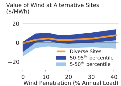
Figure 19: Difference between the marginal value of wind at alternative wind sites relative to the value of wind at sites used in the Reference scenario.
