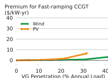
Figure 25: Change in the short-run profit premium for a fast-ramping CCGT relative to a CCGT without fast ramping.
