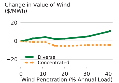
Figure 5: Change in the marginal economic value of wind with geographically concentrated or diverse wind sites relative to the Reference scenario.
