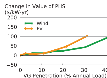
Figure 27: Change in the short-run profit of PHS with increasing VG.
