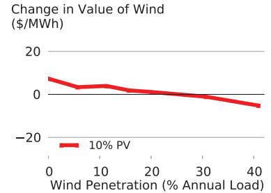
Figure 7: Change in the marginal economic value of wind with 10% penetration of PV relative to the Reference scenario.
