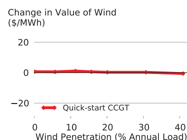
Figure 11: Change in the marginal economic value of wind with all new CCGTs having quick-start capabilities relative to the Reference scenario.
