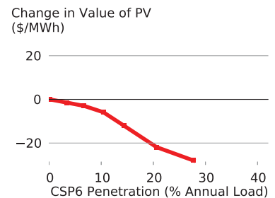
Figure 24: Change in the marginal economic value of PV at 0% penetration with increasing penetration of CSP with 6 hours of thermal storage.
