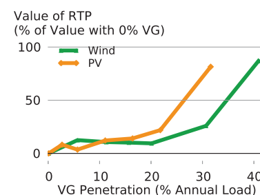
Figure 28: Change in the benefit of RTP with increasing VG as a percentage of the benefit of RTP at 0% VG.
