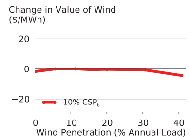
Figure 9: Change in the marginal economic value of wind with 10% penetration of CSP with 6 hours of thermal energy storage relative to the Reference scenario.
