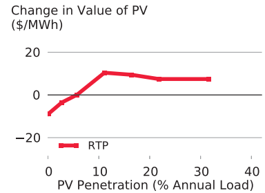
Figure 17: Change in the marginal economic value of PV with RTP and price-responsive demand relative to the Reference scenario.
