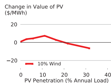
Figure 10: Change in the marginal economic value of PV with 10% penetration of wind relative to the Reference scenario.
