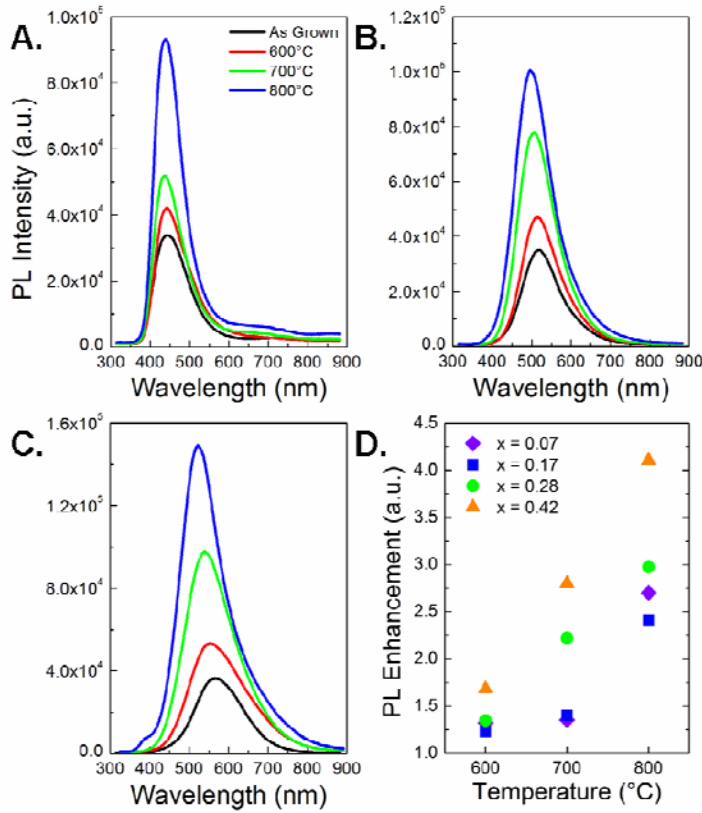
Figure 5. PL spectra of as grown and annealed In x Ga 1-x N samples (A) x = 0.17 , (B) x = 0.28 , and (C) x = 0.42 excited using a 325 nm HeCd laser. All compositions show an enhancement in emission with annealing temperature. The peak wavelength blueshifts because of a reduction in band gap from the removal of indium. Additional peaks are formed for sample (C) x = 0.42 from phase separation. (D) Integrated PL intensities show greater enhancements in QE for higher indium composition nanowire arrays.
