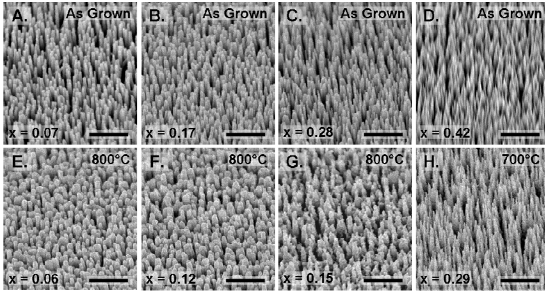
Figure 1. SEM images of as grown and annealed \text{In}_x\text{Ga}_{1-x}\text{N} nanowires. Tilted ( 45^\circ ) SEM images of as grown (A-D) and annealed (E-H) \text{In}_x\text{Ga}_{1-x}\text{N} nanowires on \text{Al}_2\text{O}_3(001) , demonstrating that samples retain the nanowire morphology after annealing. The image for each annealed nanowire array corresponds to the as grown sample directly above it. Compositions measured by SEM EDS show that the total indium content decreases after annealing (E-H), indicating that indium is preferentially etching from the lattice. Scale bar = 500 nm.
