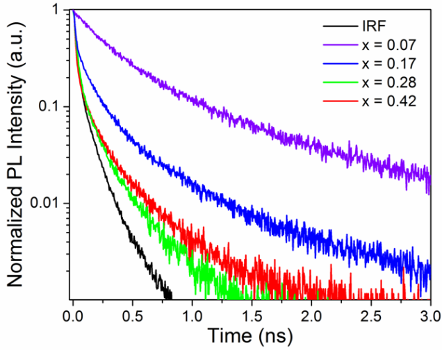
Figure 6. Time-resolved PL spectra of as grown \text{In}_x\text{Ga}_{1-x}\text{N} nanowires. Time-resolved PL spectra from samples excited using a 267 nm fs pulsed laser show a decrease in PL lifetime with increasing indium composition. The fast initial decay of samples x = 0.28 and 0.42 are limited by the instrument response function (IRF) plotted in black.
