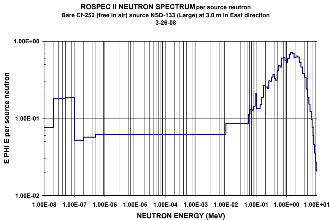
Figure C-19. Neutron spectra from bare ^{252}\text{Cf} (free in air) source NSD-133 (Large) at 3.0 m in East direction
