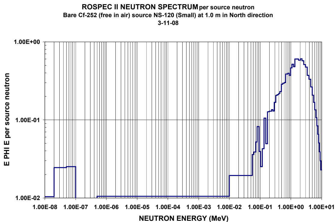
Figure C-1. Neutron spectra from bare ^{252}\text{Cf} (free in air) source NS-120 (Small) at 1.0 m in North direction
