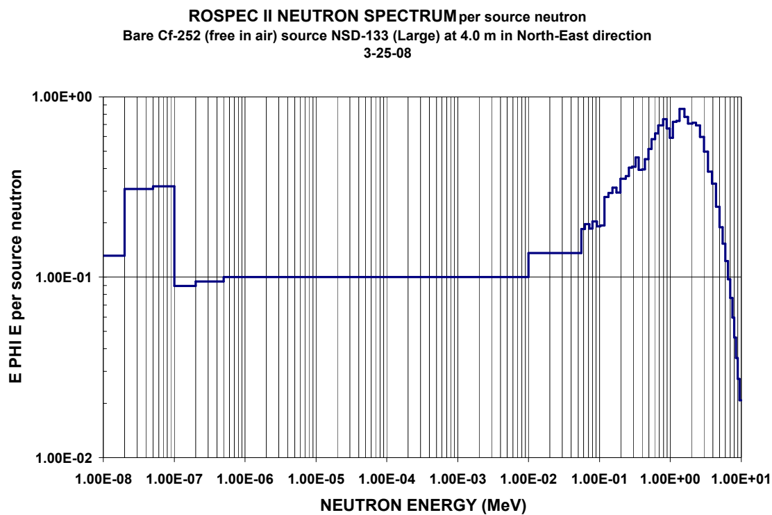
Figure C-27. Neutron spectra from bare ^{252}\text{Cf} (free in air) source NSD-133 (Large) at 4.0 m in North-East direction
