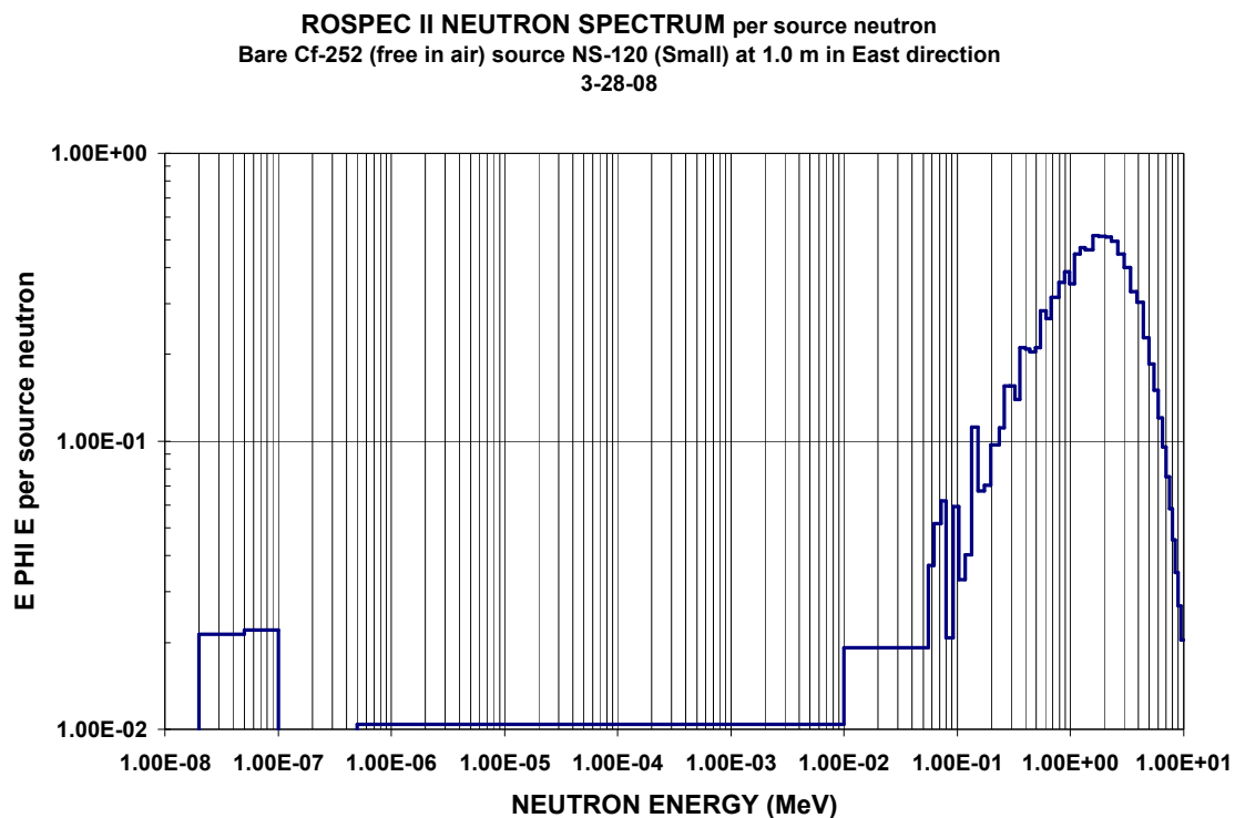
Figure C-2. Neutron spectra from bare ^{252}\text{Cf} (free in air) source NS-120 (Small) at 1.0 m in East direction
