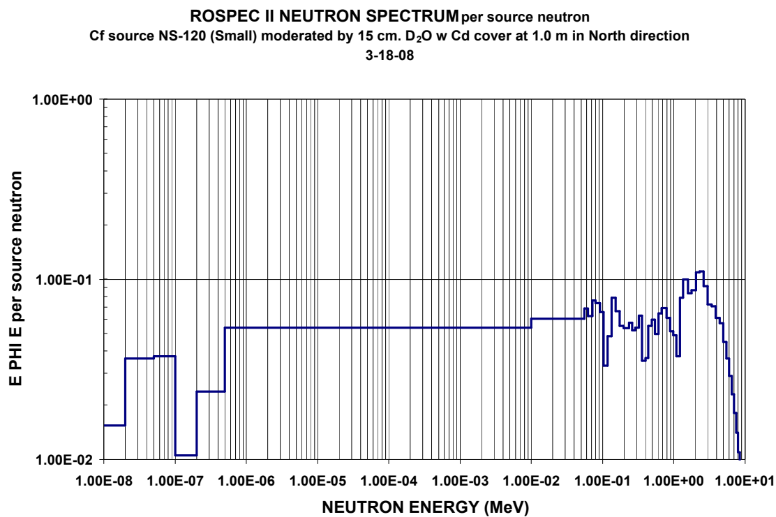
Figure C-3. Neutron spectra from ^{252}\text{Cf} source NS-120 (Small) moderated by 15 cm. \text{D}_2\text{O} w Cd cover at 1.0 m in North direction
