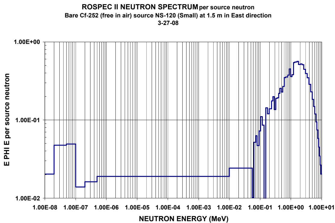
Figure C-6. Neutron spectra from bare ^{252}\text{Cf} (free in air) source NS-120 (Small) at 1.5 m in East direction
