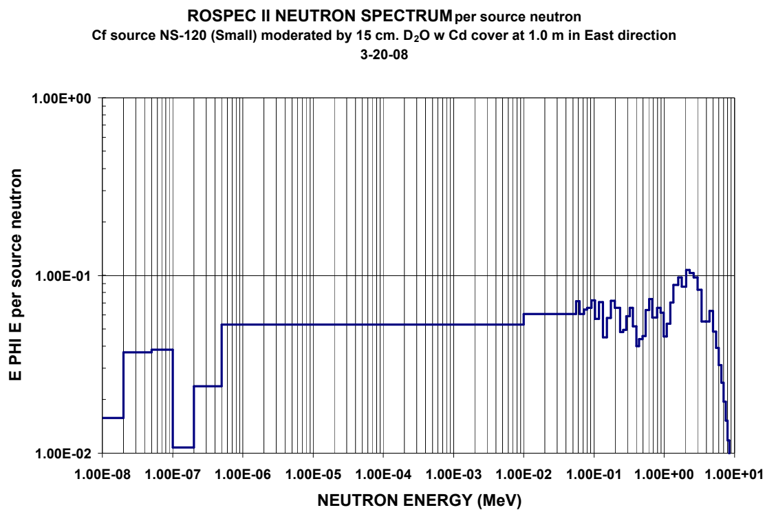
Figure C-4. Neutron spectra from ^{252}\text{Cf} source NS-120 (Small) moderated by 15 cm. \text{D}_2\text{O} w Cd cover at 1.0 m in East direction
