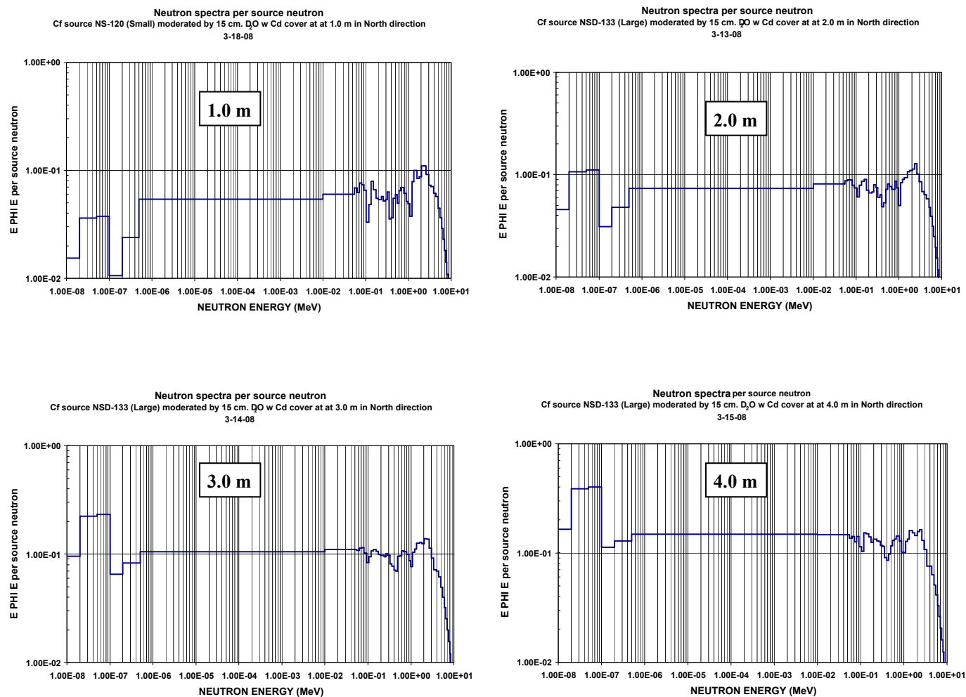
Figure 14. Neutron spectra at different distances (1.0 – 4.0 meters) from a D 2 O moderated 252 Cf source in North direction
