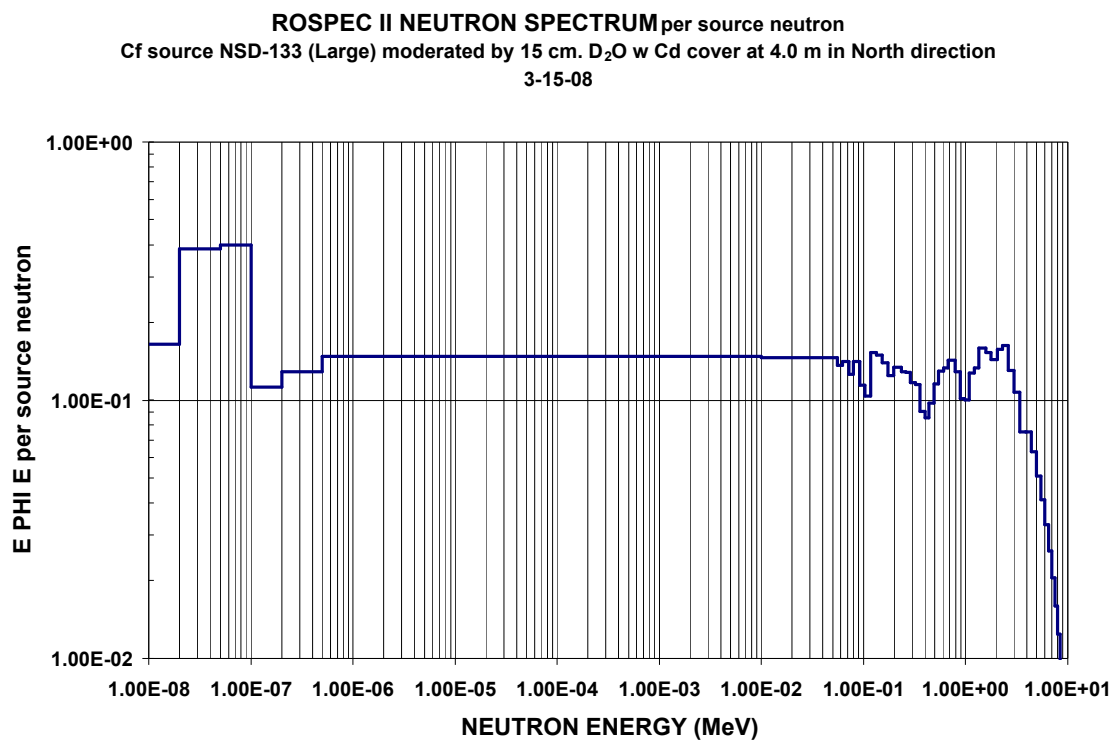
Figure C-28. Neutron spectra from ^{252}\text{Cf} source NSD-133 (Large) moderated by 15 cm. \text{D}_2\text{O} w Cd cover at 4.0 m in North direction
