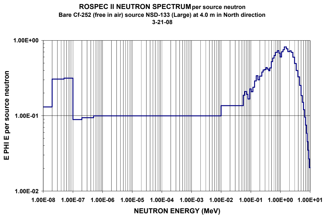
Figure C-26. Neutron spectra from bare ^{252}\text{Cf} (free in air) source NSD-133 (Large) at 4.0 m in North direction
