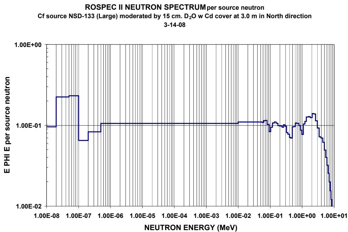
Figure C-21. Neutron spectra from ^{252}\text{Cf} source NSD-133 (Large) moderated by 15 cm. \text{D}_2\text{O} w Cd cover at 3.0 m in North direction
