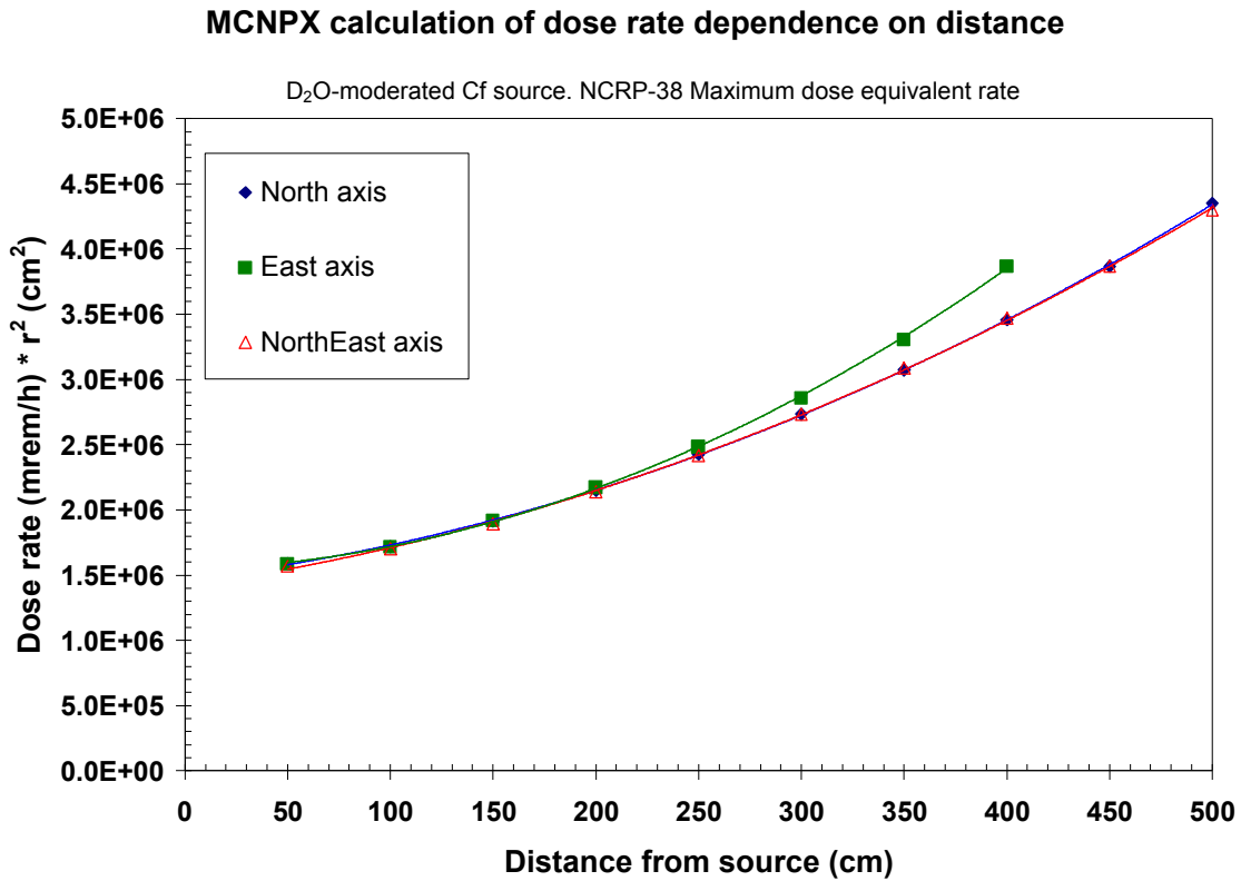
Figure 19. MCNPX calculated dose rate dependence on distance for D 2 O moderated 252 Cf
