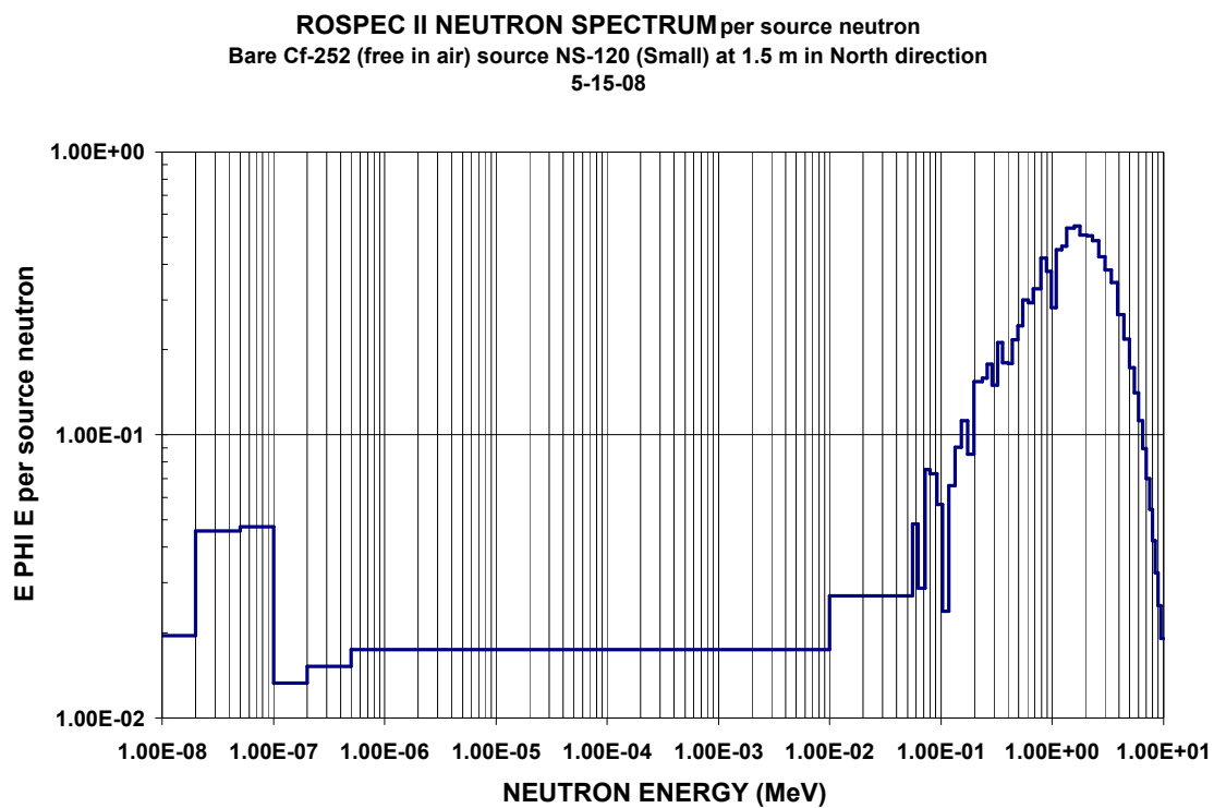
Figure C-5. Neutron spectra from bare ^{252}\text{Cf} (free in air) source NS-120 (Small) at 1.5 m in North direction
