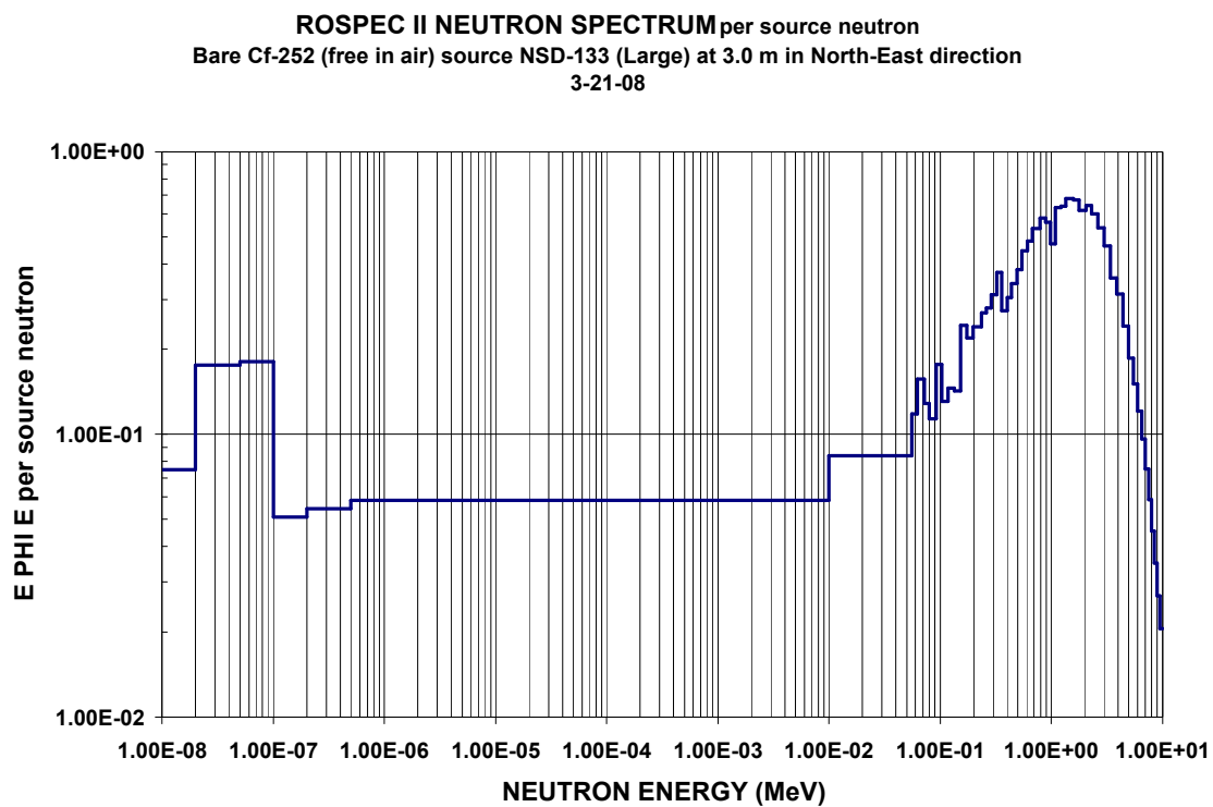
Figure C-20. Neutron spectra from bare ^{252}\text{Cf} (free in air) source NSD-133 (Large) at 3.0 m, in North-East direction
