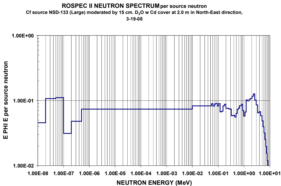
Figure C-13. Neutron spectra from ^{252}\text{Cf} source NSD-133 (Large) moderated by 15 cm. \text{D}_2\text{O} w Cd cover at 2.0 m in North-East direction
