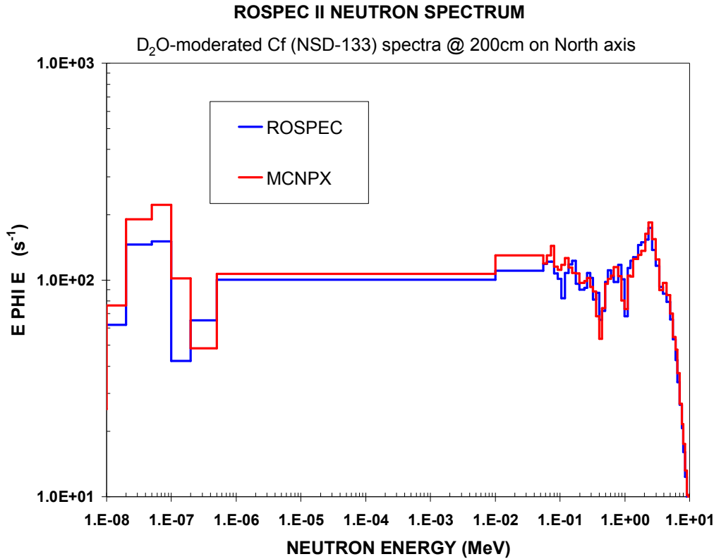
Figure 11. Absolute comparison of ROSPEC and MCNPX spectra for D 2 O moderated 252 Cf
