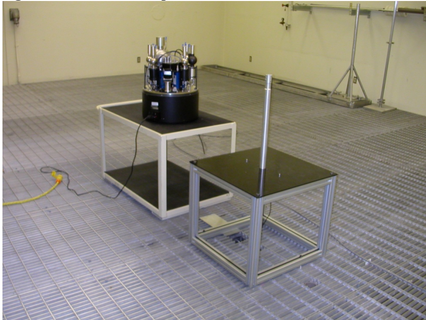
Figure 7. Neutron spectra and dose rates measurement from bare ^{252}\text{Cf} source
