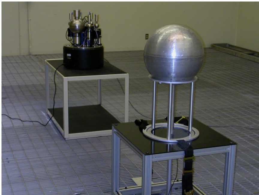
Figure 8. Neutron spectra and dose rates measurements from a \text{D}_2\text{O} moderated ^{252}\text{Cf} source
