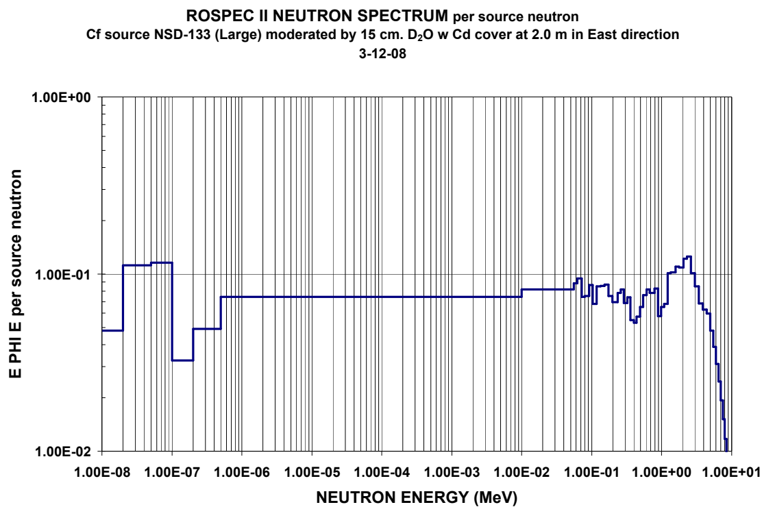
Figure C-12. Neutron spectra from ^{252}\text{Cf} source NSD-133 (Large) moderated by 15 cm. \text{D}_2\text{O} w Cd cover at 2.0 m, in East direction
