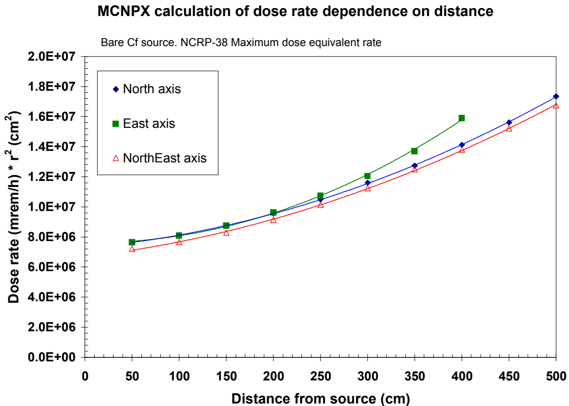
Figure 18. MCNPX calculated dose rate dependence on distance for bare ^{252}\text{Cf}
