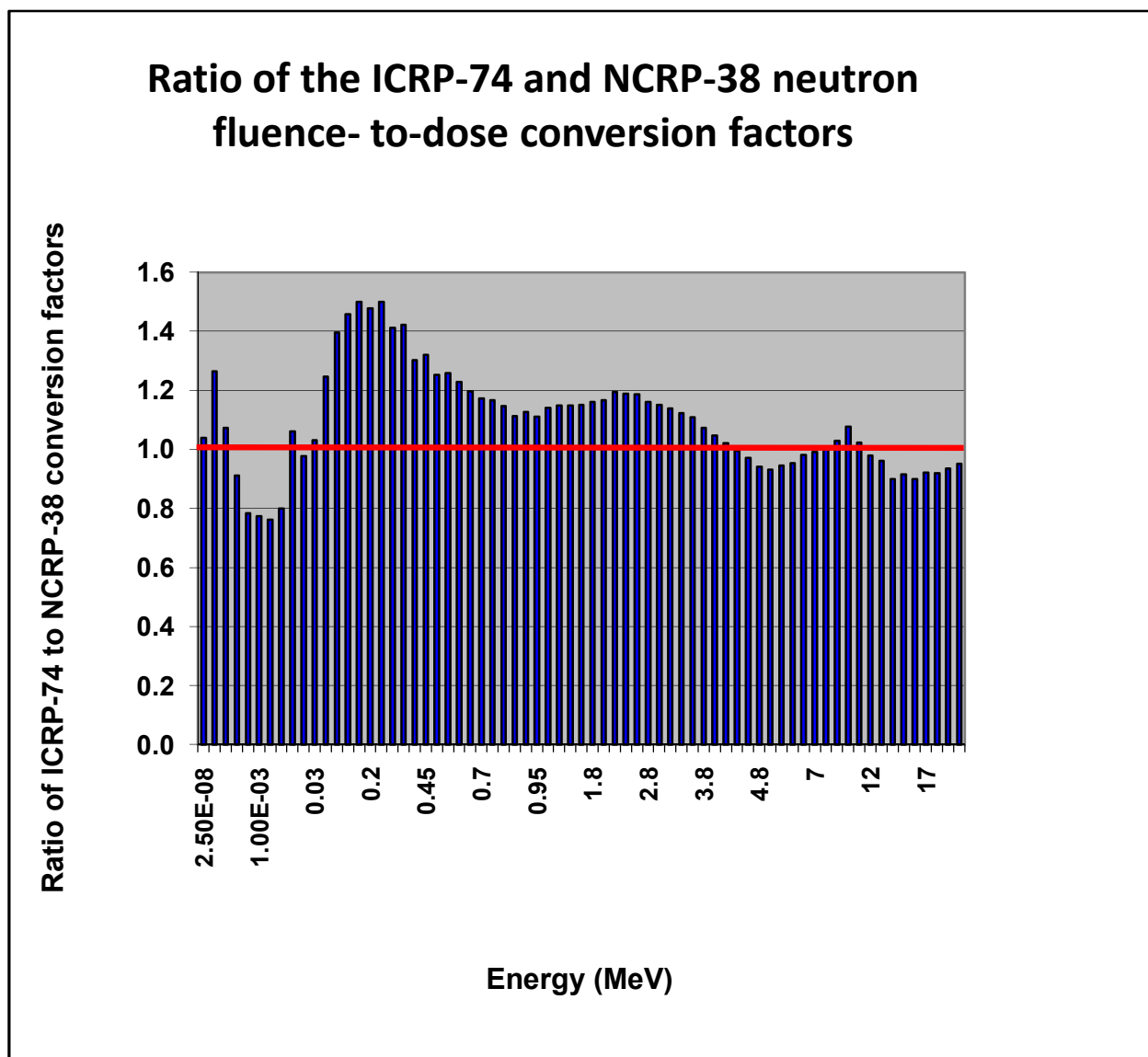
Figure 22. Ratio of the ICRP-74 and NCRP-38 neutron fluence-to-dose conversion factors
