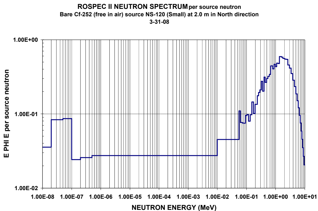
Figure C-8. Neutron spectra from bare ^{252}\text{Cf} (free in air) source NS-120 (Small) at 2.0 m in North direction
