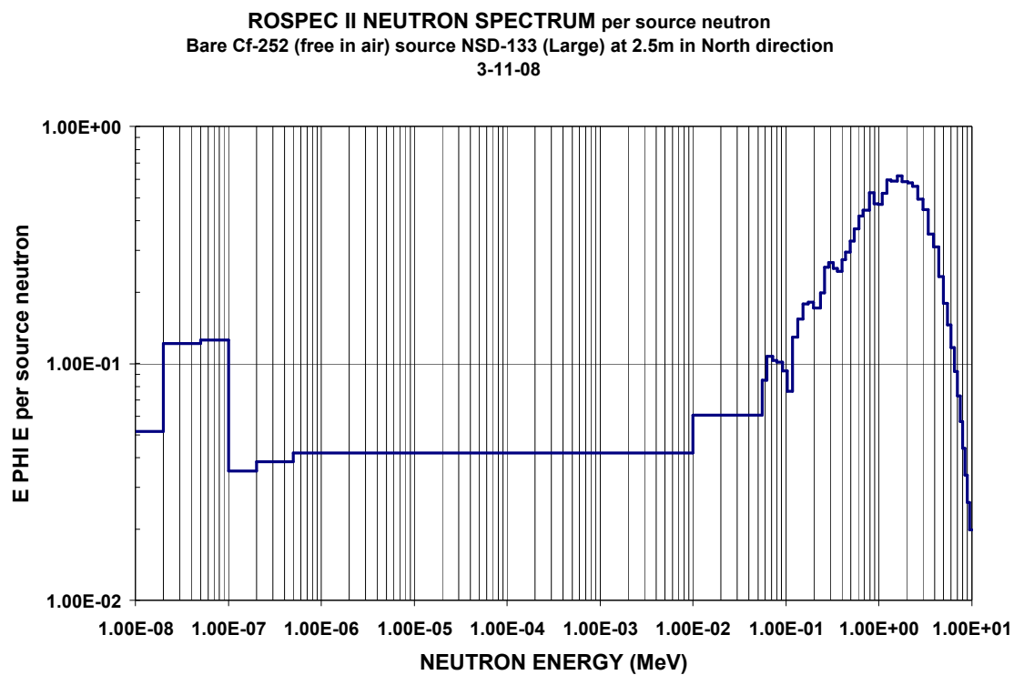
Figure C-14. Neutron spectra from bare ^{252}\text{Cf} (free in air) source NSD-133 (Large) at 2.5m in North direction
