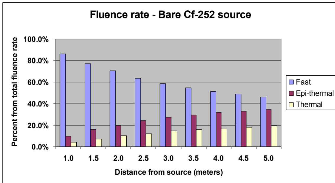
Figure 15. Contribution of different neutron energies to the total fluence at various distances from the ^{252}\text{Cf} source measured by ROSPEC
