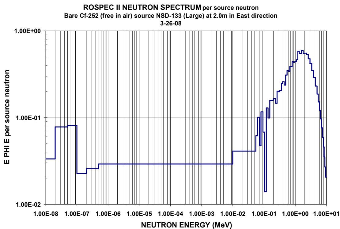
Figure C-10. Neutron spectra from bare ^{252}\text{Cf} (free in air) source NSD-133 (Large) at 2.0m in East direction
