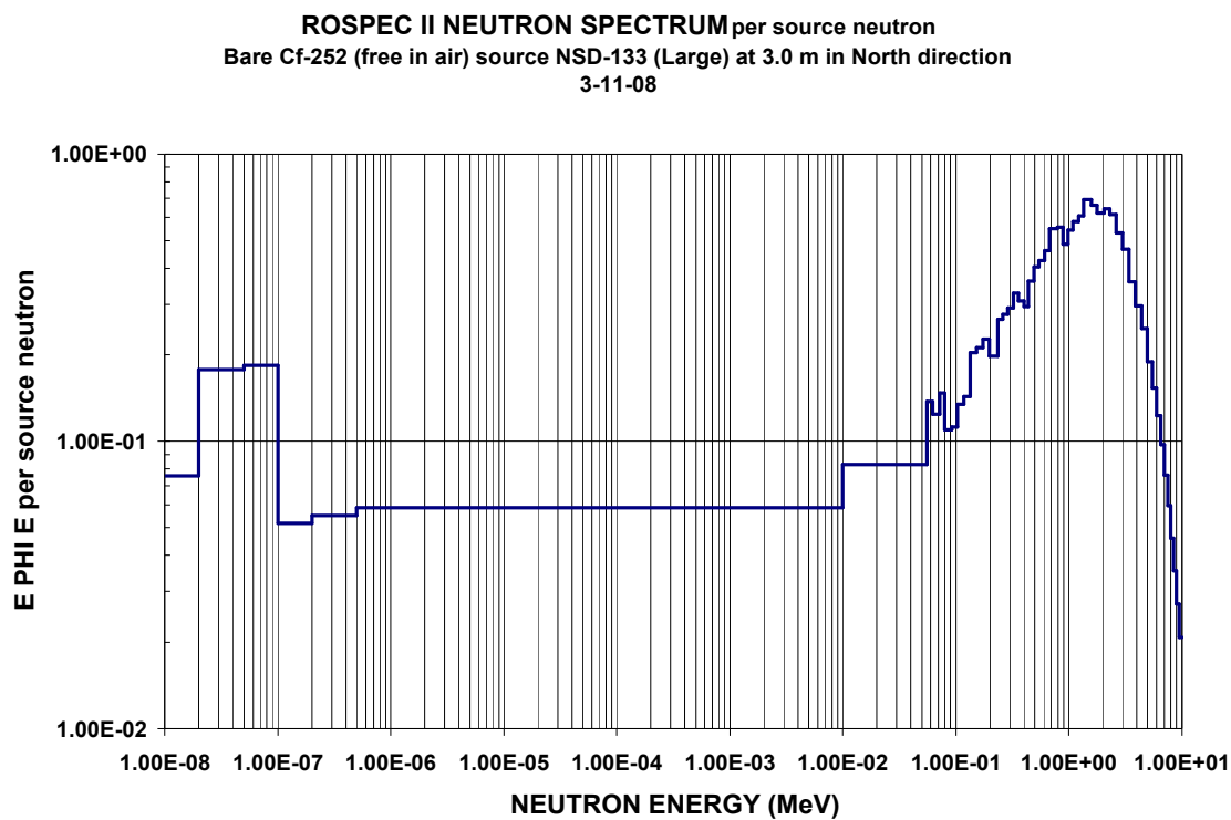
Figure C-18. Neutron spectra from bare ^{252}\text{Cf} (free in air) source NSD-133 (Large) at 3.0 m in North direction
