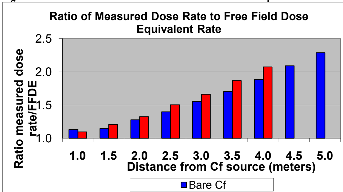
Figure 21. Ratio of measured dose rate to Free Field Dose Equivalent rate
