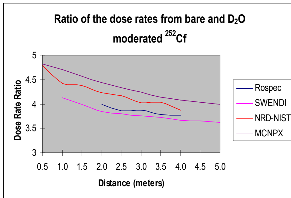
Figure 20. Ratio of the dose rates from bare ^{252}\text{Cf} and \text{D}_2\text{O} moderated ^{252}\text{Cf} sources in the North direction
