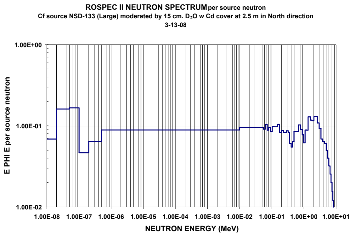
Figure C-16. Neutron spectra from ^{252}\text{Cf} source NSD-133 (Large) moderated by 15 cm. \text{D}_2\text{O} w Cd cover at 2.5 m, in North direction
