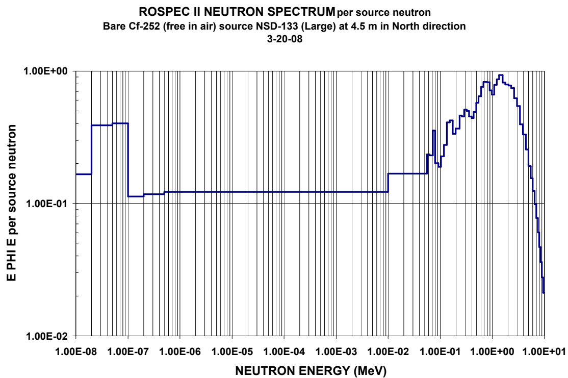
Figure C-29. Neutron spectra from bare ^{252}\text{Cf} (free in air) source NSD-133 (Large) at 4.5 m in North direction
