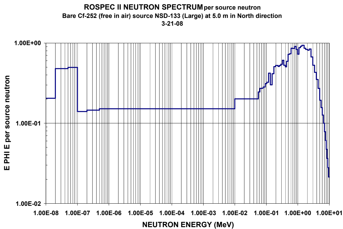
Figure C-30. Neutron spectra from bare ^{252}\text{Cf} (free in air) source NSD-133 (Large) at 5.0 m in North direction
