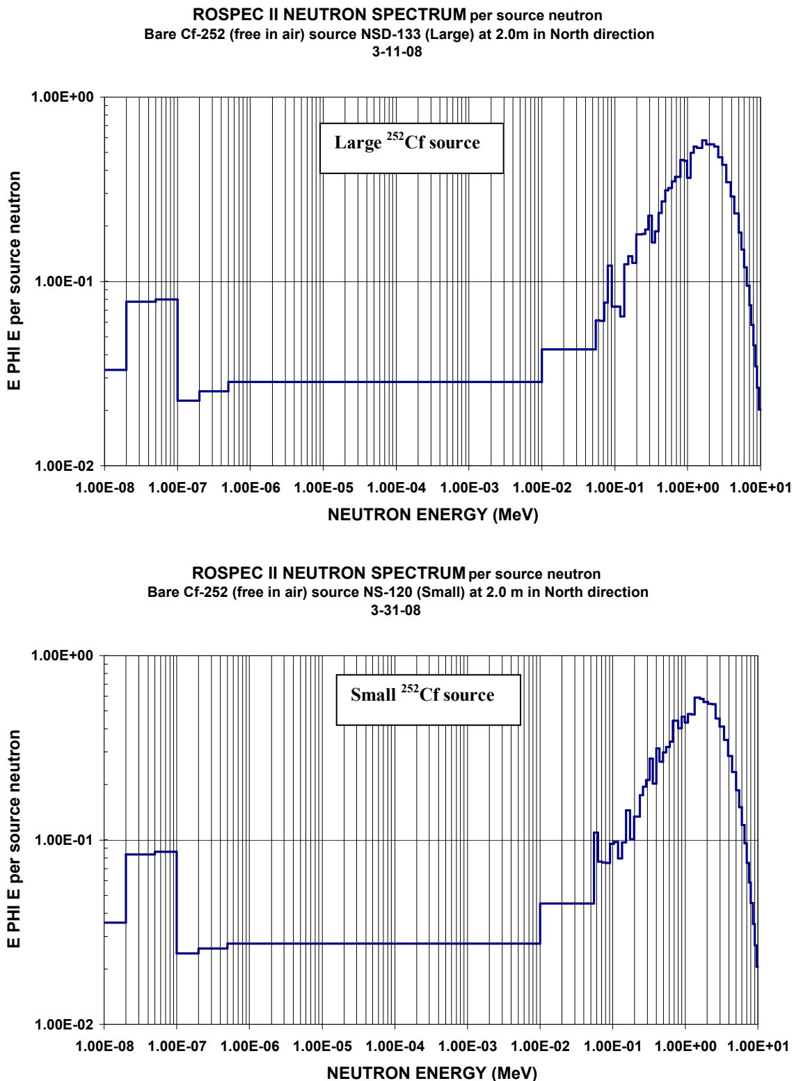
Figure 12. Spectra from Large and Small Bare ^{252}\text{Cf} sources at 2.0 meters
