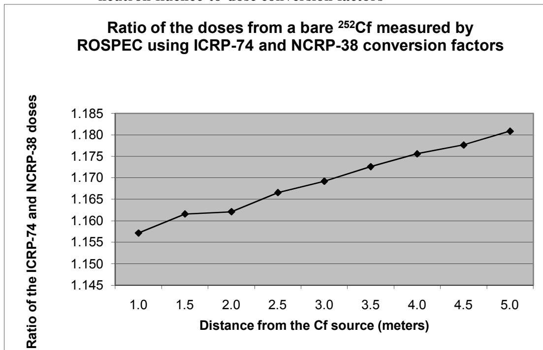
Figure 23. Comparison of the measured dose rates using ICRP-74 and NCRP-38 neutron fluence-to-dose conversion factors
