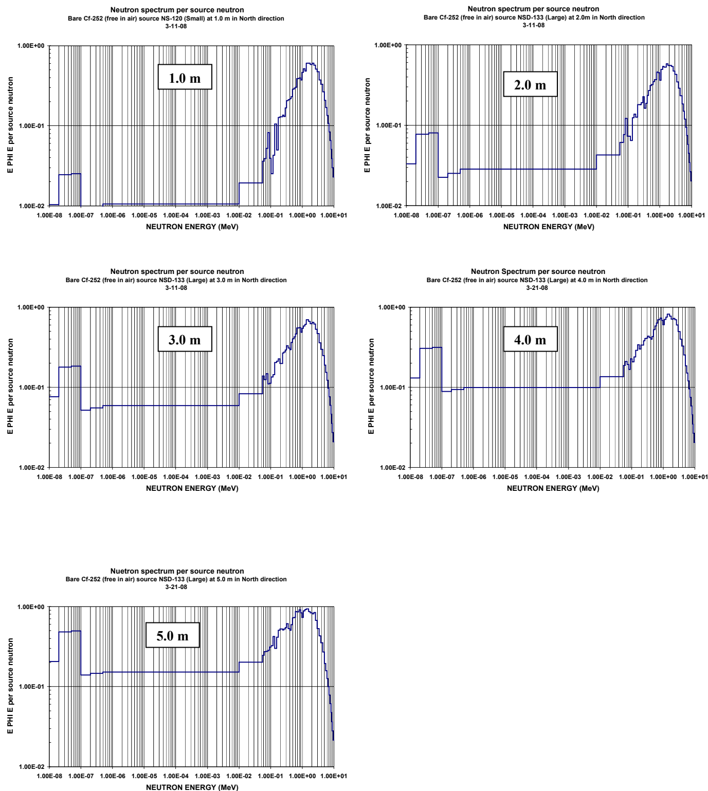
Figure 13. Neutron spectra at different distances (1.0 – 5.0 meters) from a bare ^{252}\text{Cf} source in North direction
