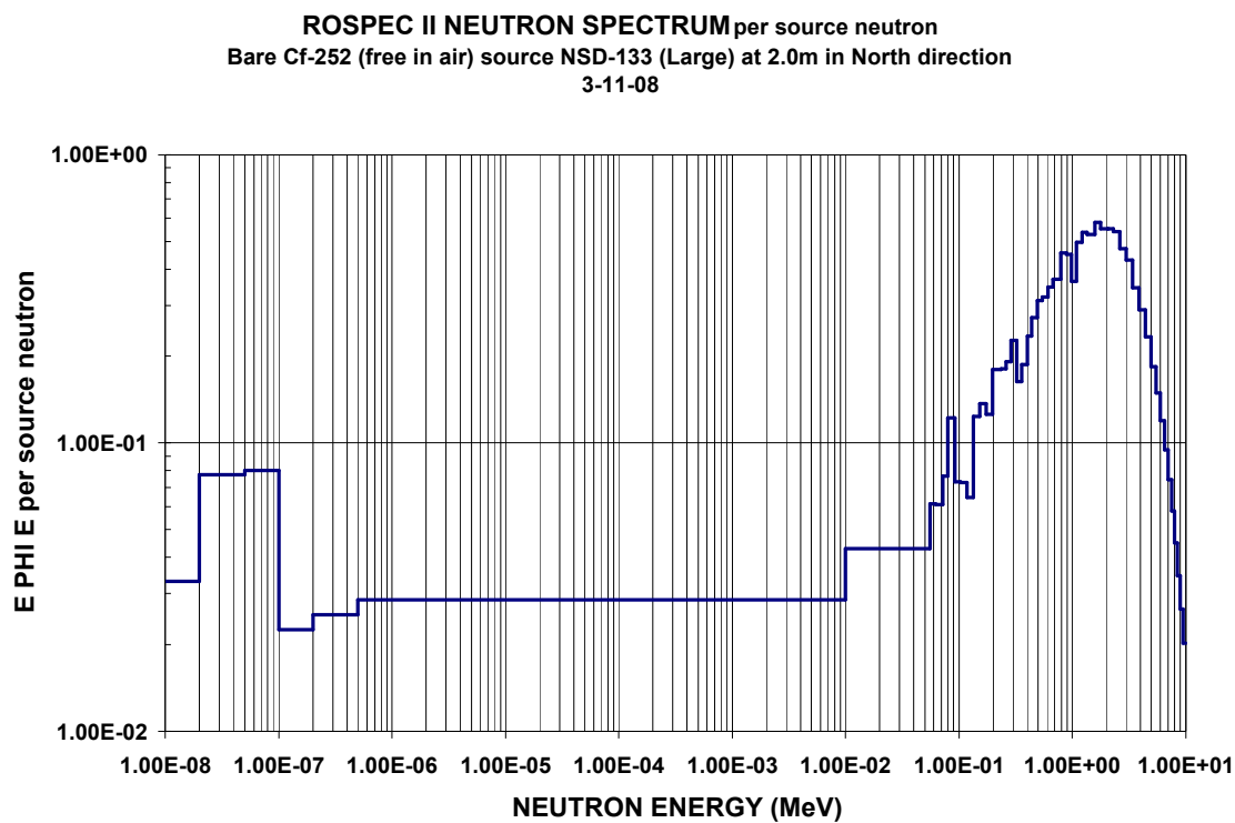
Figure C-9. Neutron spectra from bare ^{252}\text{Cf} (free in air) source NSD-133 (Large) at 2.0m in North direction
