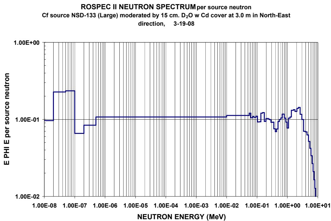
Figure C-23. Neutron spectra from ^{252}\text{Cf} source NSD-133 (Large) moderated by 15 cm. \text{D}_2\text{O} w Cd cover at 3.0 m in North-East direction
