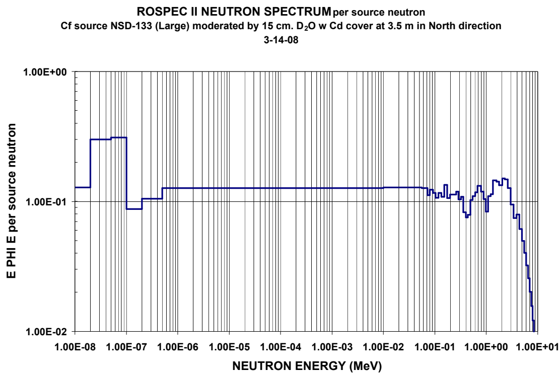
Figure C-25. Neutron spectra from ^{252}\text{Cf} source NSD-133 (Large) moderated by 15 cm. \text{D}_2\text{O} w Cd cover at 3.5 m in North direction
