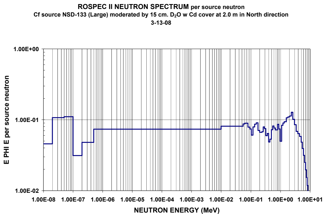
Figure C-11. Neutron spectra from ^{252}\text{Cf} source NSD-133 (Large) moderated by 15 cm. \text{D}_2\text{O} w Cd cover at 2.0 m in North direction
