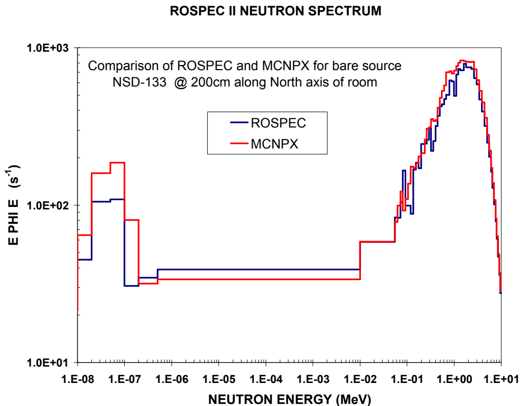
Figure 10. Absolute comparison of ROSPEC and MCNPX spectra for bare 252 Cf
