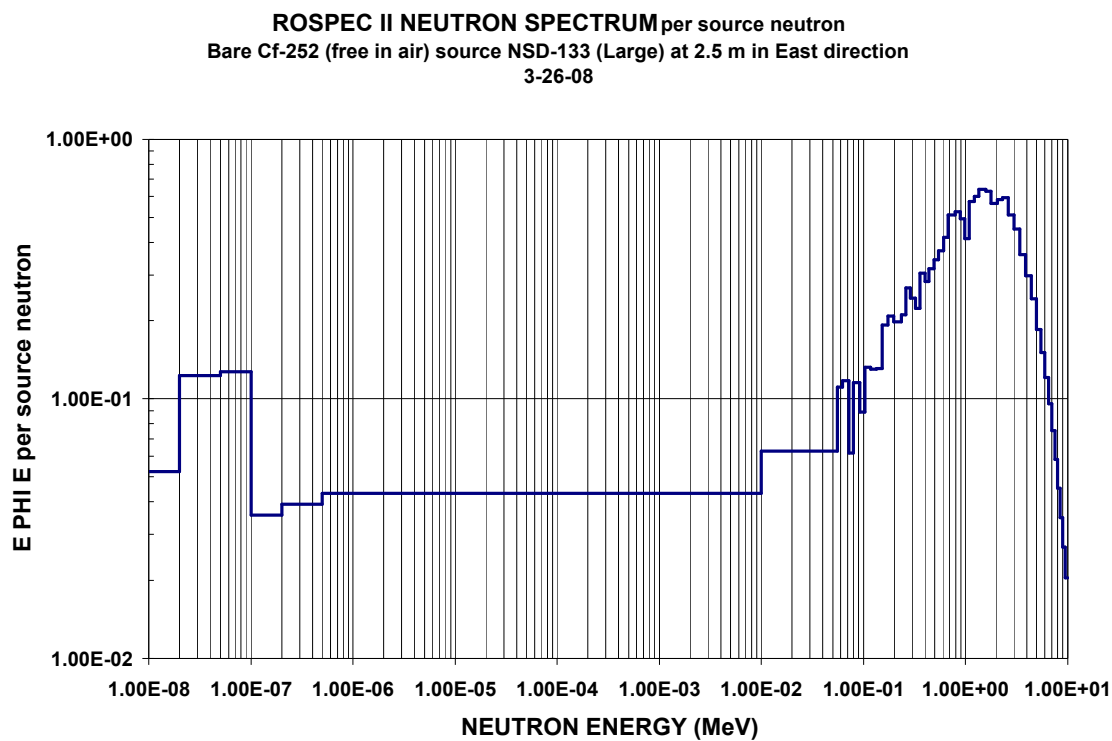
Figure C-15. Neutron spectra from bare ^{252}\text{Cf} (free in air) source NSD-133 (Large) at 2.5 m in East direction
