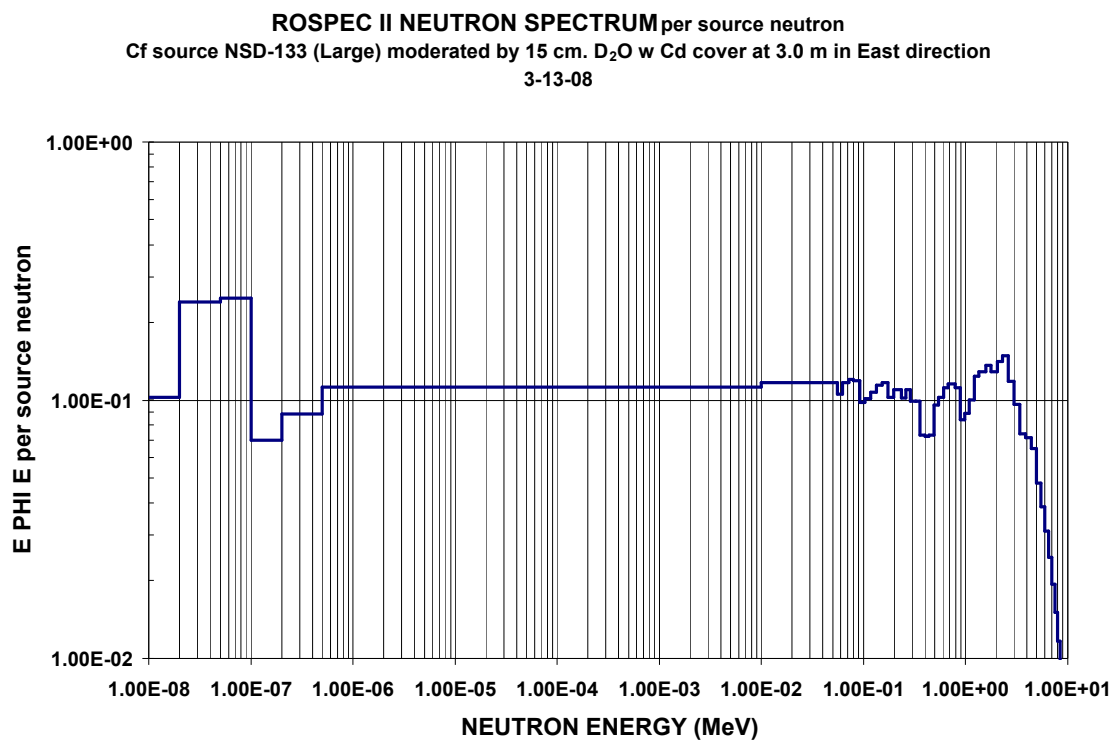
Figure C-22. Neutron spectra from ^{252}\text{Cf} source NSD-133 (Large) moderated by 15 cm. \text{D}_2\text{O} w Cd cover at 3.0 m in East direction
