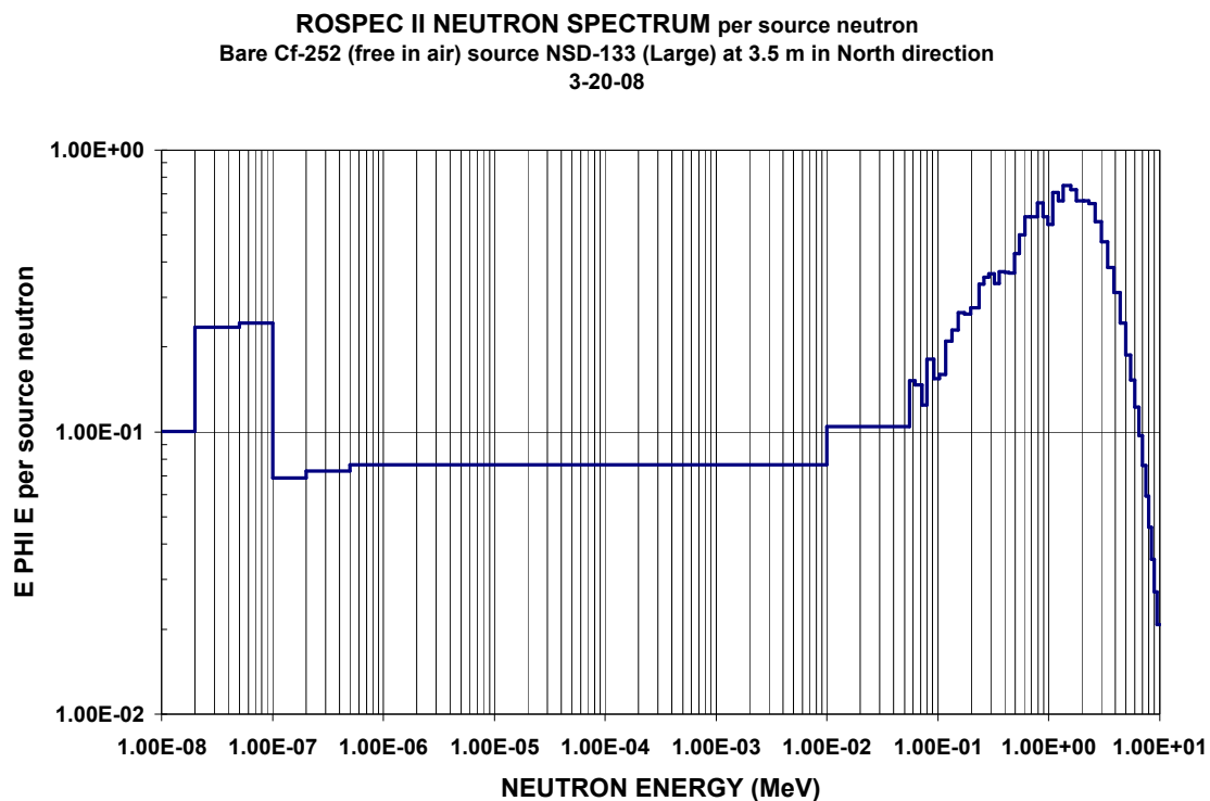
Figure C-24. Neutron spectra from bare ^{252}\text{Cf} (free in air) source NSD-133 (Large) at 3.5 m in North direction
