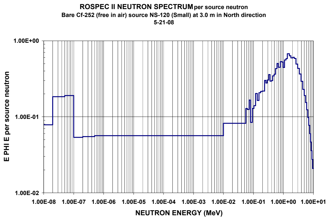
Figure C-17. Neutron spectra from bare ^{252}\text{Cf} (free in air) source NS-120 (Small) at 3.0 m in North direction
