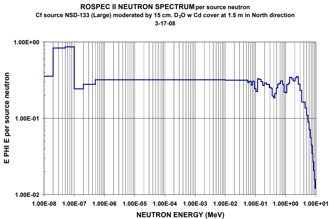
Figure C-7. Neutron spectra from ^{252}\text{Cf} source NSD-133 (Large) moderated by 15 cm. \text{D}_2\text{O} w Cd cover at 1.5 m in North direction
