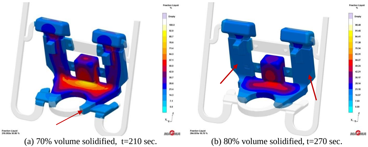
Figure 4.5.23 Potential areas where contraction stresses can develop and promote mechanical hot tearing are shown by the arrows.
