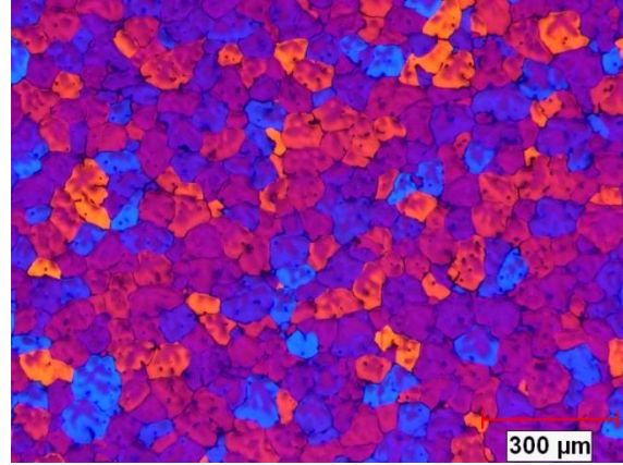
(b) N6080-10, 330C, refined, 50x.
