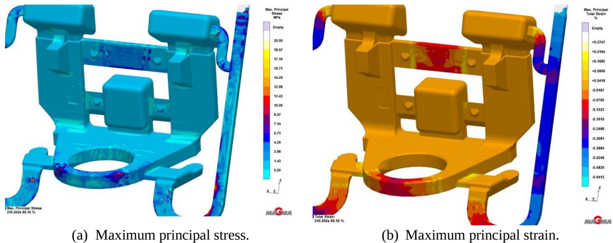
Figure 4.5.25 Predicted maximum principal stress and maximum principal strain when die was opened after 120 seconds.
