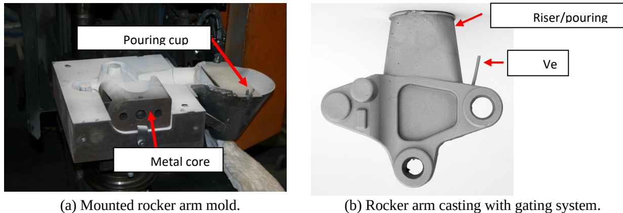
Figure 4.3.3 Photographs of a mounted rocker arm mold and rocker arm casting.
