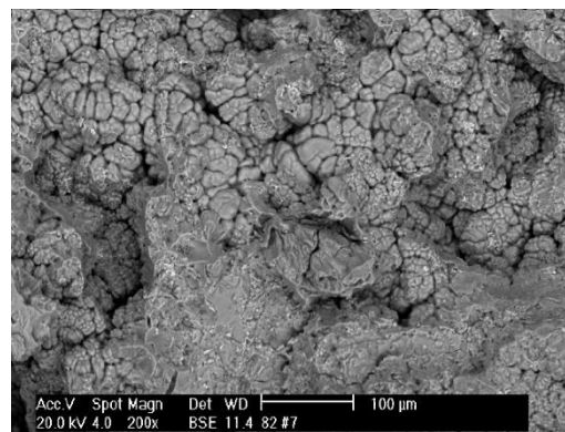
(b) N6082-#7, 200x.
