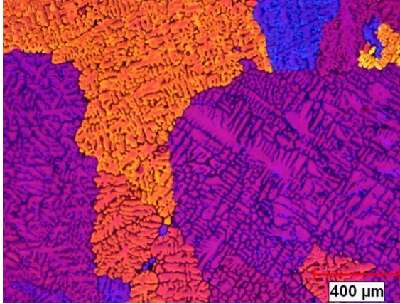
(a) N6080-1, 330C, not refined, 37.5x.
