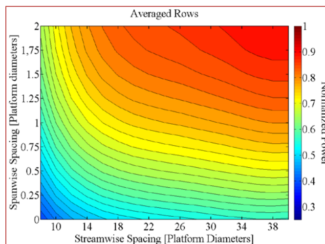
Figure 7. The average of the power captured by all four rows in Scenario 2 as a function of spanwise and streamwise spacing.
