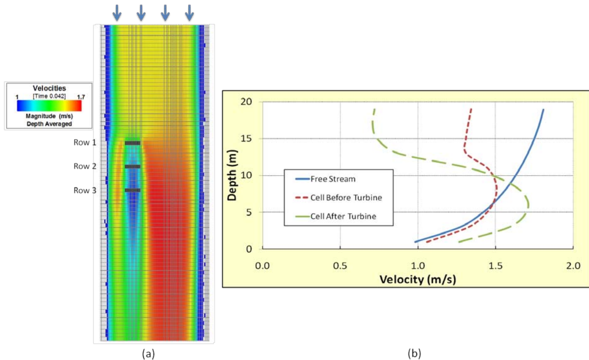
Figure 8. Environmental effects on an unoptimized array. (a) An unoptimized array layout and its effect on the channel velocity. (b) The velocity profile before and after the introduction of the MHK array.
