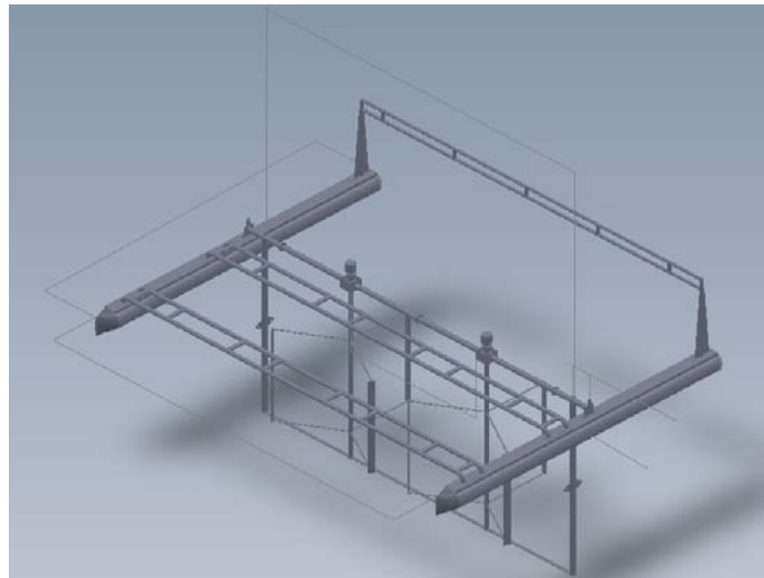
Figure 2. Two crossflow turbines attached to a floating platform that is modeled in the SNL-EFDC simulations.
