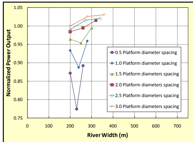
Figure 5. Results of normalized power for increasing spanwise spacing (Scenario 1).
