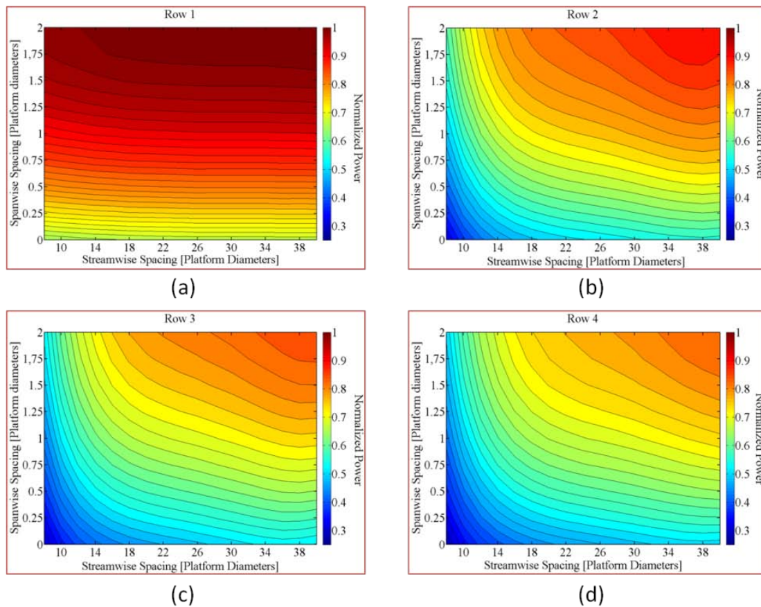
Figure 6. Normalized power with changing streamwise and spanwise spacing for (a) row 1, (b) row 2, (c) row 3, and (d) row 4.
