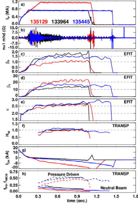
Fig. 6. High- \kappa discharges designed to maximize the non-inductive fraction (black), the pulse length (blue), and \beta_T (red).
