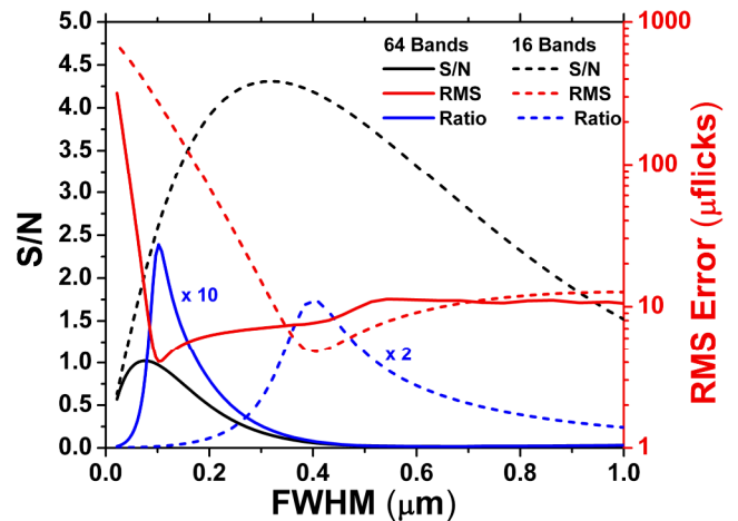
Figure 7: Reconstructed S/N and RMS error for spectral configurations of 16 and 64 channels as a function of the mean FWHM of the channels.
