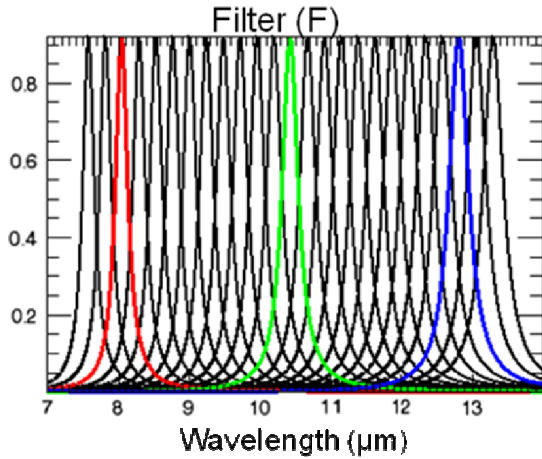
Figure 2: 25 equally spaced spectral filters which span the LWIR spectral domain.
