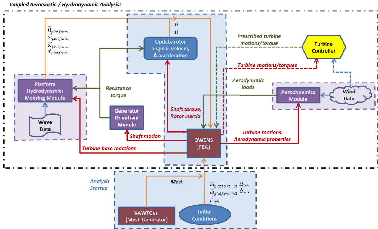
Figure 1. Analysis framework for the OWENS toolkit
