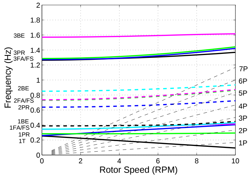
Figure 14. Campbell diagram of land-based 2 bladed SNL 5MW VAWT
