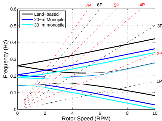
Figure 15. Tower mode Campbell diagram of 3 bladed 5MW VAWT for land and monopile support conditions
