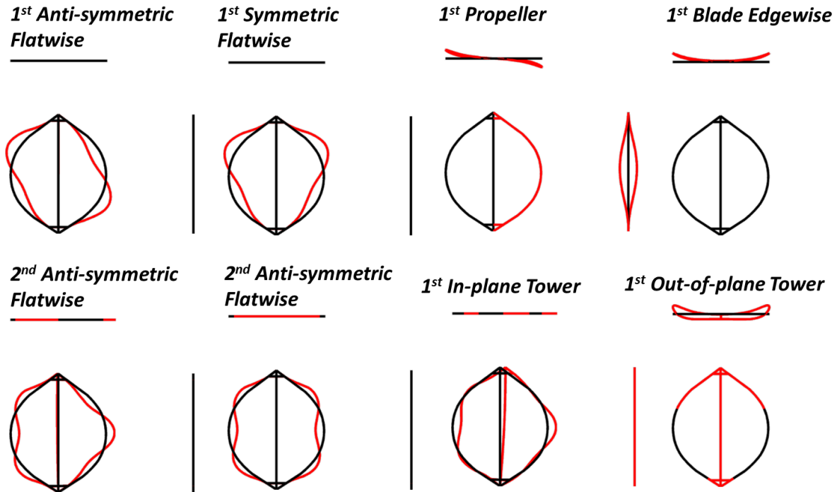
Figure 9. Lower mode shapes for SNL 34-meter VAWT
