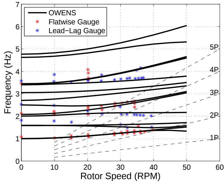
Figure 8. Campbell diagram of SNL 34-meter VAWT
