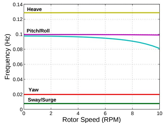
Figure 20. Rigid body mode Campbell diagram of 2 bladed 5MW VAWT on barge platform
