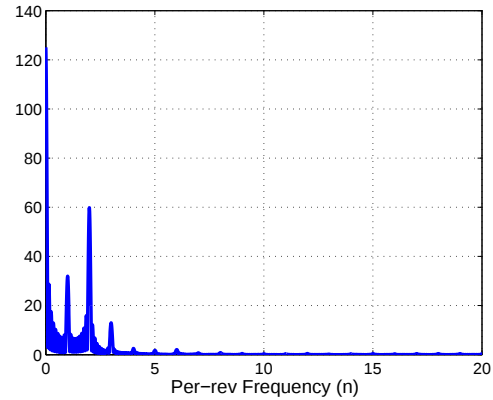
Figure 5. FFT of effective axial force on a single blade vs. normalized azimuth
