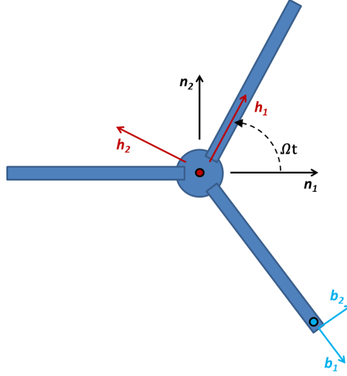
Figure 3. Illustration of various coordinate systems considered in blade/tower forcing
