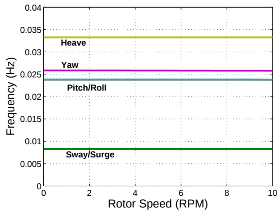
Figure 19. Rigid body mode Campbell diagram of 2 bladed 5MW VAWT on spar buoy platform
