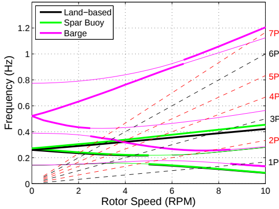
Figure 17. Tower mode Campbell diagram of 3 bladed 5MW VAWT for land and floating support conditions
