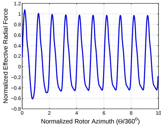
Figure 4. Effective radial force on a single blade vs. normalized azimuth
