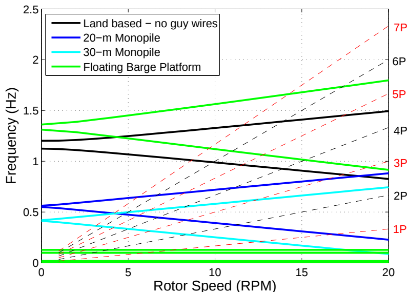
Figure 10. Campbell diagram of SNL 34-meter VAWT tower modes for various support conditions
