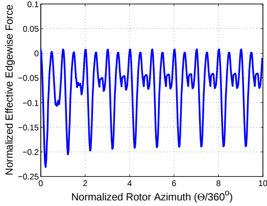
Figure 6. Effective edgewise force on a single blade vs. normalized azimuth
