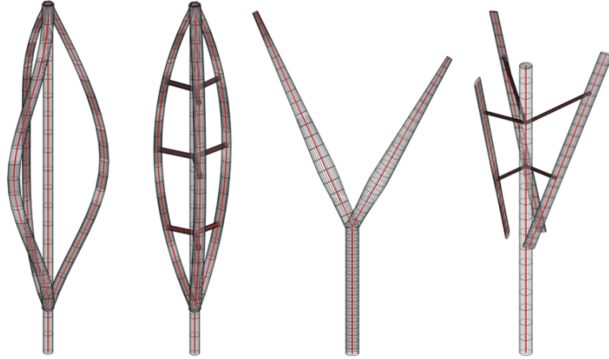
Figure 2. Arbitrary VAWT configurations produced by VAWTGen
