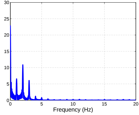
Figure 7. FFT of effective edgewise force on a single blade vs. normalized azimuth
