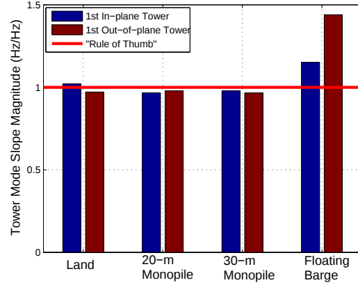
Figure 12. Tower mode slopes for various support conditions
