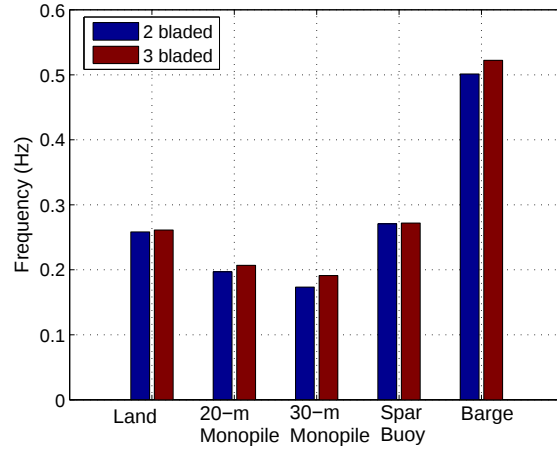
Figure 21. Parked tower mode frequencies for 2 and 3 bladed SNL 5MW VAWT on various support conditions
