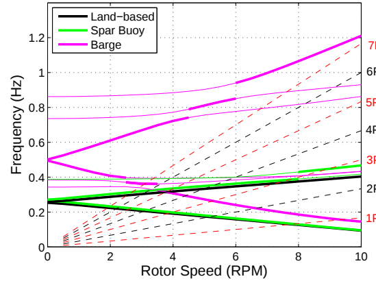
Figure 18. Tower mode Campbell diagram of 2 bladed 5MW VAWT for land and floating support conditions
