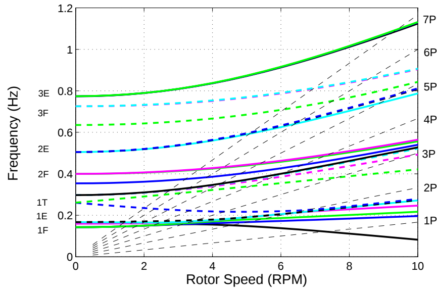
Figure 13. Campbell diagram of land-based 3 bladed SNL 5MW VAWT
