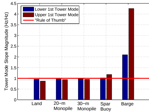
Figure 23. Tower mode slope for 2 bladed SNL 5MW VAWT on various support conditions
