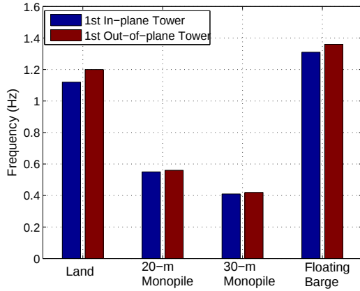
Figure 11. Parked tower mode frequencies for various support conditions
