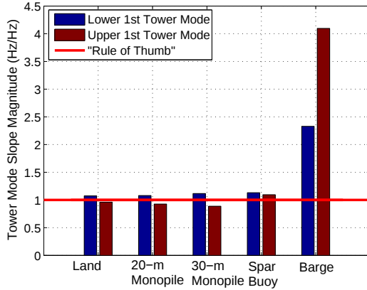
Figure 22. Tower mode slope for 3 bladed SNL 5MW VAWT on various support conditions
