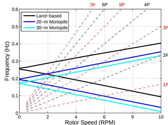
Figure 16. Tower mode Campbell diagram of 2 bladed 5MW VAWT for land and monopile support conditions
