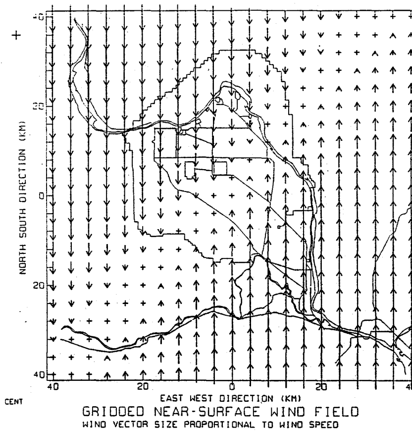
Figure D.13. Wind Field Plot for Test Case 4
