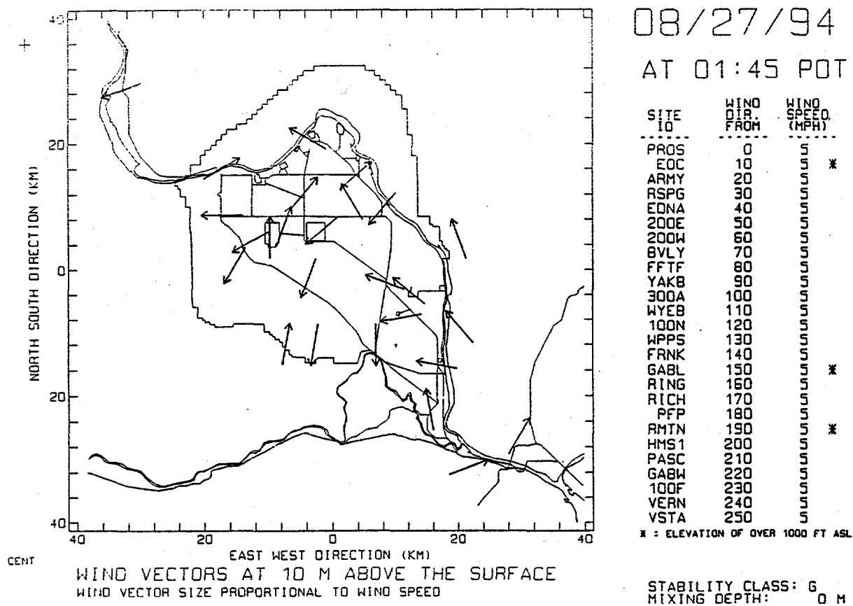
Figure D.9. Plot of Monitored Winds for Test Case 3 at 01:45 PDT. All stations are reporting a wind speed of 5 mph. Wind directions range from 0° to 250°.
