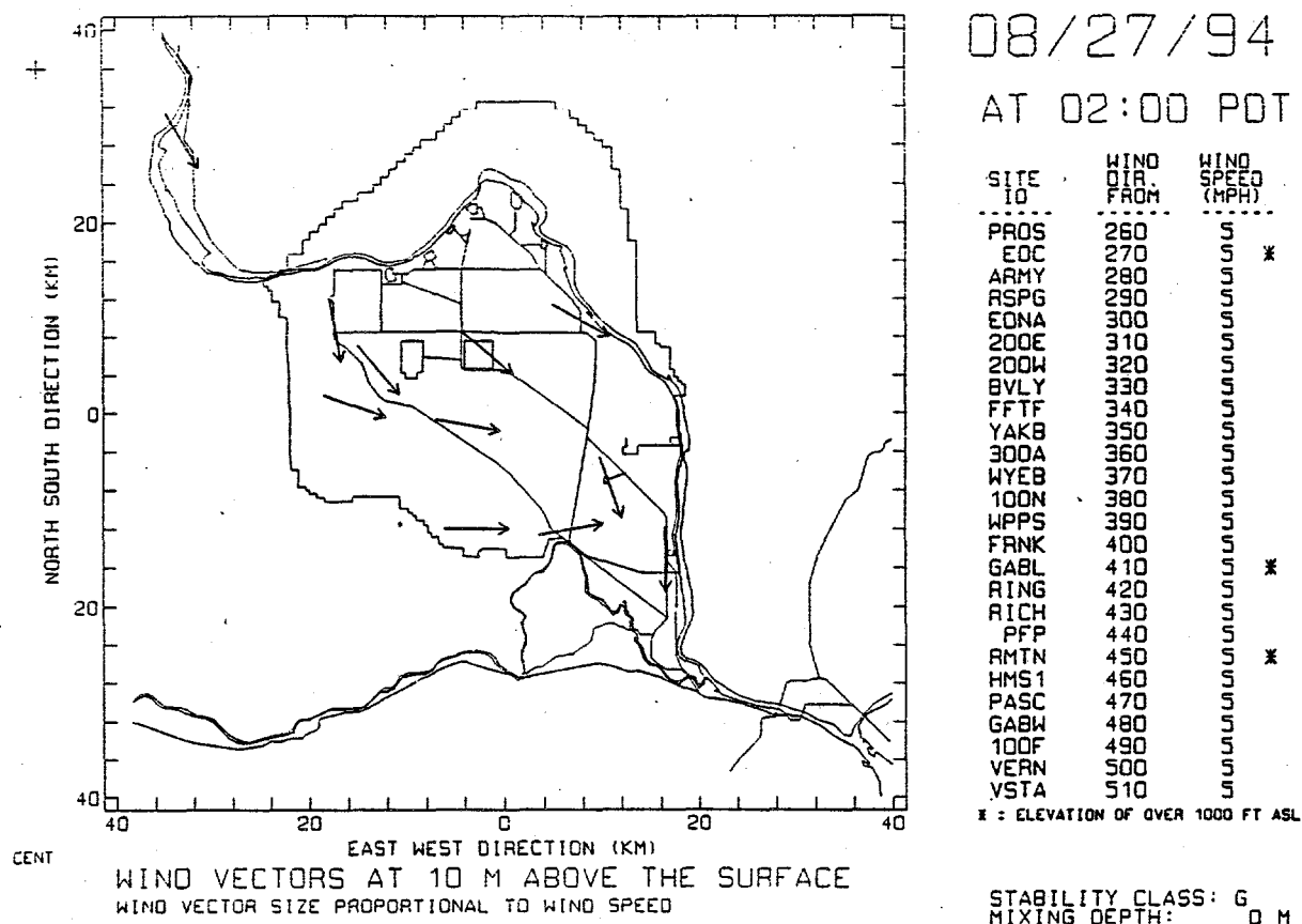
Figure D.10. Plot of Monitored Winds for Test Case 3 at 02:00 PDT. All stations are reporting a wind speed of 5 mph. Wind directions range from 260° to 510°; wind vectors are not plotted when directions are greater than 360°.
