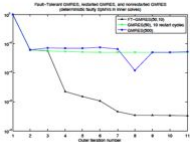
FT-GMRES vs. GMRES on mult_dcop_03 (a Xyce circuit simulation problem).
