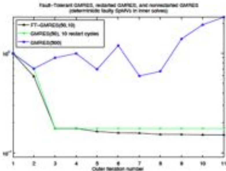
FT-GMRES vs. GMRES on Ill_Stokes (an ill-conditioned discretization of a Stokes PDE).
