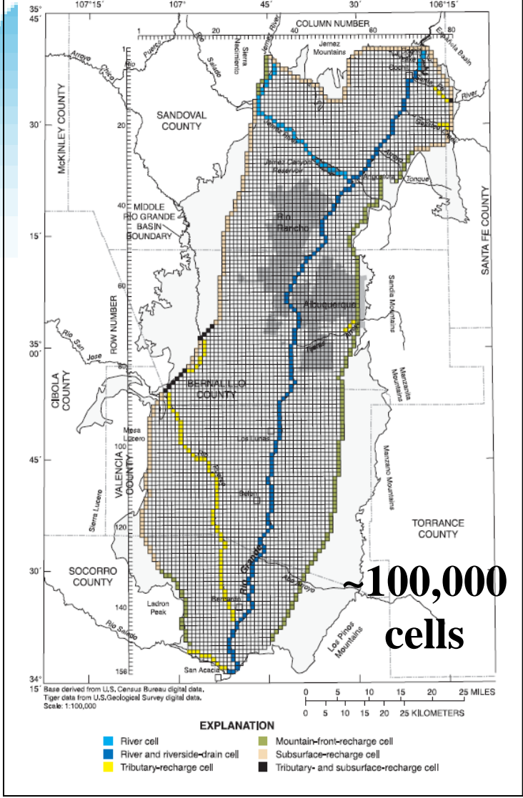
McAda and Barroll 2002, Figure 7. Albuquerque Basin MODFLOW model extent.
