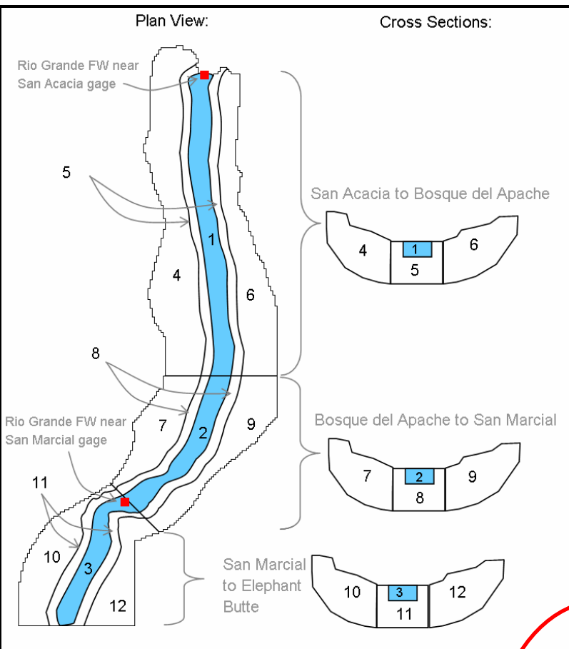
Socorro GW Basin (based on Shafike 2005 model)
