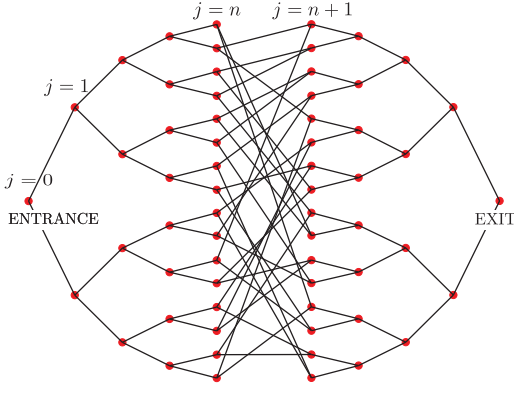
FIG. 1: Two binary trees of depth n = 4 glued randomly. The number of vertices is N = 2^{n+2} - 2 . Each vertex is labeled with a randomly chosen 2n -bit string. j is the column number.
