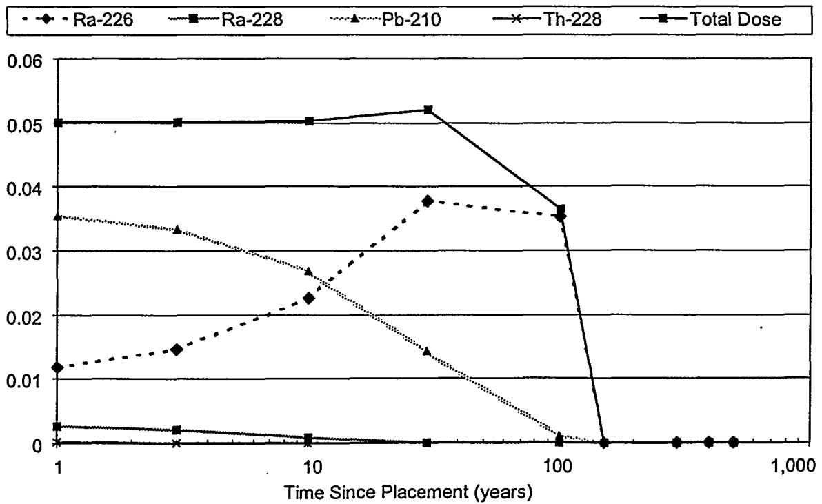
Figure 6. Potential Doses to an Individual from Ingestion of Contaminated Meat
