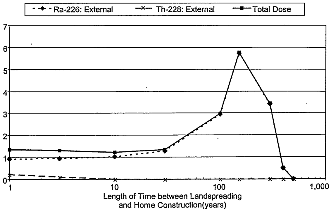
Figure 2. Potential Doses to a Resident of a Home with a Basement Excavated below the Contaminated Zone
