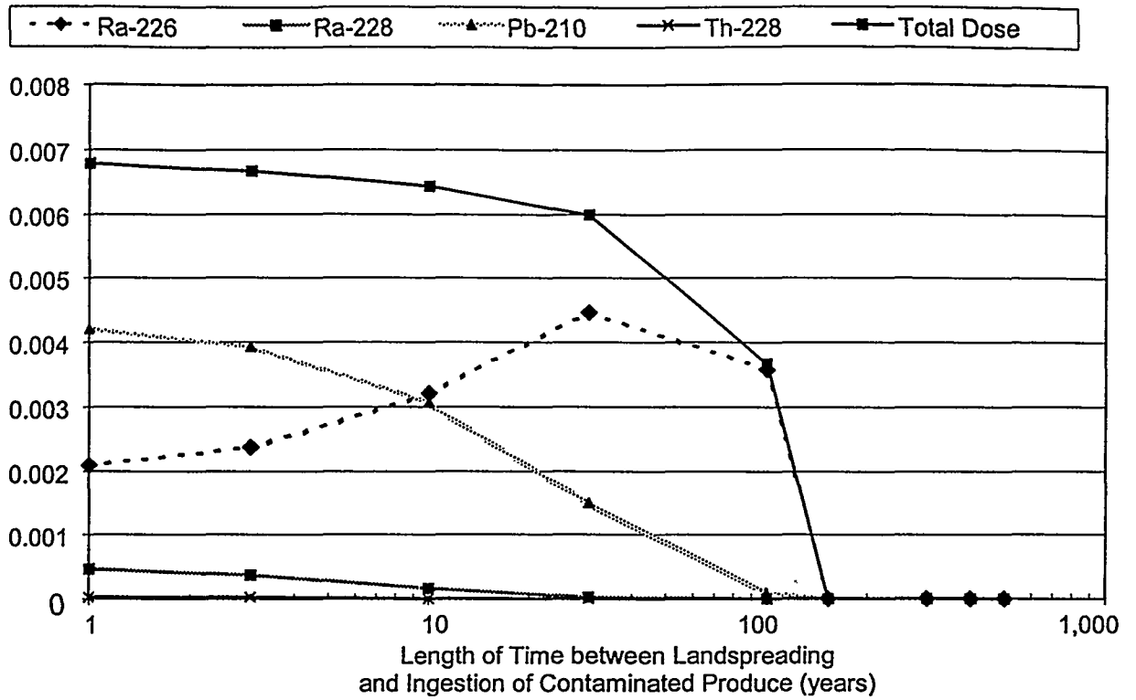
Figure 5. Potential Doses to an Individual from Ingestion of Contaminated Produce
