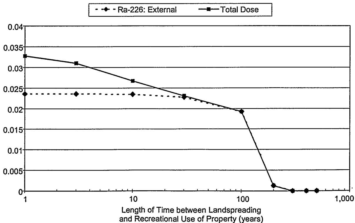
Figure 4. Potential Doses to a Member of the General Public Resulting from Occasional Recreational Use of the Property
