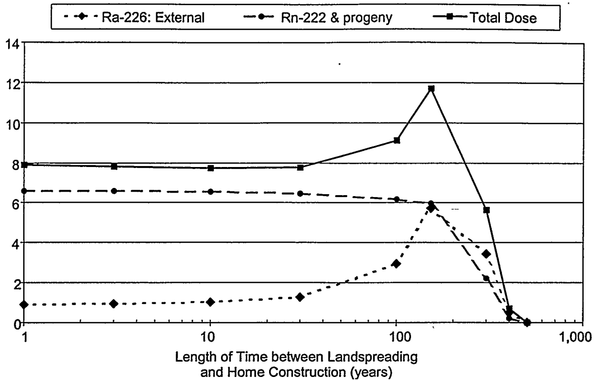
Figure 1. Potential Doses to a Resident of a Home with a Crawl Space Located over the Contaminated Zone
