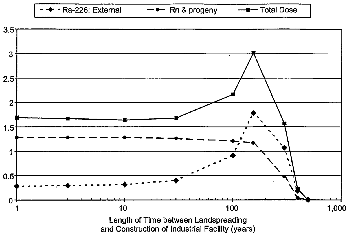
Figure 3. Potential Doses to an Industrial Worker
