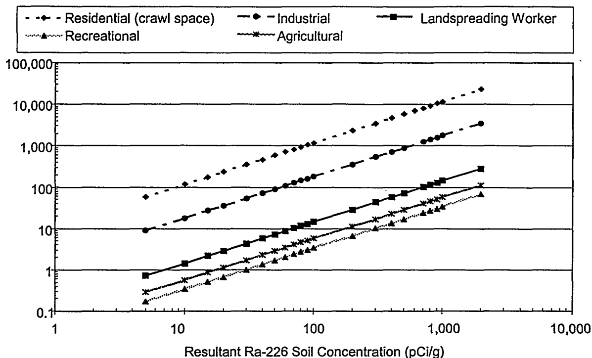
Figure 7. Correlation of Peak Year Dose to NORM Concentration
