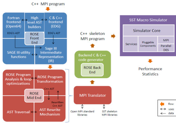
Figure 1: Automatic Translation Framework
