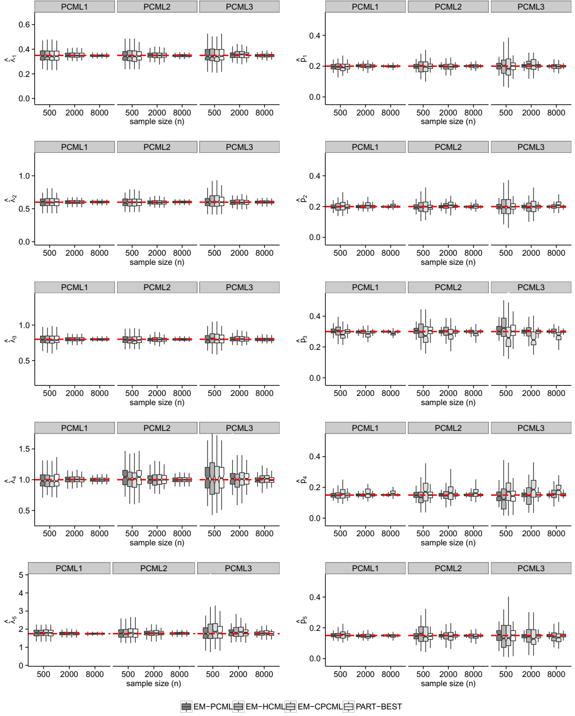
Figure 5.5: MLE of FMM from partially supervised learning on synthetic data sets with U(2,4) censoring time
