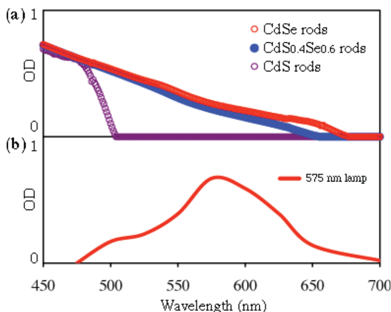
Figure 7. (a) Absorption spectra of colloidal CdS, \text{CdS}_{0.4}\text{Se}_{0.6} , and CdSe nanorods (recorded in toluene with quartz cuvettes), and (b) irradiance spectrum of 575 nm lamp (all spectra were arbitrarily normalized to a maximum optical density OD = 1).
