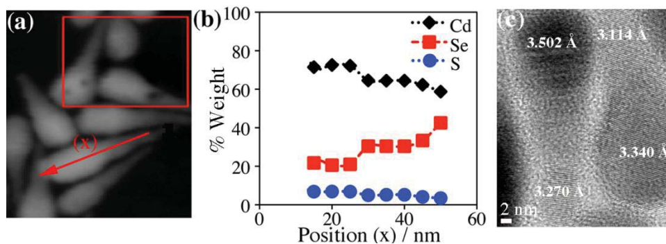
Figure 6. Individual \text{CdS}_{0.42}\text{Se}_{0.58} nanorod sample analyses: (a) Direction and length(x), and (b) composition plot of an EDS line scan (arrow length=50 nm; square area was used for drift correction). (c) HR-TEM micrograph showing interplanar (002) d spacings (perpendicular to c axis) become progressively larger from the tail to the head of the nanorods.
