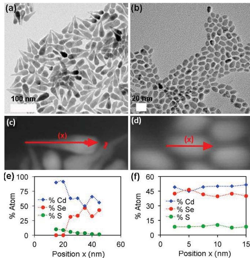
Figure 8. TEM images (a,b) and EDS line scans (c,d,e,f) of axially anisotropic CdS 0.42 Se 0.58 nanorods made with a 9:1 TOPS–TOPSe precursor mixture (a,c,e), and regular CdS 0.34 Se 0.66 nano-rods made with a 9:1 TBPS–TBPSe precursor mixture (b,d,f). Arrows represent 50 nm in (c) and 17.5 nm in (d). Other conditions: Cd(ODPA) 2 , 320°C, 85 min. XRD shows all nanorods have mainly hexagonal (wurtzite) crystal structures.
