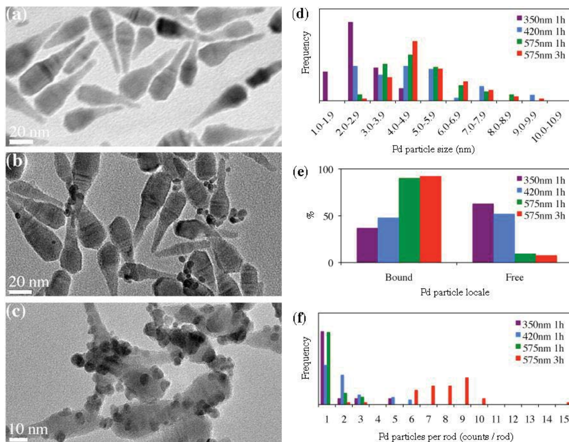
Figure 5. Sample TEM micrographs of CdS 0.4 Se 0.6 nanorods (a), and CdS 0.4 Se 0.6 -Pd heterostructures prepared photochemically at 575 nm, 24 °C for 1 h (b) and 3 h (c). Pd particle size (d), locale (e), and loading per rod (f) histograms for CdS 0.4 Se 0.6 -Pd heterostructures prepared photochemically at 350 nm for 1 h (violet), 420 nm for 1 h (blue), 575 nm for 1 h (green), and 575 nm for 3 h (red) (>50-100 CdS 0.4 Se 0.6 nanorods and >50-300 Pd particles measured in each case).
