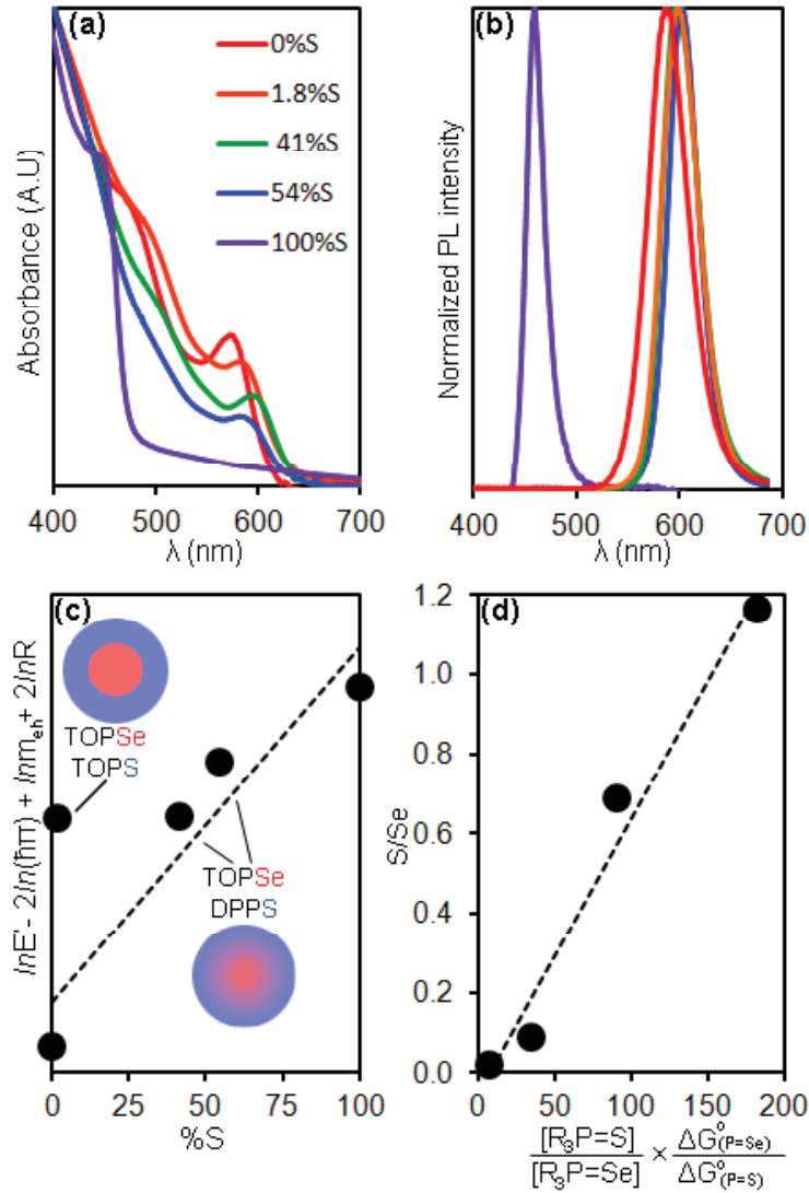
Figure 6. (a) UV-Vis, (b) PL, and (c) size-corrected band gaps of CdS 1-x Se x dots obtained from different R 3 PS–R 3 PSe mixtures. In (c), faster CdSe compared to CdS nucleation with TOPSe–TOPS leads to CdSe/CdS core/shells, whereas concomitant CdSe and CdS nucleation with TOPSe–DPPS leads to CdS 1-x Se x alloys. (d) Sulfur to selenium ratio (S/Se) in CdS 1-x Se x dots as a function of relative precursor concentration and reactivity: \{([R_3PS]/[R_3PSe]) \times [(-\Delta G^{\circ}P=Se)/(-\Delta G^{\circ}P=S)]\} . In (d), k = 0.00688 .
