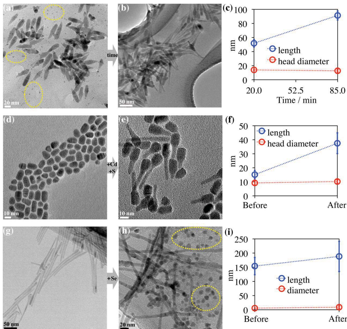
Figure 8. Mechanistic investigations of anisotropic \text{CdS}_{1-x}\text{Se}_x nanorod formation: (a-c) Time evolution of \text{CdS}_{0.68}\text{Se}_{0.32} nanorods: At short reaction times (20 min), the nanorods head has already formed, along with very small CdS nuclei (circled) (a). Over time (85 min total reaction time), small CdS nuclei dissolved and only final \text{CdS}_{0.68}\text{Se}_{0.32} nanorods were observed. (d-i) Independent formation of \text{CdS}_{1-x}\text{Se}_x nanorods from preassembled elements: (d-f) Reaction of CdSe nanorods (d) with Cd and S precursors results in \text{CdS}_{1-x}\text{Se}_x nanorod formation (e), (g-i) whereas reaction of CdS nanorods (g) with Se does not (a few CdSe nuclei, circled, formed instead) (h).
