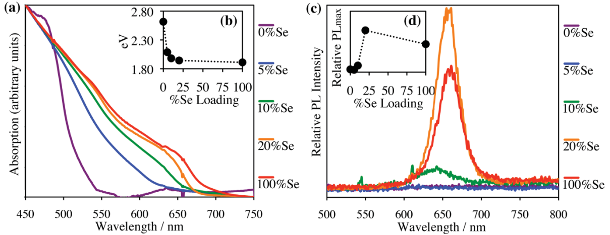
Figure 3. CdS_{1-x}Se_x optical properties: Change in absorption (a), band gap (b), and PL intensity (c, d) with increasing Se loading. (Low solubility of CdS nanorods results in scattering above 500 nm)
