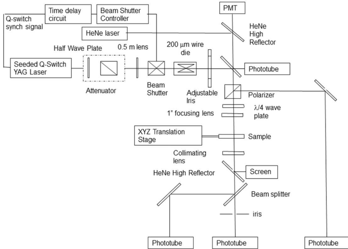
Figure 4: Experimental set-up
