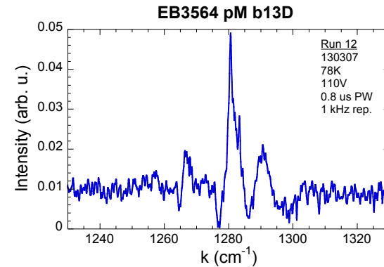
Pulsed Laser Spectrum
