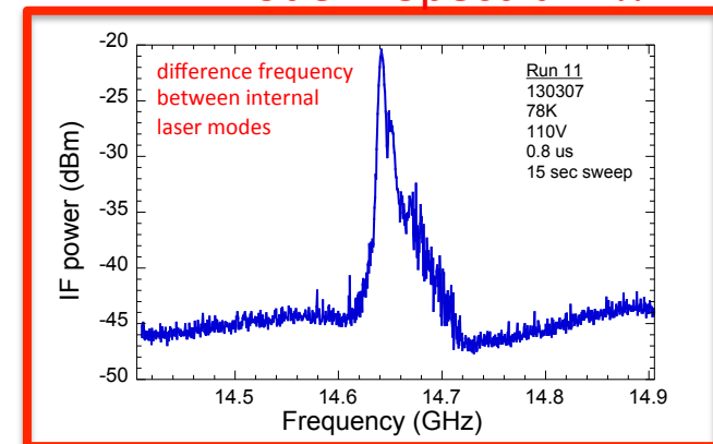
Diode IF Spectrum !!
