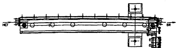
Figure 5: Storage ring AC thick injection septum
