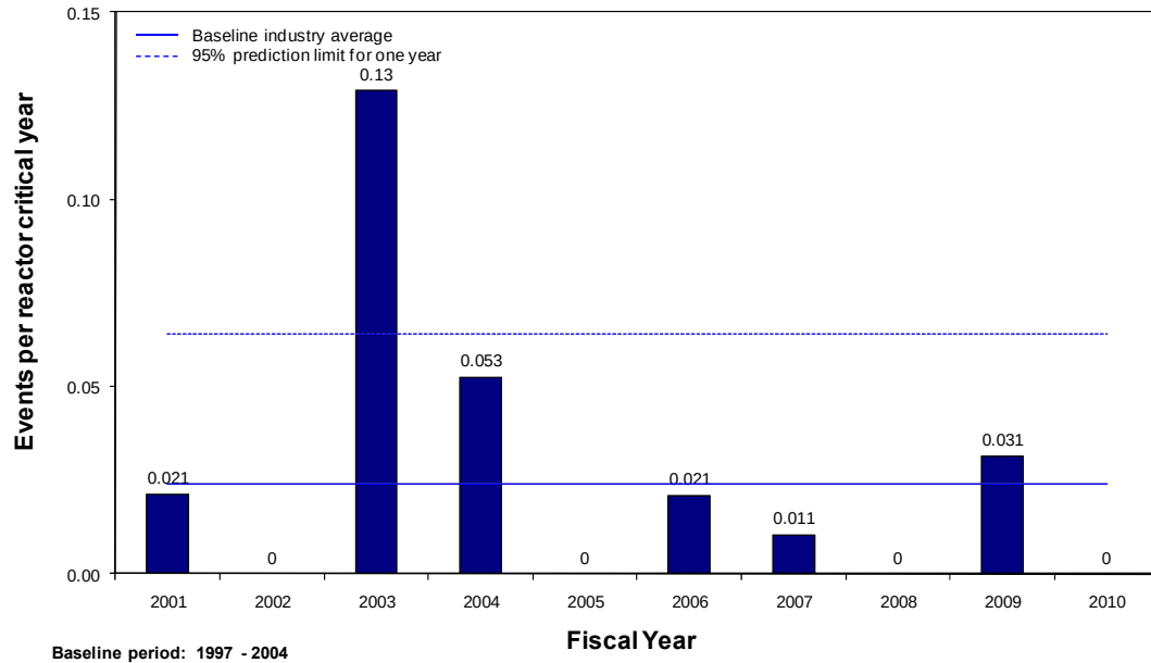
Figure 2. Example of BRIIE Reporting – Loss Offsite Power
