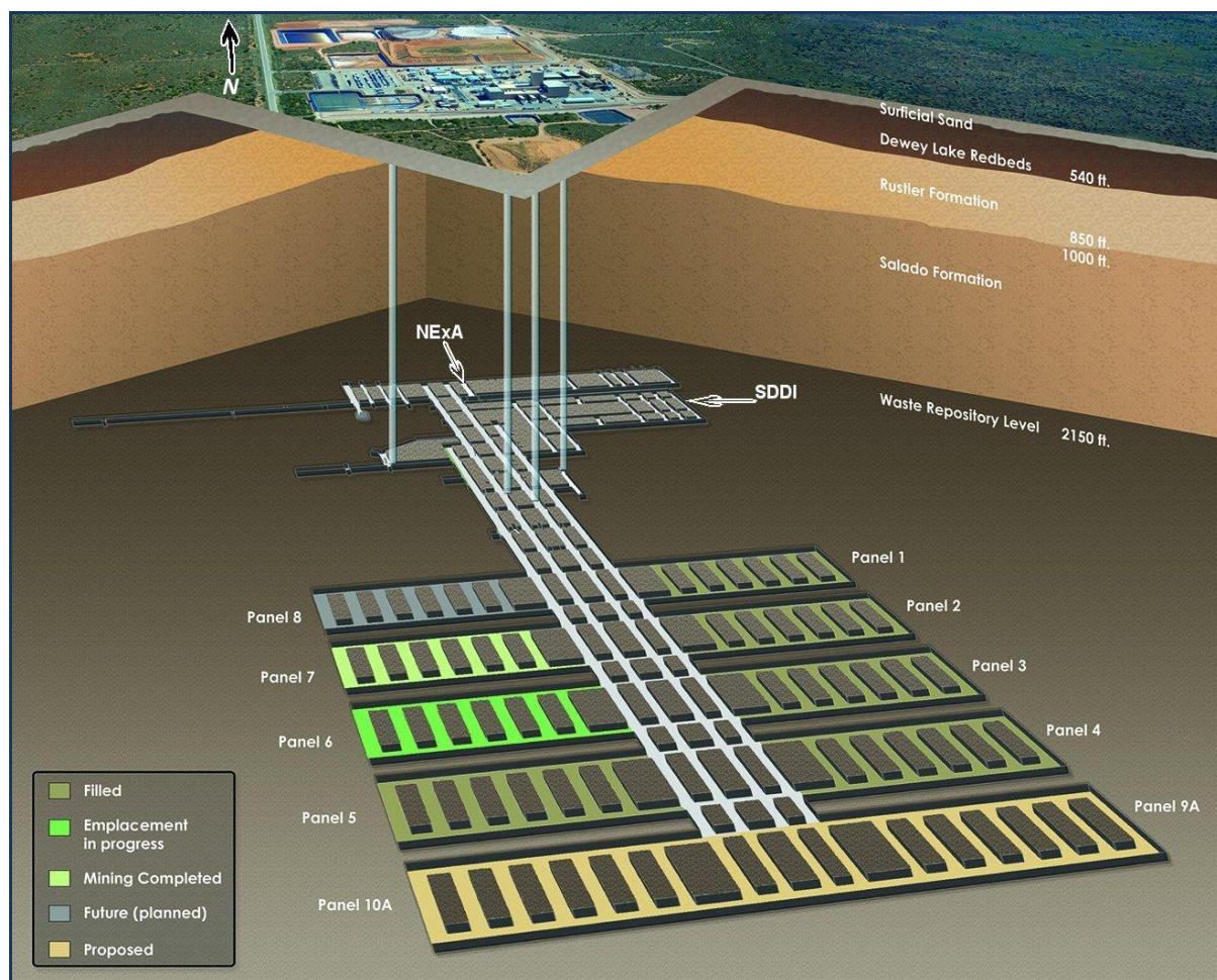
Figure 0.1 WIPP layout
