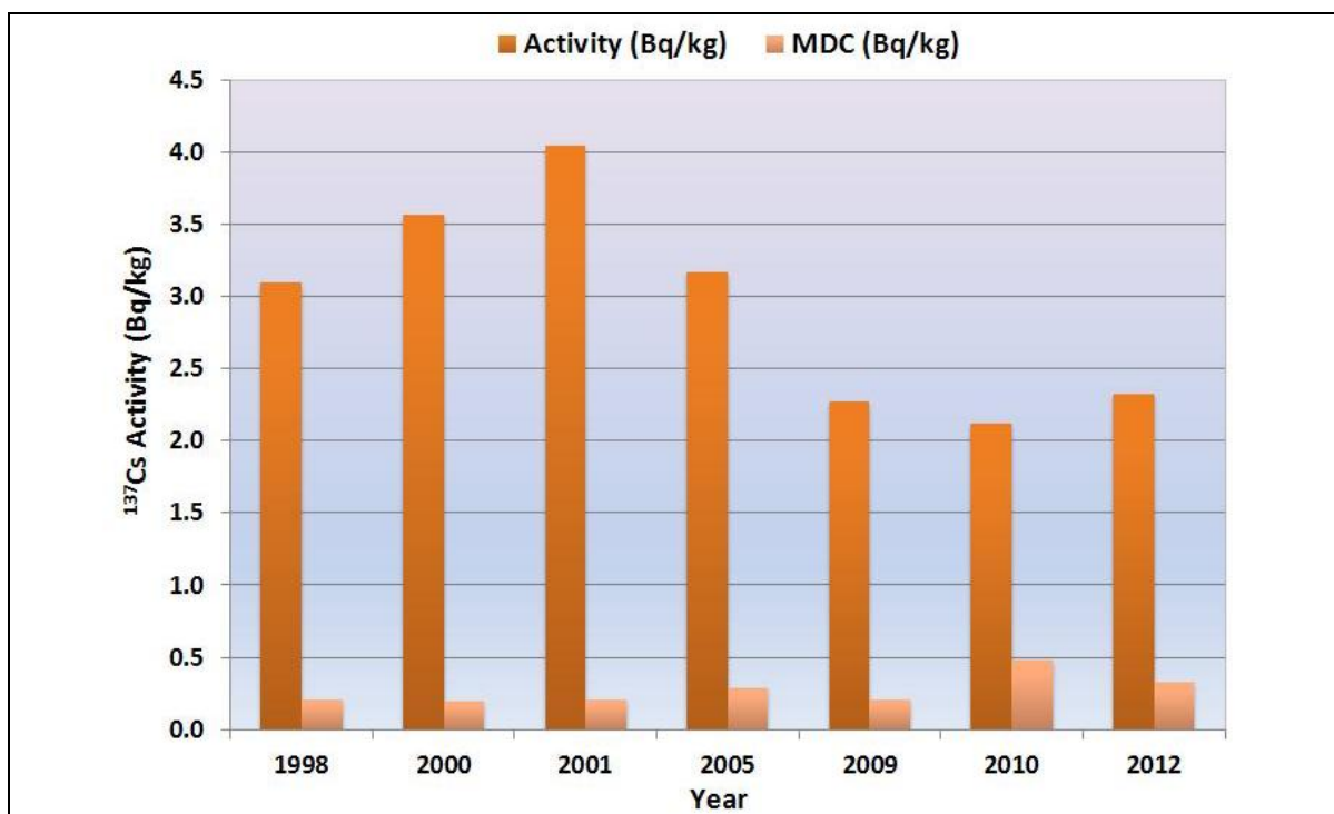
Figure 6.17 Average Activity Concentrations of ^{137}\text{Cs} in Near Field Soil (1998-2012)
