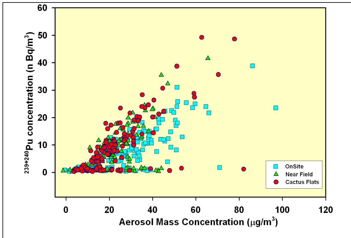
Figure 5.18 Aerosol mass vs. ^{239+240}\text{Pu} activity concentrations in high volume aerosol samples at the three stations near the WIPP site.
