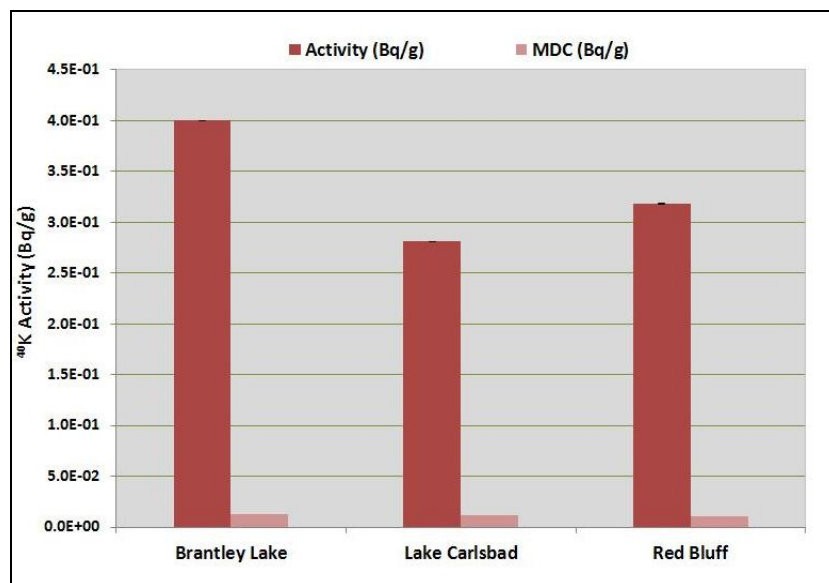
Figure 7.8 ^{40}\text{K} activity concentrations in sediment samples in three regional reservoirs
