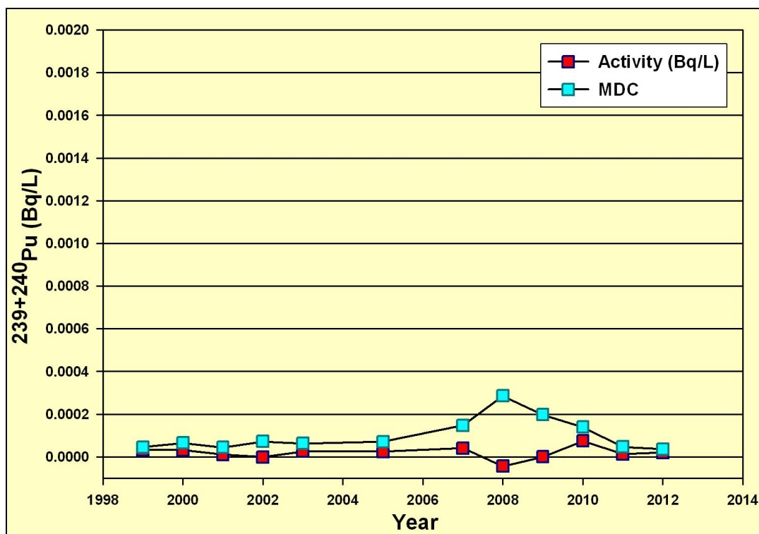
Figure 2.9 ^{239+240}\text{Pu} in Double Eagle Drinking Water from 1999-2012 EPA action level for all alpha emitters is 15pCi/L (0.56 Bq/L)
