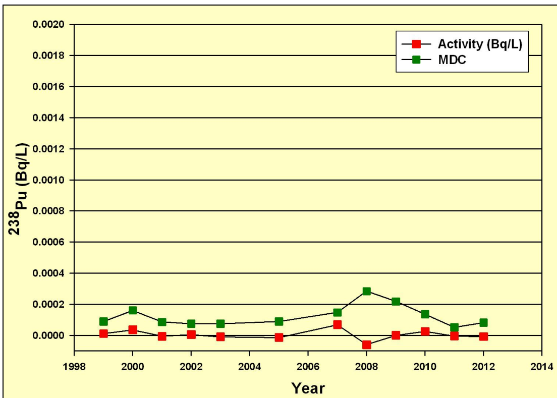
Figure 2.8 ^{238}\text{Pu} in Hobbs Drinking Water from 1998 – 2012
