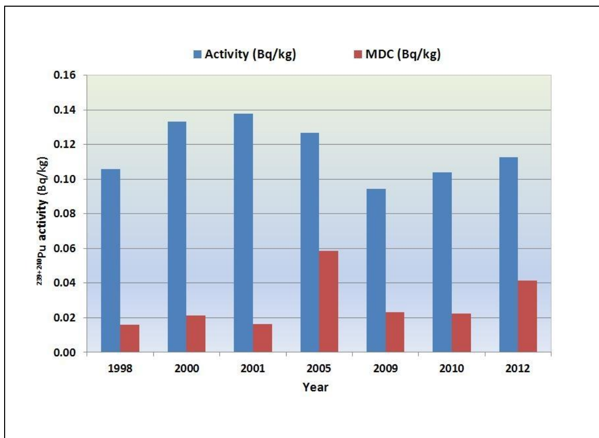
Figure 6.14 Average Activity Concentrations of ^{239+240}\text{Pu} in Near Field Soil (1998-2012)
