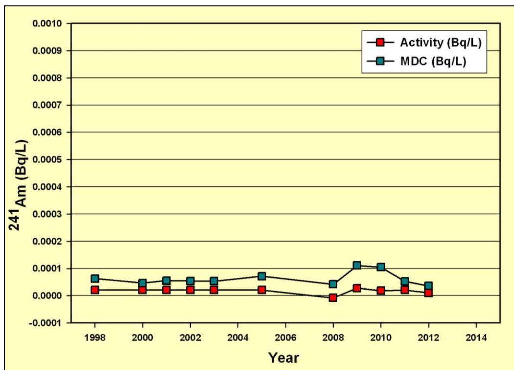
Figure 2.6 ^{241}\text{Am} in Carlsbad Drinking Water from 1998 - 2012 EPA action level for all alpha emitters is 15pCi/L (0.56 Bq/L)
