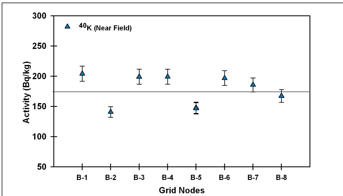
Figure 6.10 Activity Concentrations of ^{40}\text{K} in Soil Samples Collected from Near Field in 2012
