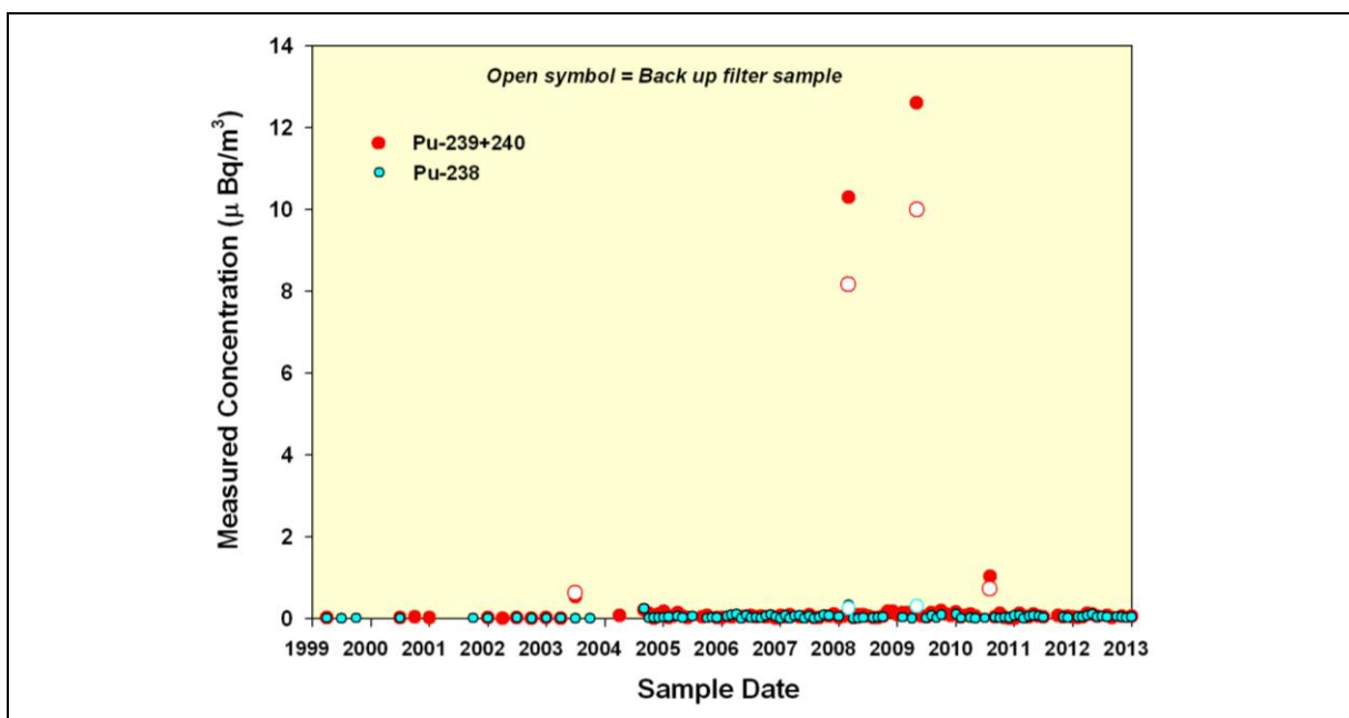
Figure 1.24 Activity Concentrations of ^{239+240}\text{Pu} and ^{238}\text{Pu} in Station A filters (1999-2012)
