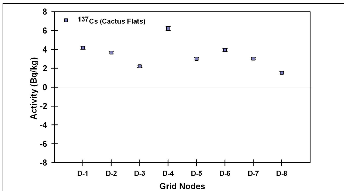
Figure 6.9 Activity Concentrations of ^{137}\text{Cs} in Soil Samples Collected from Cactus Flats in 2012
