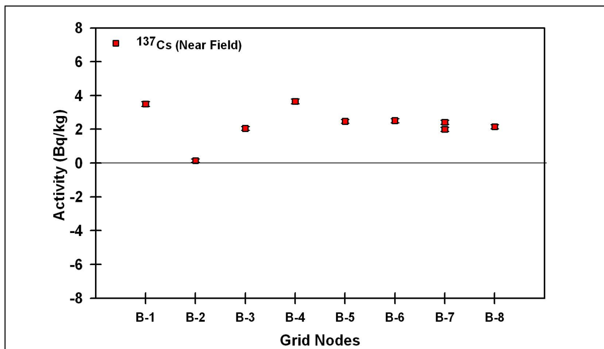
Figure 6.8 Activity Concentrations of ^{137}\text{Cs} in Soil Samples Collected from Near Field in 2012
