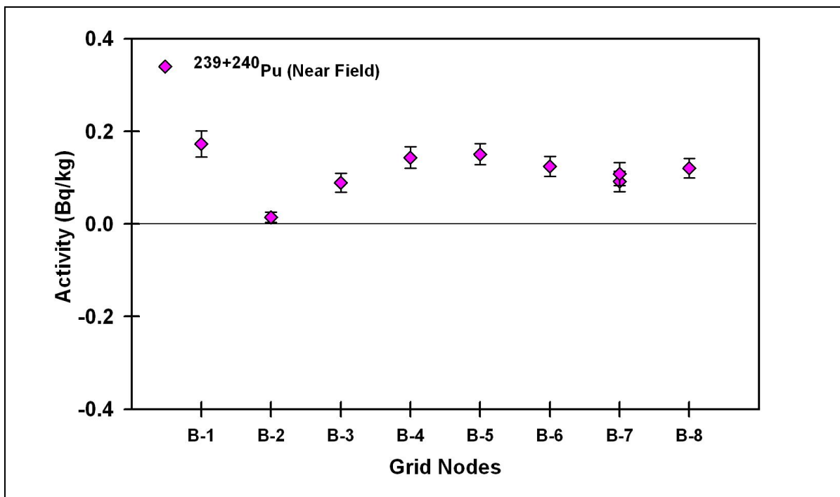
Figure 6.2 Activity Concentrations of ^{239+240}\text{Pu} in Soil Samples Collected from Near Field in 2012
