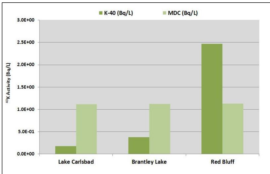
Figure 7.17 ^{40}\text{K} activity concentrations in surface water samples in three regional reservoirs
