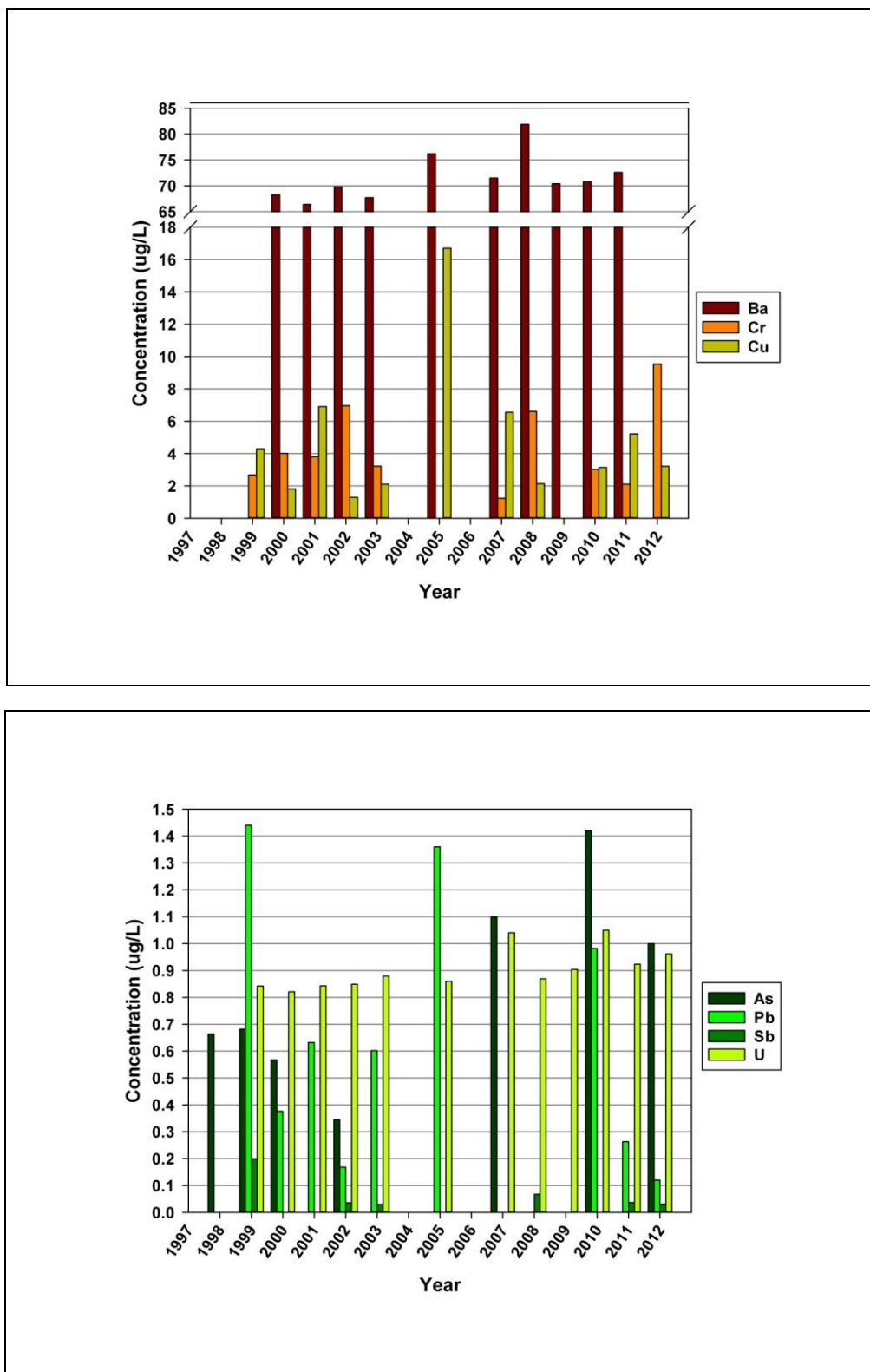
Figure 2.12 Concentrations (µg/L) of Select Inorganic Analytes Measured in Carlsbad Drinking Water from 1998 - 2012
