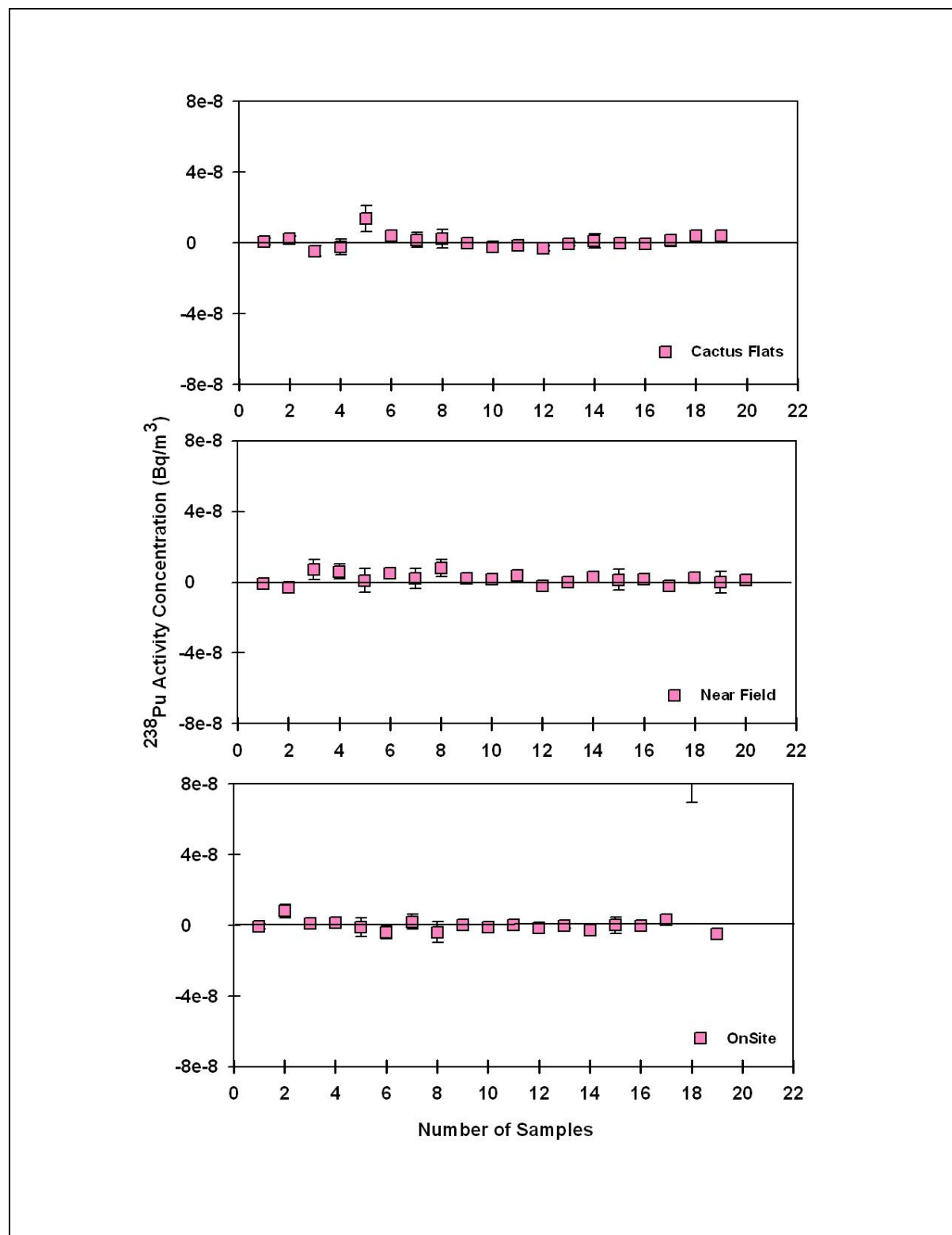
Figure 5.20 238 Pu Concentrations in Aerosol Filters Collected in 2012
