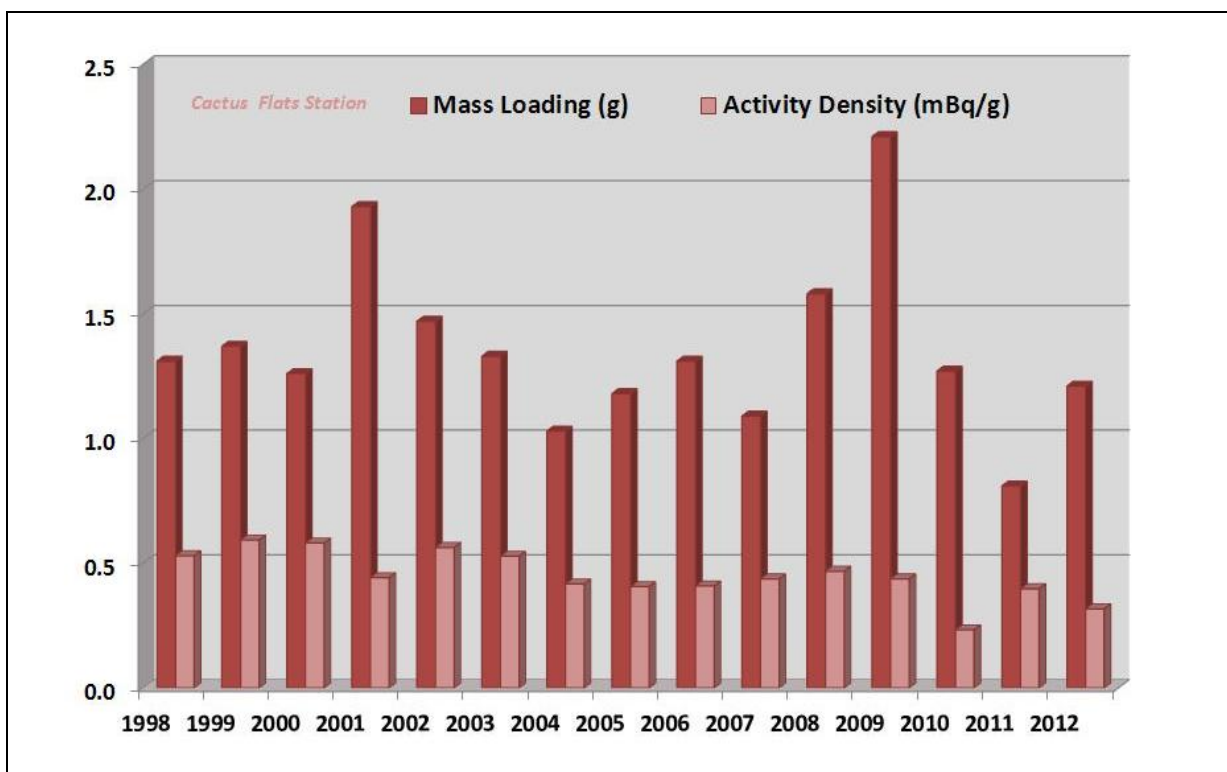
Figure 5.16 Average High Volume Ambient Aerosol Mass Loading and ^{239+240}\text{Pu} Activity Density at Cactus Flats Station
