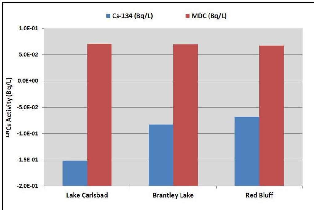
Figure 7.14 ^{134}\text{Cs} activity concentrations in surface water samples in three regional reservoirs
