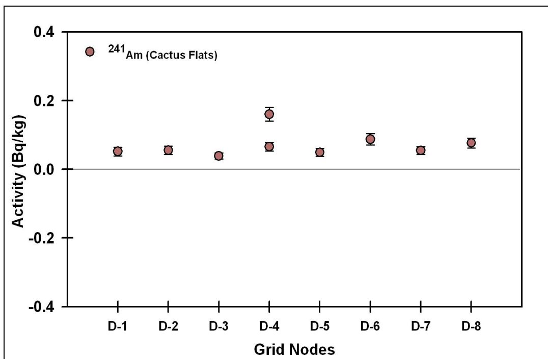
Figure 6.7 Activity Concentrations of ^{241}\text{Am} in Soil Samples Collected from Cactus Flats in 2012
