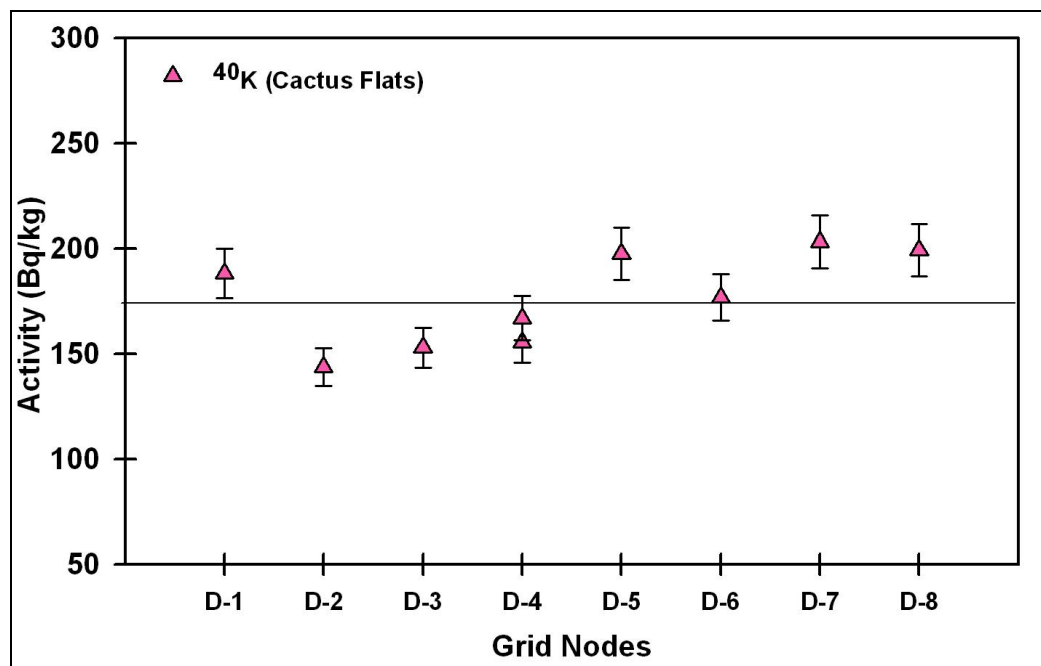
Figure 6.11 Activity Concentrations of ^{40}\text{K} in Soil Samples Collected from Cactus Flats in 2012
