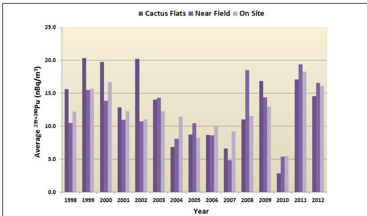
Figure 5.11 Average High Volume Ambient Aerosol ^{239+240}\text{Pu} Activity Concentrations in the Vicinity of WIPP Site
