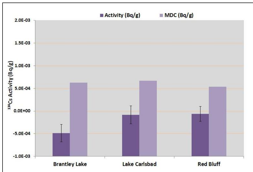
Figure 7.6 ^{134}\text{Cs} activity concentrations in sediment samples in three regional reservoirs
