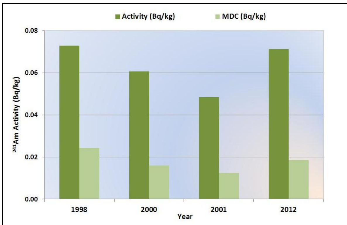
Figure 6.20 Average Activity Concentrations of ^{241}\text{Am} in Cactus Flats (1998-2012)
