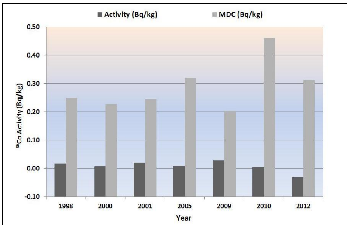
Figure 6.18 Average Activity Concentrations of ^{60}\text{Co} in Near Field Soil (1998-2012)
