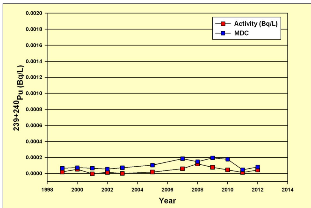
Figure 2.7 ^{239+240}\text{Pu} in Hobbs Drinking Water from 1999-2012
