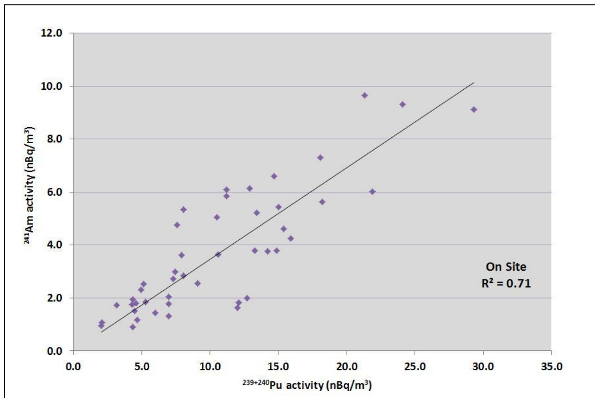
Figure 5.10 Correlation between ^{241}\text{Am} and ^{239+240}\text{Pu} Activity Concentrations in Aerosol Samples Collected from On Site Station
