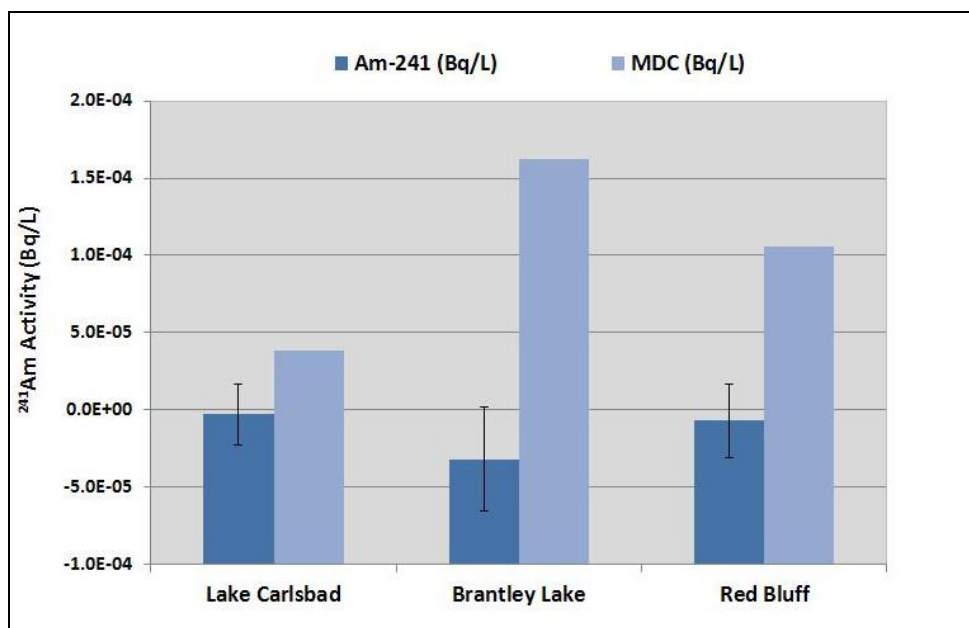
Figure 7.11 ^{241}\text{Am} activity concentrations in surface water samples in three regional reservoirs
