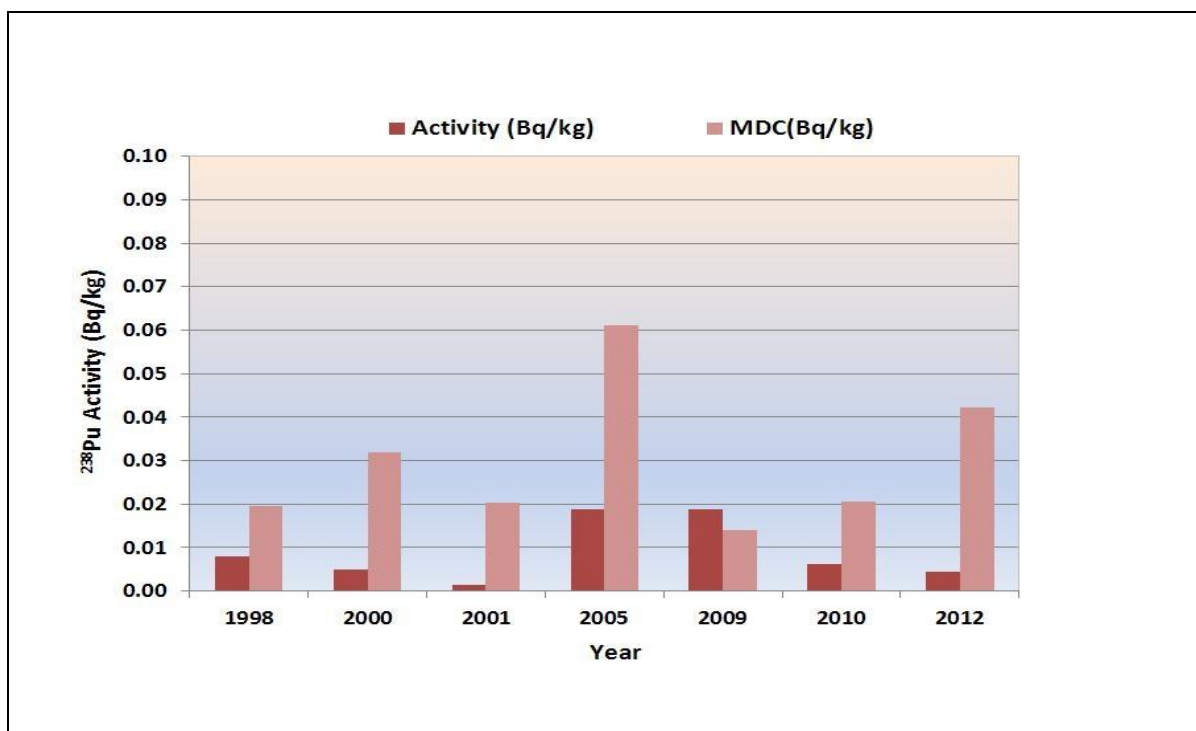
Figure 6.15 Average Activity Concentrations of ^{238}\text{Pu} in Near Field Soil (1998-2012)
