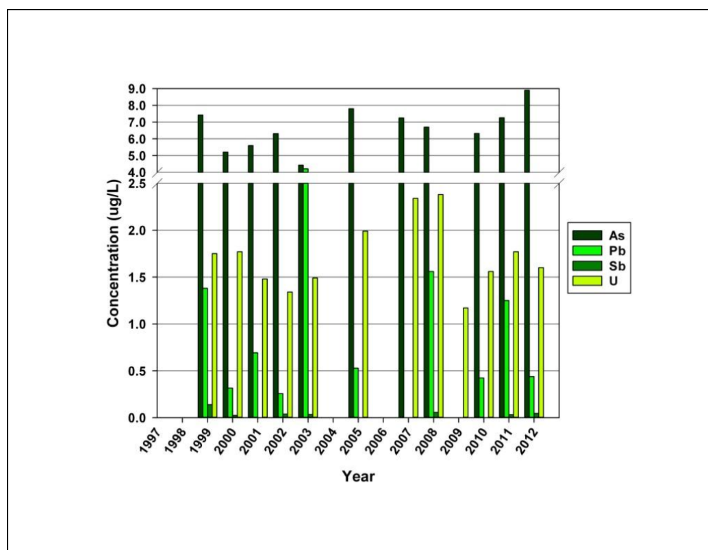
Figure 2.13 Concentrations (µg/L) of Select Inorganic Analytes Measured Near the WIPP site (Double Eagle) from 1998 - 2012
