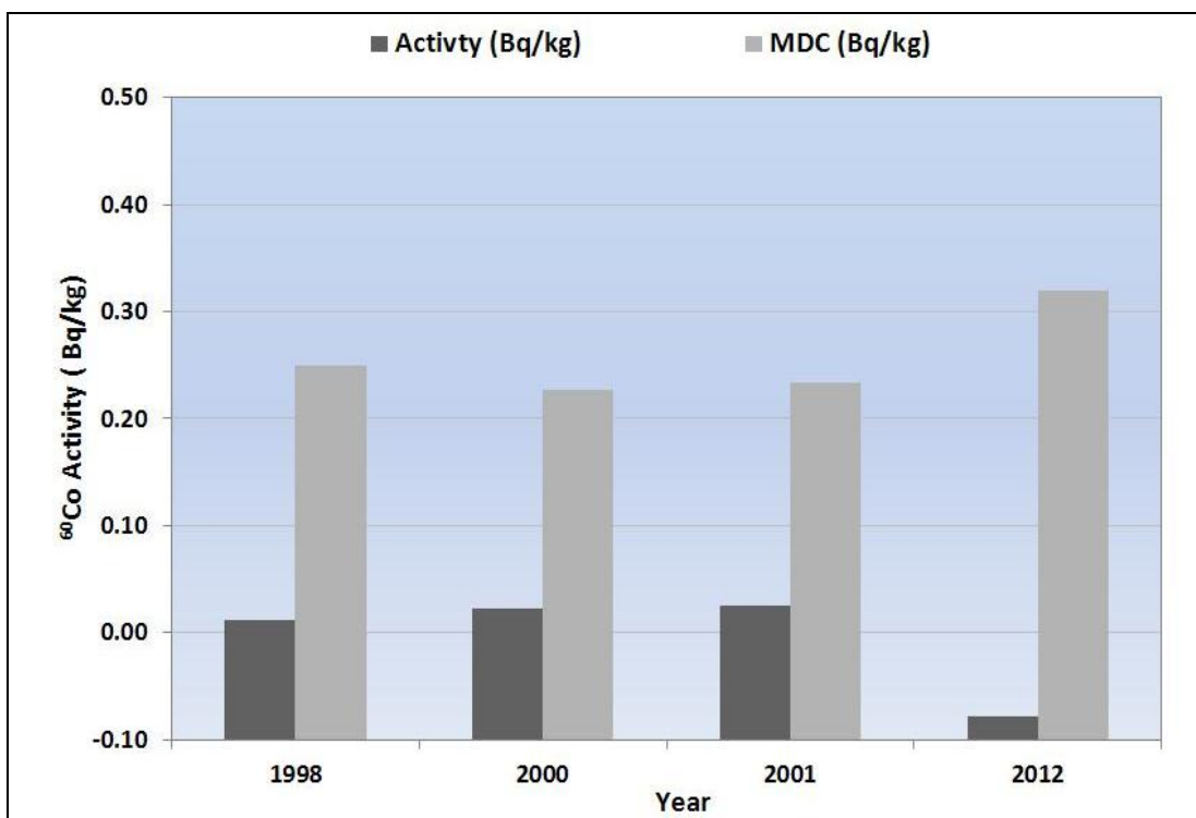
Figure 6.24 Average Activity Concentrations of ^{60}\text{Co} in Cactus Flats (1998-2012)
