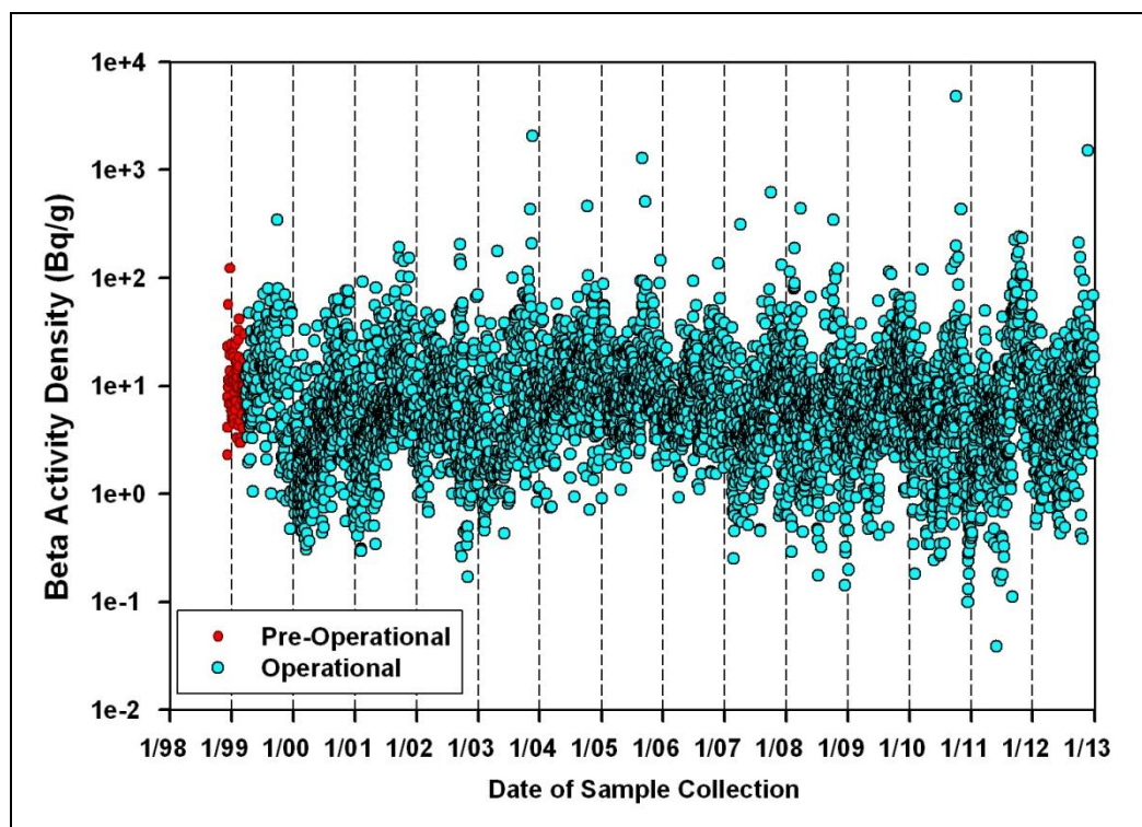
Figure 1.7 Gross Beta Activity Densities measured in Station A Filters
