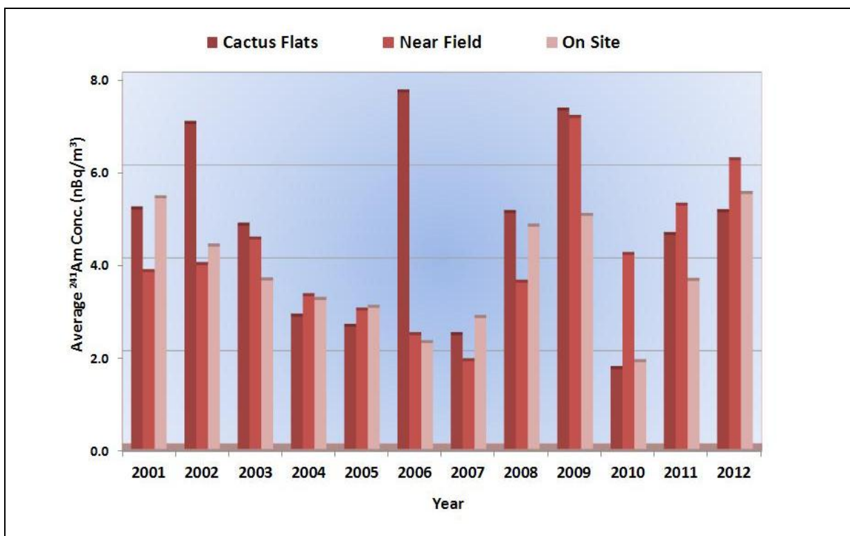
Figure 5.12 Average High Volume Ambient Aerosol ^{241}\text{Am} Activity Concentrations in the Vicinity of the WIPP Site
