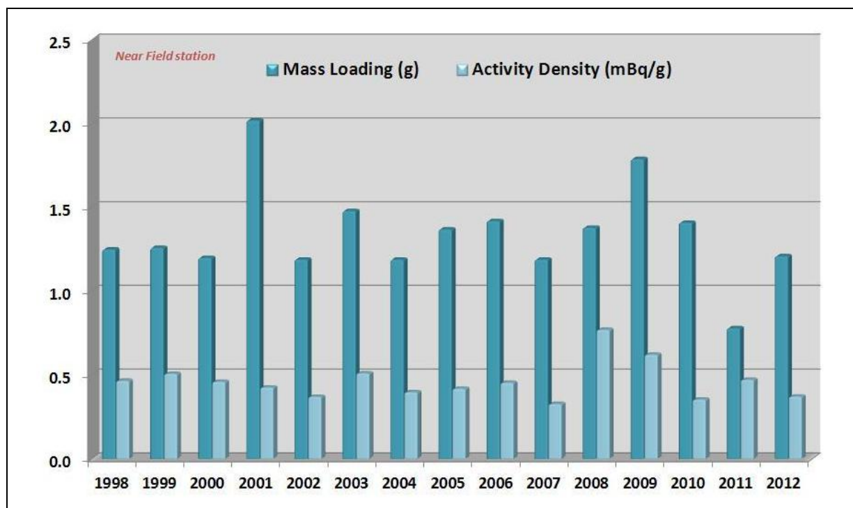
Figure 5.15 Average High Volume Ambient Aerosol Mass Loading and ^{239+240}\text{Pu} Activity Density at Near Field Station
