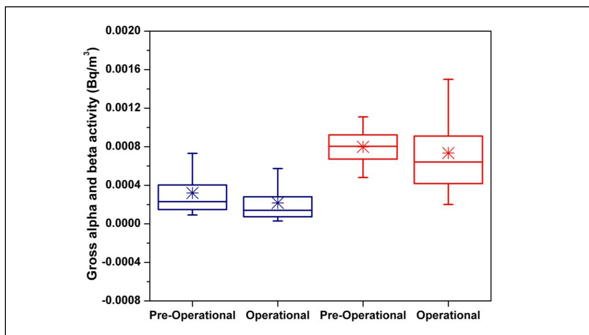
Figure 1.8 Comparison of pre-operational and operational Gross alpha (Navy Box) and beta (red box) activity concentration (Bq/m³) in the Station A filters.
