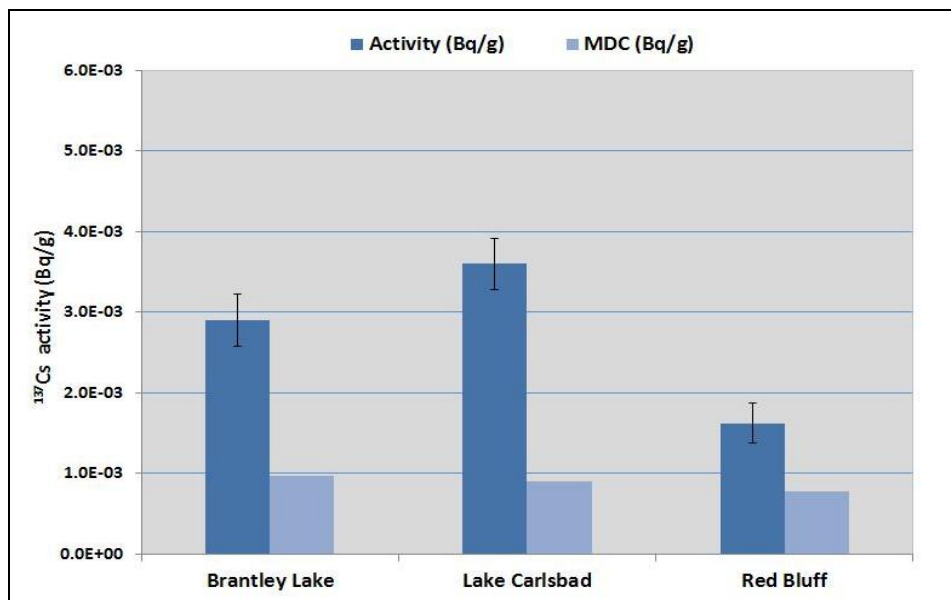
Figure 7.5 ^{137}\text{Cs} activity concentrations in sediment samples in three regional reservoirs
