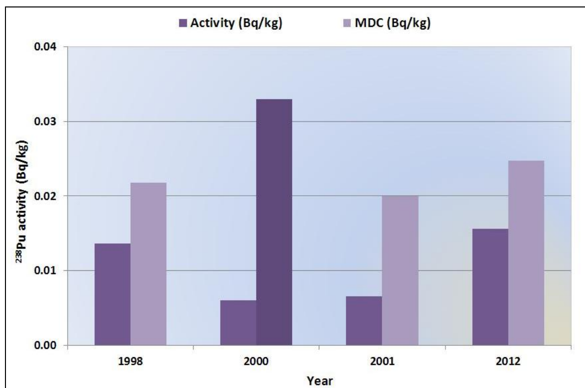
Figure 6.21 Average Activity Concentrations of ^{238}\text{Pu} in Cactus Flats (1998-2012)
