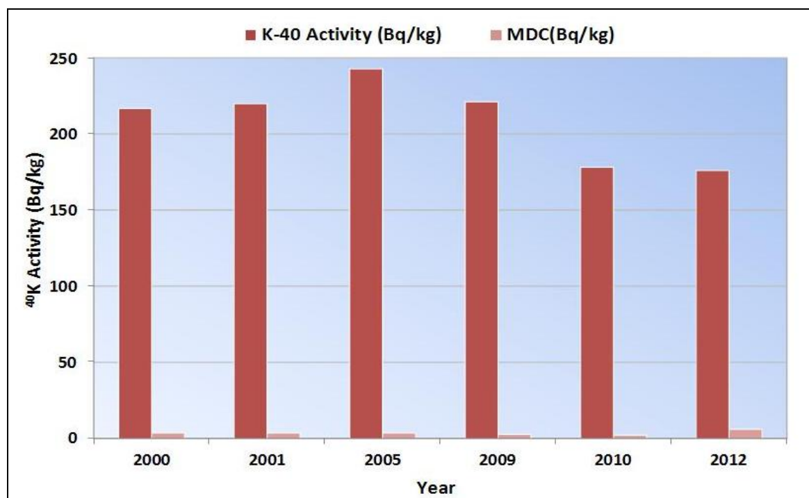
Figure 6.19 Average Activity Concentrations of ^{40}\text{K} in Near Field Soil (1998-2012)
