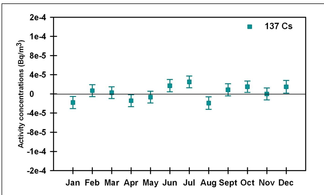
Figure 1.20 ^{137}\text{Cs} Concentrations in Station A Composites in 2012
