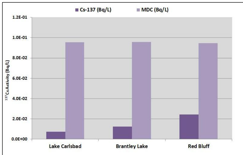
Figure 7.15 ^{137}\text{Cs} activity concentrations in surface water samples in three regional reservoirs
