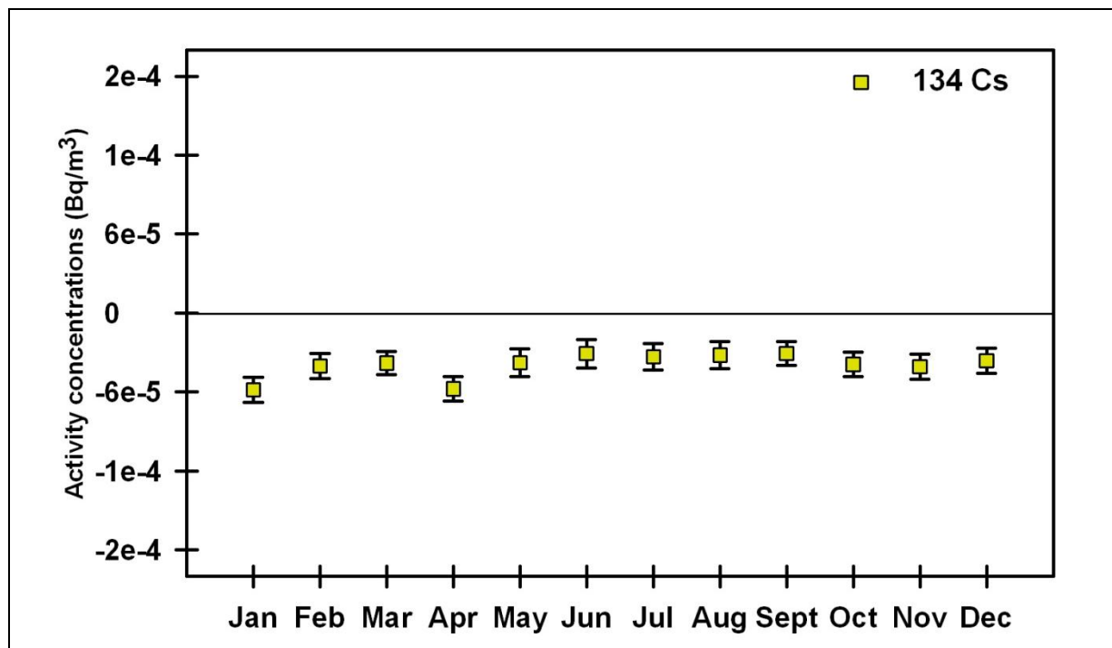
Figure 1.21 ^{134}\text{Cs} Concentrations in Station A Composite in 2012
