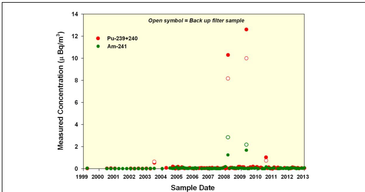
Figure 1.23 Activity Concentrations of ^{239+240}\text{Pu} and ^{241}\text{Am} in Station A filters (1999-2012)
