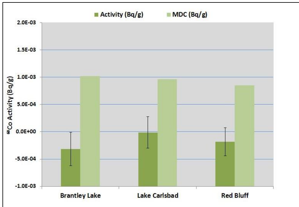
Figure 7.7 ^{60}\text{Co} activity concentrations in sediment samples in three regional reservoirs
