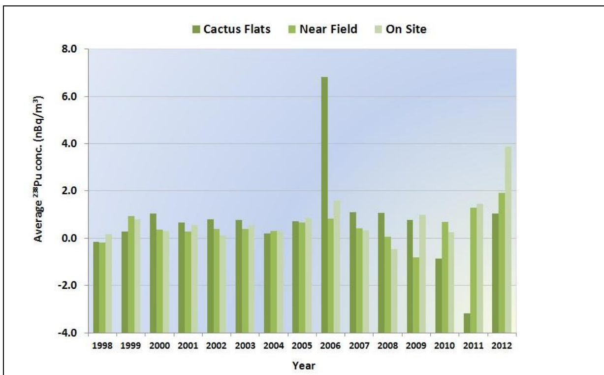
Figure 5.13 Average High Volume Ambient Aerosol ^{238}\text{Pu} Activity Concentrations in the vicinity of the WIPP Site
