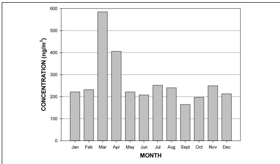
Figure 1.32 Monthly Average Concentrations of AI for 2012
