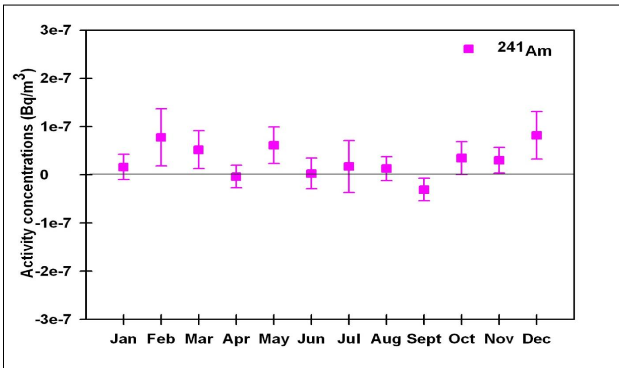
Figure 1.19 ^{241}\text{Am} Concentrations in Station A composites in 2012
