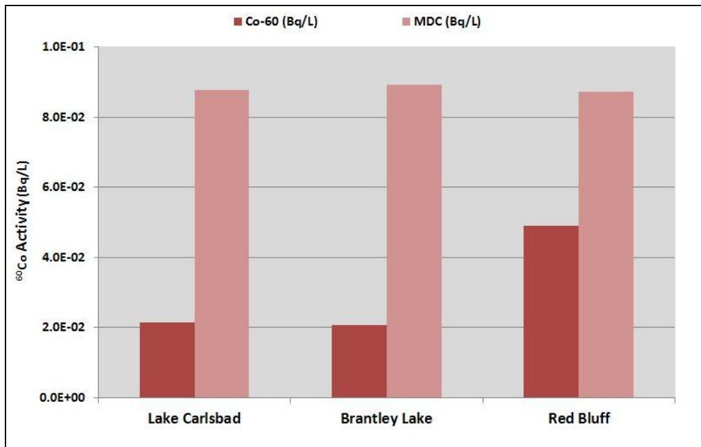
Figure 7.16 ^{60}\text{Co} activity concentrations in surface water samples in three regional reservoirs
