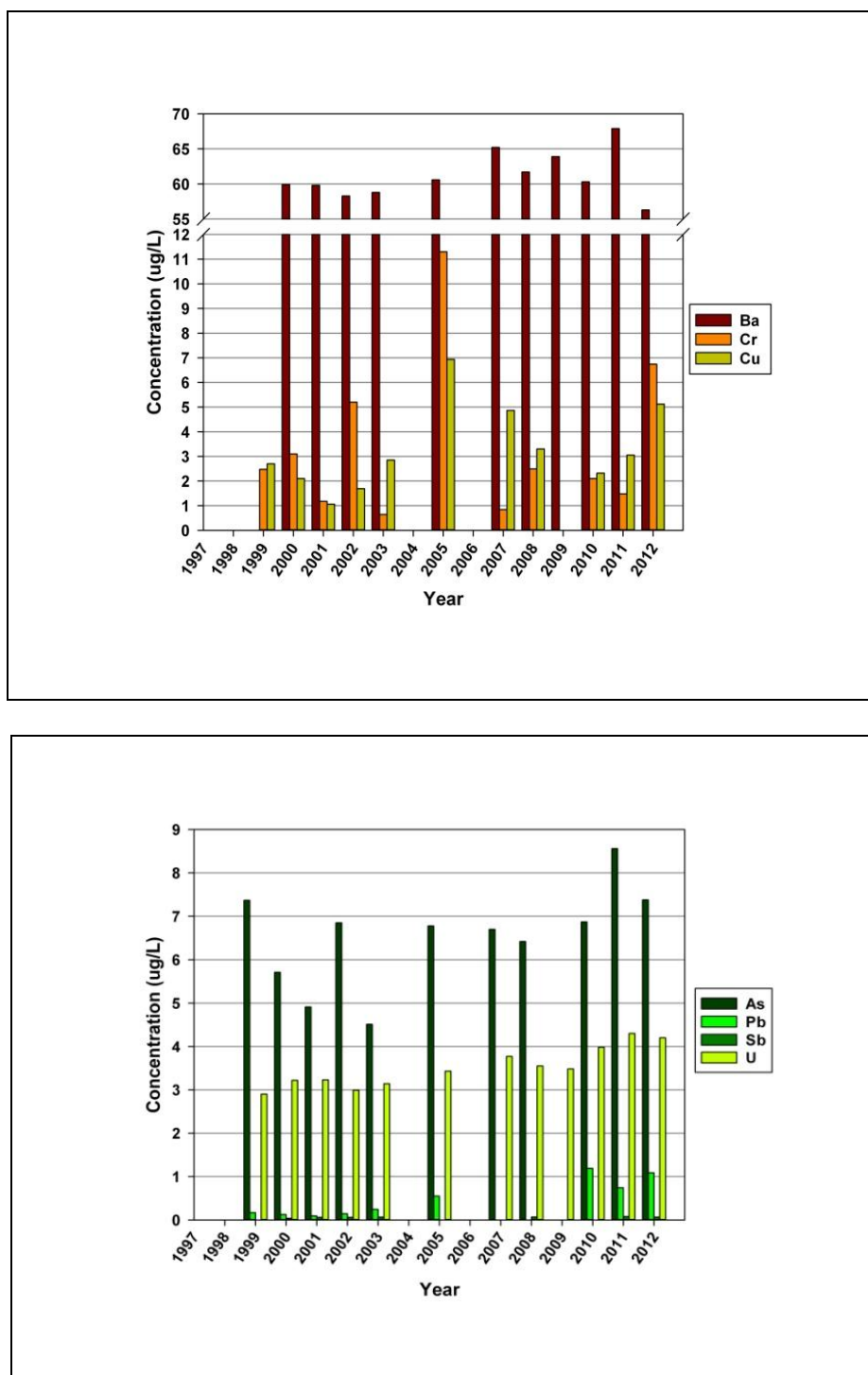
Figure 2.15 Concentrations ( \mu\text{g/L} ) of Select Inorganic Analytes Measured in Hobbs Drinking Water from 1998 - 2012
