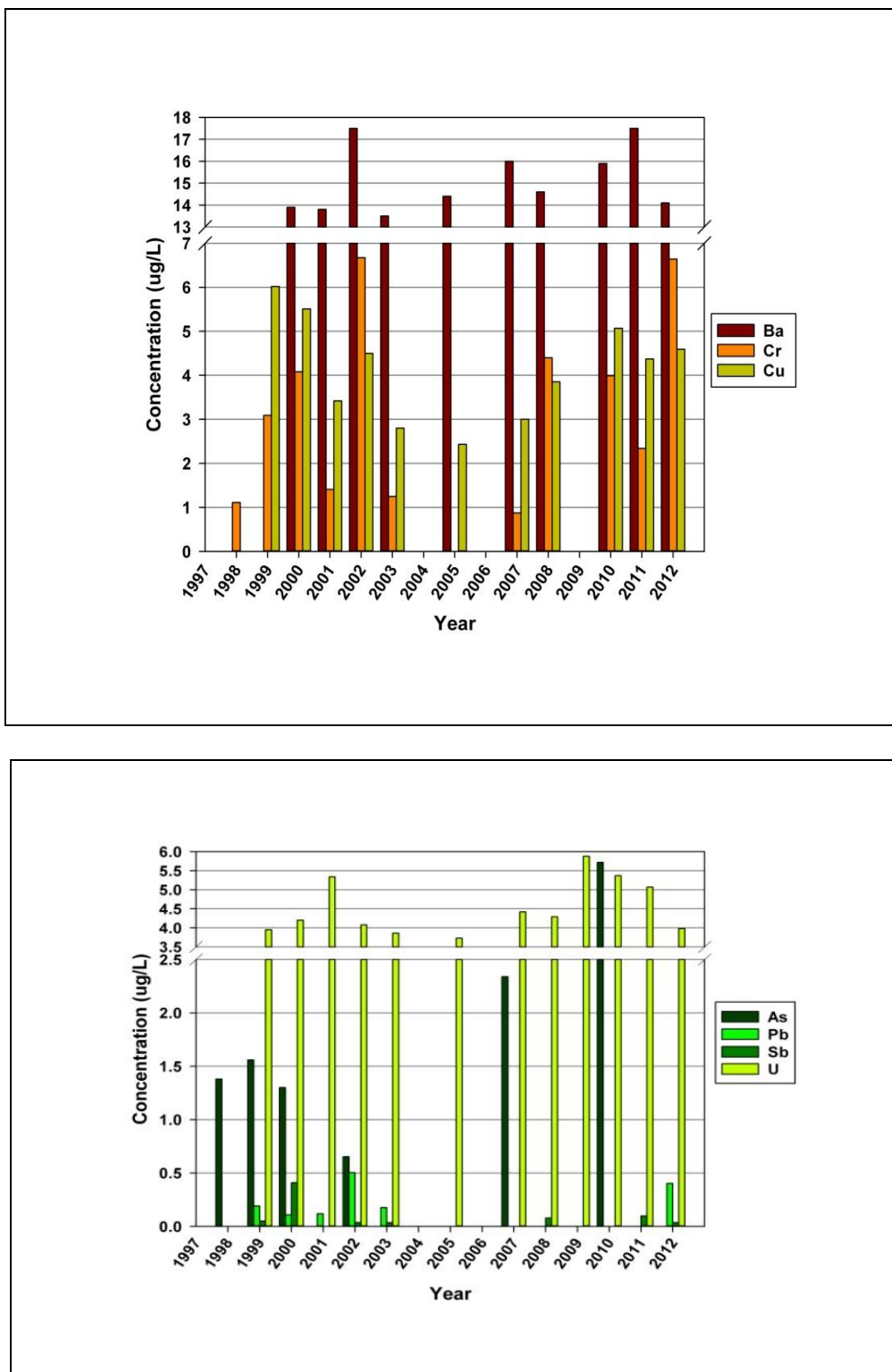
Figure 2.16 Concentrations (µg/L) of Select Inorganic Analytes Measured in Otis Drinking Water from 1998 - 2012
