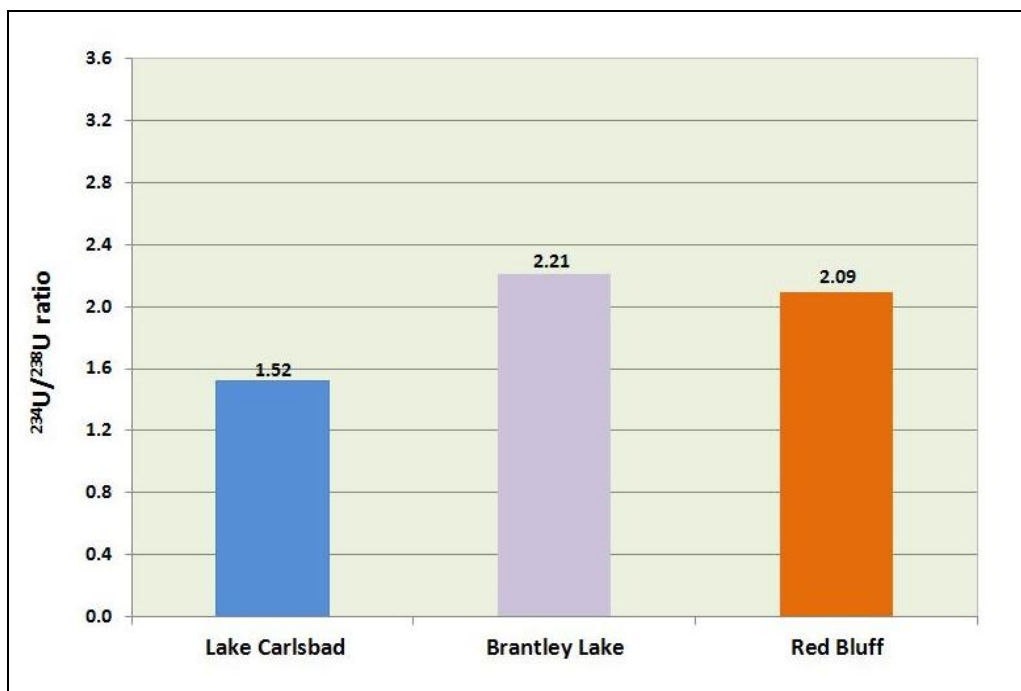
Figure 7.13 The ^{234}\text{U}/^{238}\text{U} Activity Ratio in surface water samples of three reservoirs in the vicinity of the WIPP site
