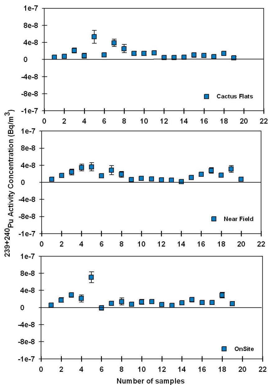
Figure 5.19 ^{239+240}\text{Pu} Concentrations in Aerosol Filters Collected in 2012
