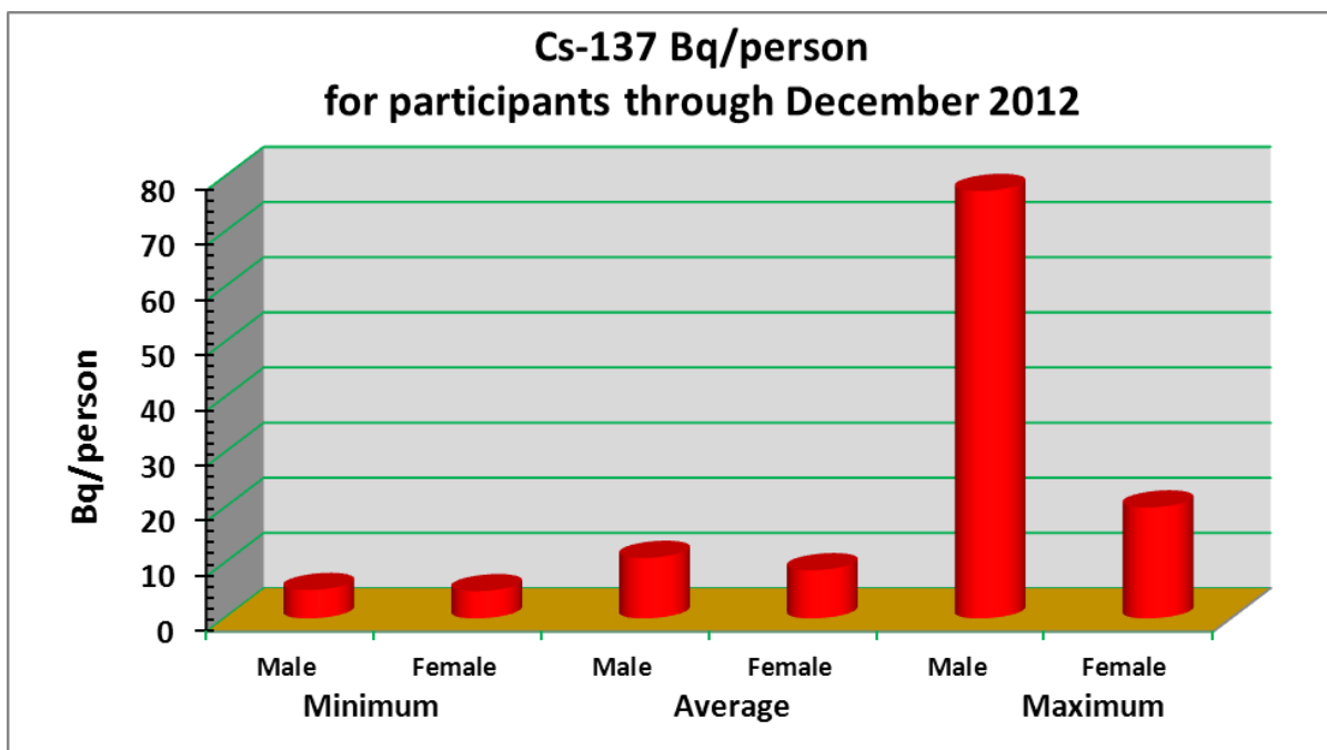
Figure 3.5 Minimum, average, and maximum ^{137}\text{Cs} activity for participants, separated by gender, through December 2012
