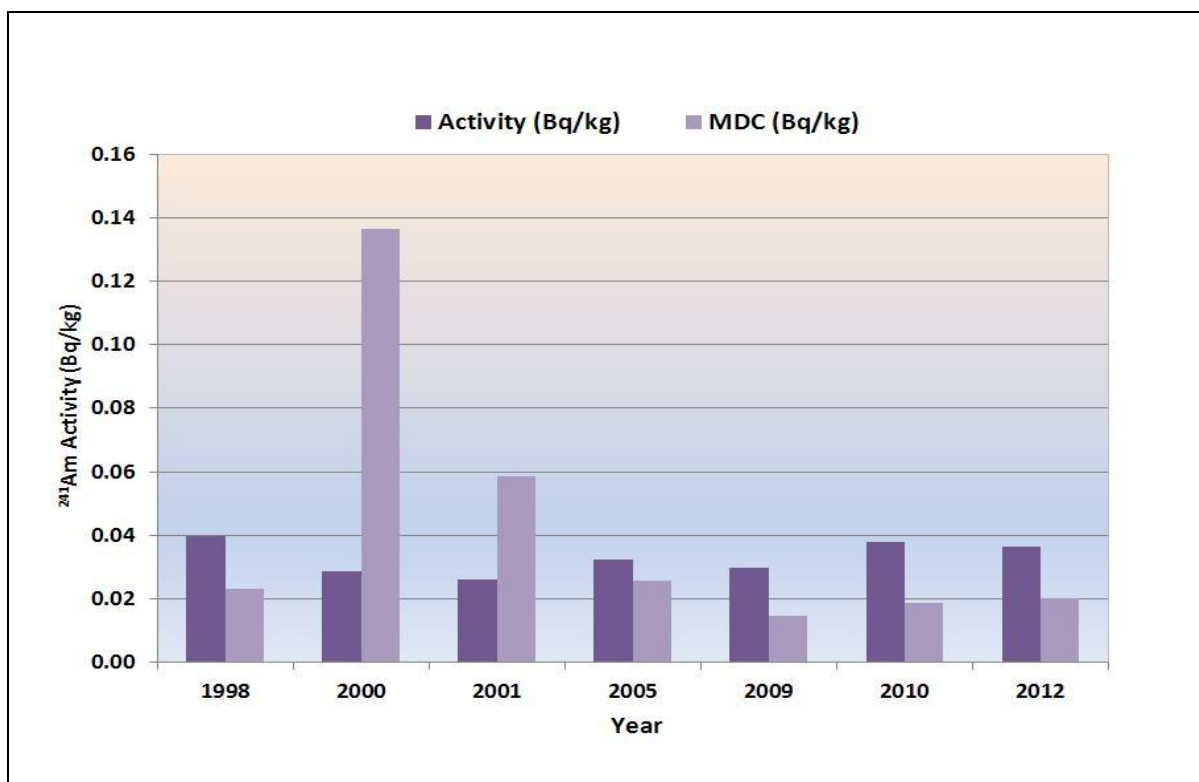
Figure 6.16 Average Activity Concentrations of ^{241}\text{Am} in Near Field Soil (1998-2012)
