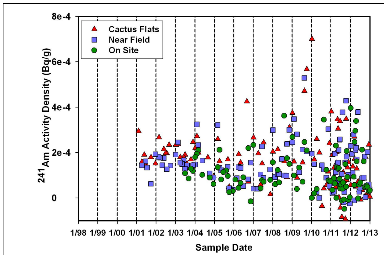
Figure 5.7 High Volume Ambient Aerosol ^{241}\text{Am} Activity Densities
