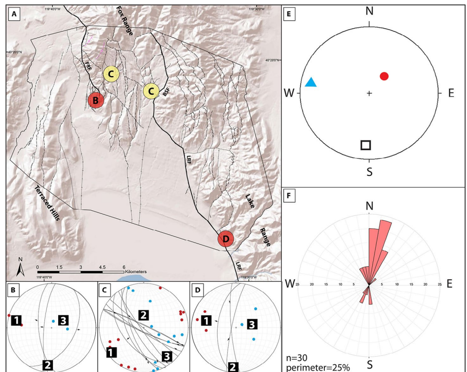
Figure 2. A) Locations where kinematic data were collected. Circles with letters correspond with the kinematic plots below. B-D) Lower hemisphere, equal area stereographic projections of fault planes and strain axes (T-axes=red dots, P-axes=blue dots), and mean principal strain axes (black squares; 1=maximum, 2=intermediate, 3=minimum). B) Strain axes derived from fault slip data from a splay of the Fox Range fault. C) Strain axes derived from fault slip data from within the step-over. D) Strain axes derived from fault slip data from the Lake Range. E) Lower hemisphere, equal area stereographic projection of the principle axes of stress derived from inversion of the spatially sorted data (Blue triangle=minimum stress, red circle=maximum stress, open square=intermediate stress). F) Rose diagram of the strike of vein orientations that cut Miocene volcanic rocks and Quaternary indurated sediments. Radius equals 25% of the data.
