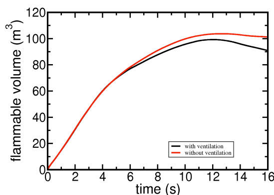
Figure 12. Simulation results showing time evolution of flammable volume of hydrogen (4% - 75% mole fraction) from forklift release of 0.8 kg \text{H}_2 in the full-scale warehouse for cases with and without forced ventilation.
