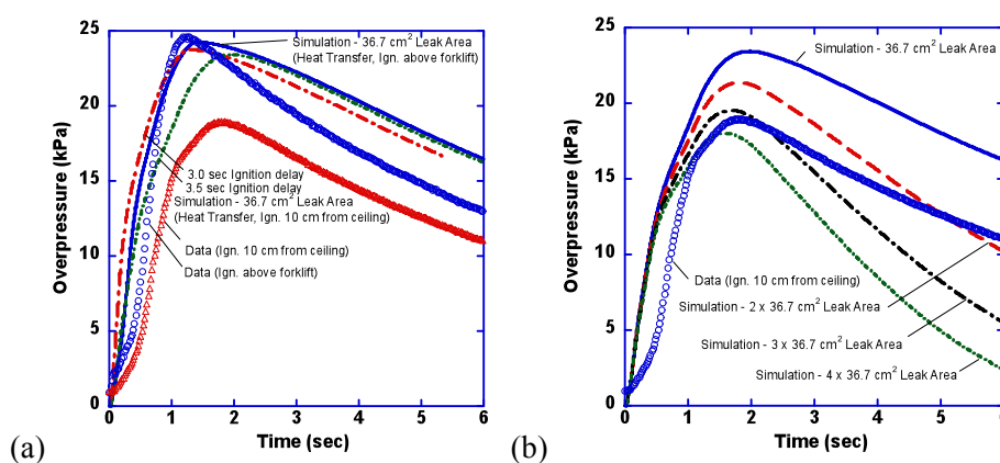
Figure 11. (a) Comparison of simulation results and experimental data for ignition 3 cm above forklift (3.0 sec ignition delay time) and ignition 10 cm from warehouse ceiling (3.0 and 3.5 sec ignition delay time). (b) Comparison of simulation results with experimental data for ignition 10 cm from warehouse ceiling (3.5 sec ignition delay time) where the amount of warehouse leakage was varied in the simulations.
