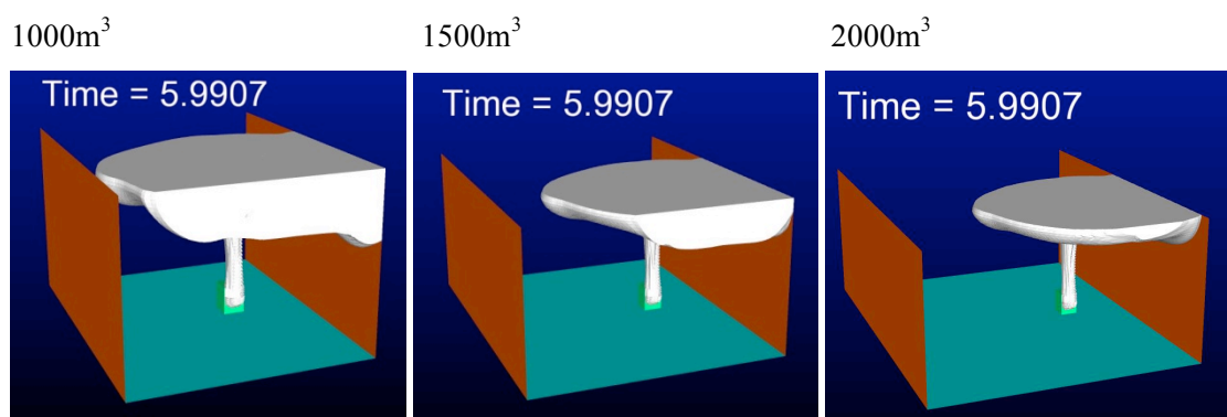
Figure 14. Simulations showing flammable hydrogen cloud (4% - 75% mole fraction) 6 sec into the 0.8 kg forklift release for full-scale warehouses with a 7.62 m high ceiling and volumes of 1000 m 3 , 1500 m 3 , and 2000 m 3 (without ventilation).
