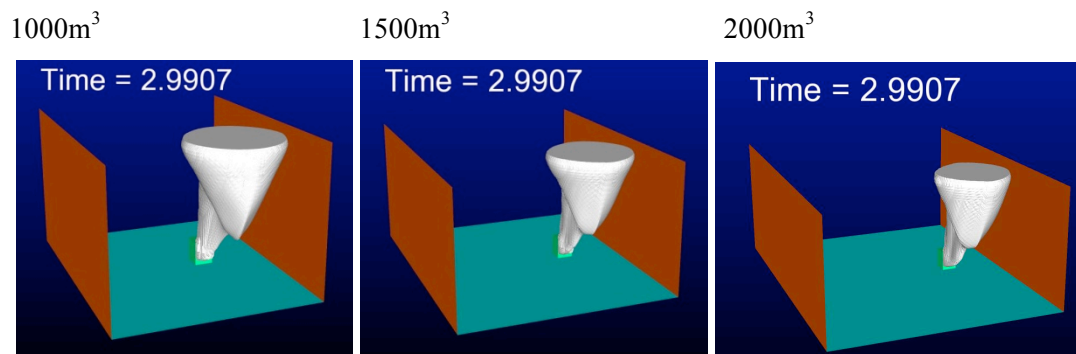
Figure 13. Simulations showing flammable hydrogen cloud (4% - 75% mole fraction) 3 sec into the 0.8 kg forklift release for full-scale warehouses with a 7.62 m high ceiling and volumes of 1000 m 3 , 1500 m 3 , and 2000 m 3 (without ventilation).
