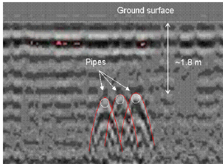
Figure 7: Ground Penetrating Radar (GPR) image of pipes underneath roadway [19].
