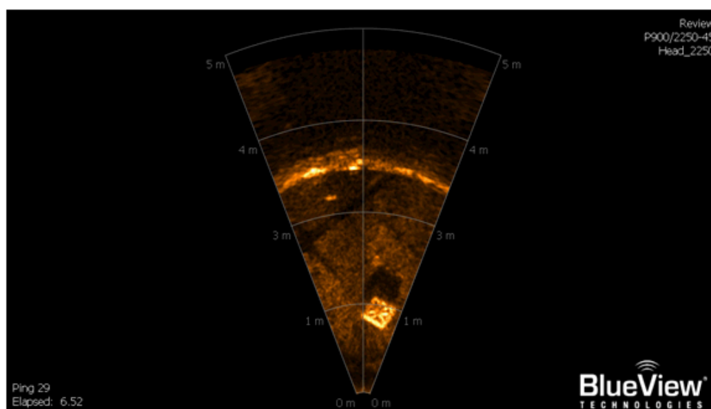
Figure 8: 2D sonar imaging using 2250 kHz sound pulses [20].
