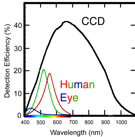
Figure 2: Human eye versus Charge Coupled Devices (CCD) commonly found in digital cameras [4].
