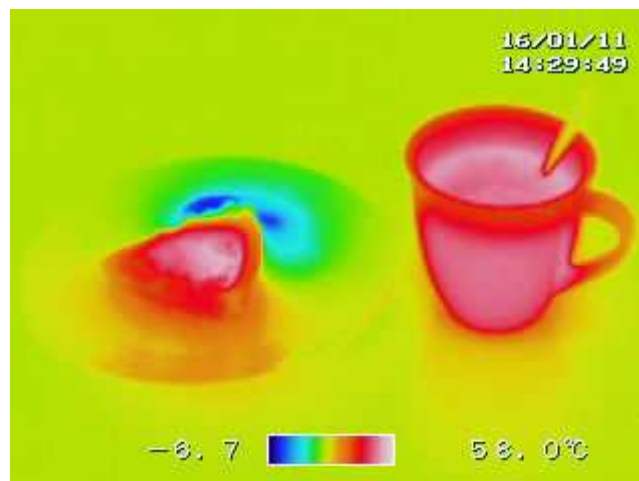
Figure 6: Coffee and apple pie image in the LWIR, using an uncooled detector (microbolometer) commercial thermal imager (Photo courtesy of Pieter Kuiper using an NEC Thermo Shot camera).
