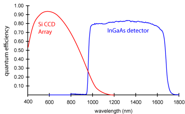
Figure 3: Quantum efficiency (sensitivity) of a silicon detector (CCD) versus InGaAs detector [5].
