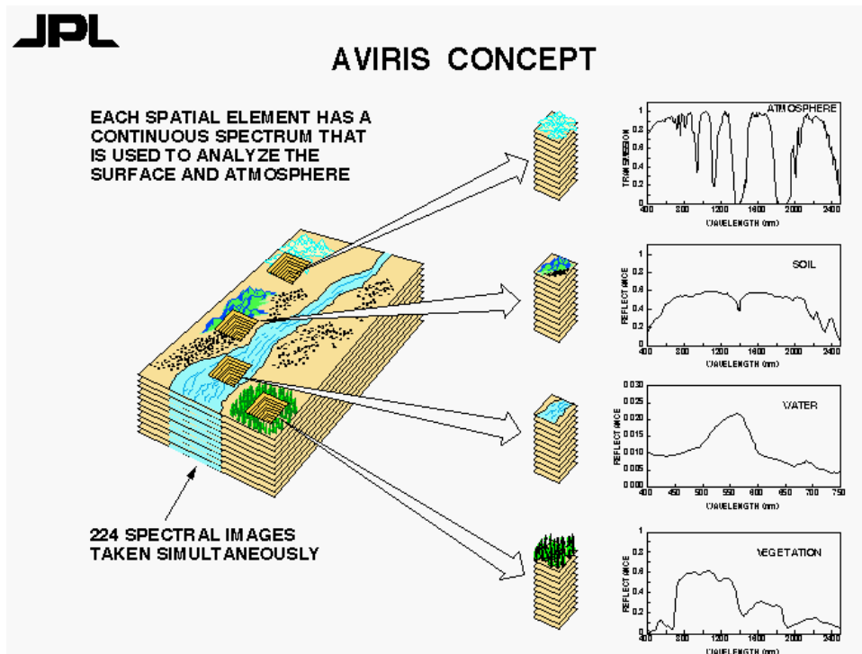
Figure 9: Imaging spectroscopy, or hyperspectral imaging, allows stand-off material analysis. This conceptual figure appears at [22].
