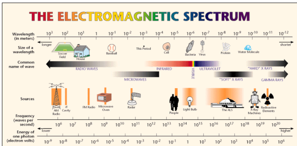
Figure 1: The electromagnetic spectrum (Courtesy: Remote Sensing Tutorial [3]).
