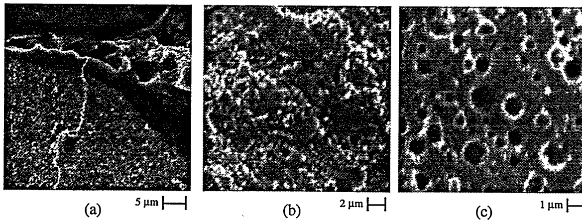
Figure 6. SEM micrographs of irradiated RERTR-2 microplate A005 (U-10Mo) at 69% burnup.
