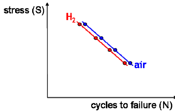
Figure 5. Schematic of the cyclic stress amplitude ( S ) vs number of cycles to failure ( N ) plots measured in hydrogen gas and in air. These S - N data points are typically plotted on linear-log axes, since N changes by orders of magnitude.
