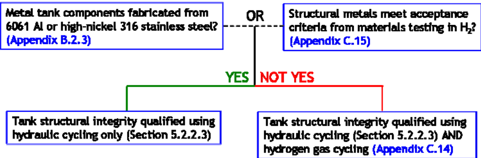
Figure 3. Logic diagram for addressing hydrogen embrittlement in the SAE J2579.
