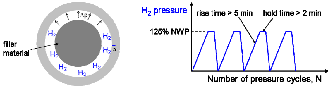
Figure 7. Schematic of hydrogen embrittlement performance test procedures.
