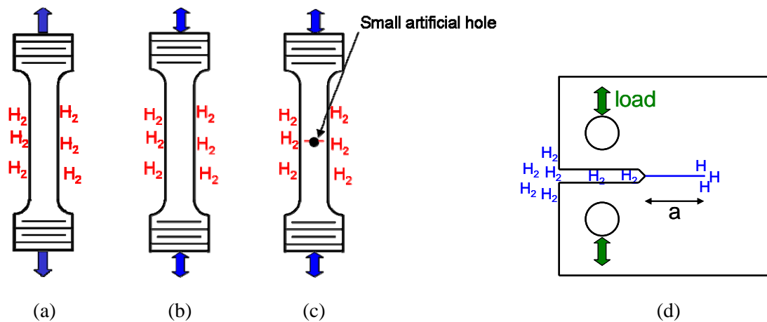
Figure 4. Schematics of materials test specimens in Appendix C.15 of SAE J2579. The slow strain rate specimen (a) is subjected to monotonic loading, while the fatigue life specimens (b) and (c) as well as the fatigue crack growth rate specimen (d) are tested under cyclic loading.
