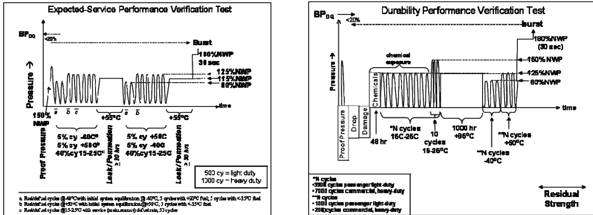
Figure 2. Schematics showing protocols for the expected service performance test (pneumatic) and the durability performance test (hydraulic).
