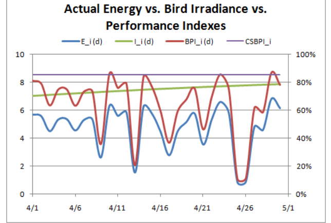
Figure 2: For sample system i , compare (a) daily energy vs. clear sky daily insolation, and (b) BPI vs. clear sky BPI.
