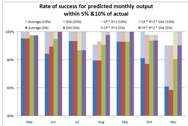
Figure 6: Rates of successfully predicted monthly output within 5% (dark colors) and 10% (light colors) of actual generation. The Conversion Profile and the R^2 values were calculated from daily energy data measured during the preceding month.
