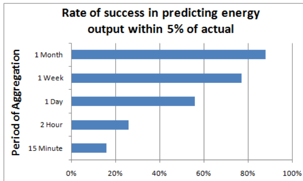
Figure 3: Rate of success in predicting energy output given by the arithmetic mean of N-1 energy estimates. Results based on 15-minute measurements and compared over 7 months (May-November 2010).
