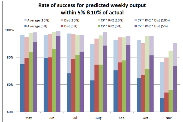
Figure 5: Rates of successfully predicted weekly output within 5% (dark colors) and 10% (light colors) of actual generation. The Conversion Profile and the R^2 values were calculated from daily energy data measured during the preceding month.
