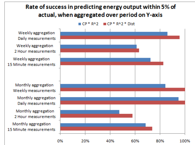
Figure 4: Rate of success in predicting weekly and monthly energy output during June 2010 with two different methods. The R^2 coefficients were calculated based on the intervals noted (15-min, 2-hour, 1-day, 1-week) for the period of May 2010.
