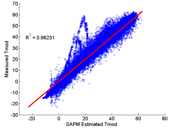
Figure 8: Measured module temperature vs. component-model estimate with 1:1 line
