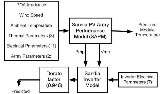
Figure 2: Data flow for component-based model
