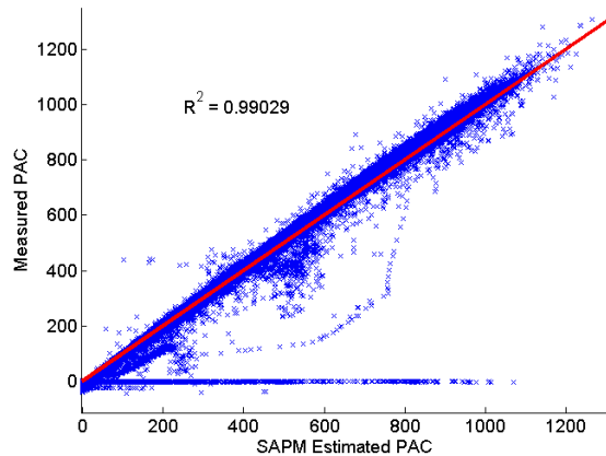
Figure 7: Measured AC power vs. component-model estimated AC power with 1:1 line
