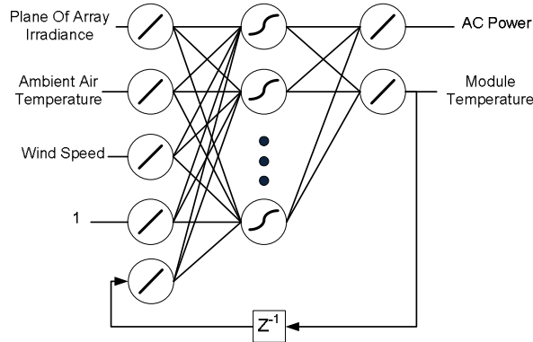
Figure 1: Recurrent neural network used
