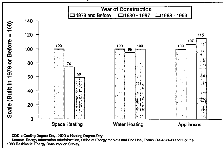
Natural Gas Consumption Figure 3.10. Natural Gas End-Use Intensities by Year of Construction, 1993
