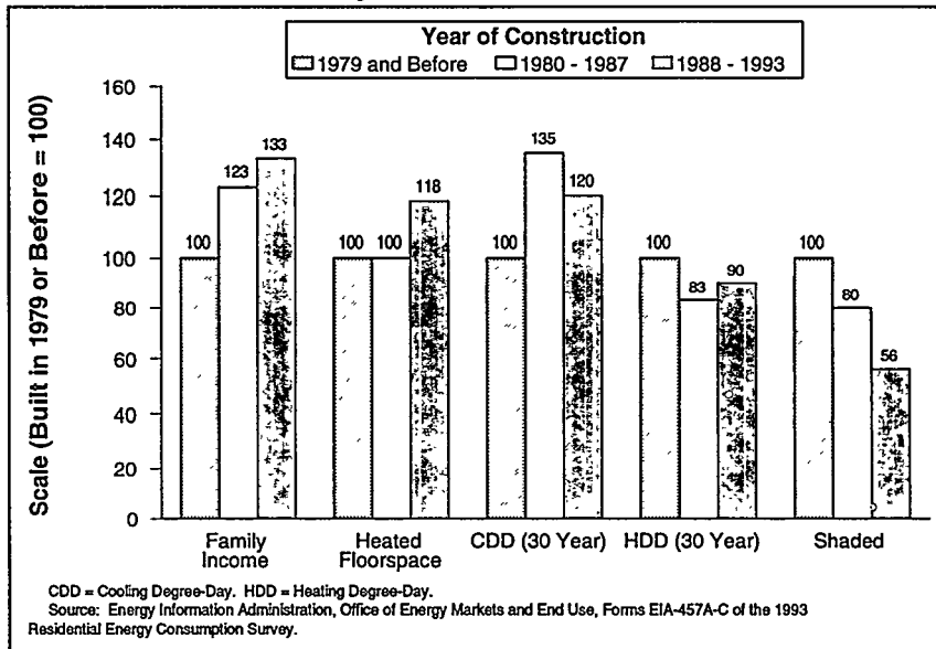
Figure 3.9. Indices for Impact of Climate, Shading, Floorspace, and Income by Year of Construction, 1993
