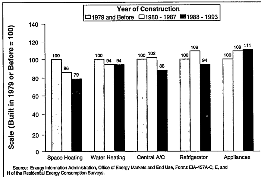
Figure 3.8. End-Use Electricity Intensities By Year of Construction, 1993
