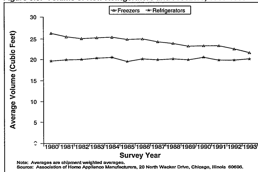
Figure 3.3. Volume of New Refrigerators and Freezers, 1980-1993
