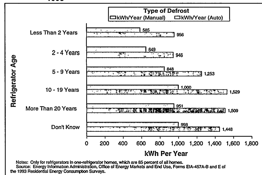
Figure 3.4. Energy Use of Refrigerators by Age and Defrost Type, 1993
