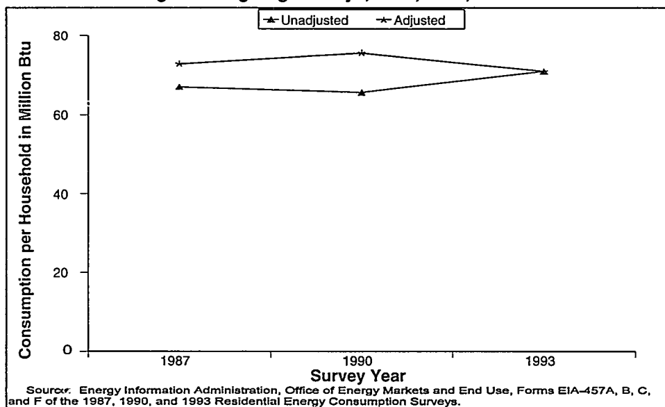
Figure 2.2. Natural Gas Space-Heating Consumption Adjusted for 30-Year Average Heating Degree-Days, 1987, 1990, and 1993
