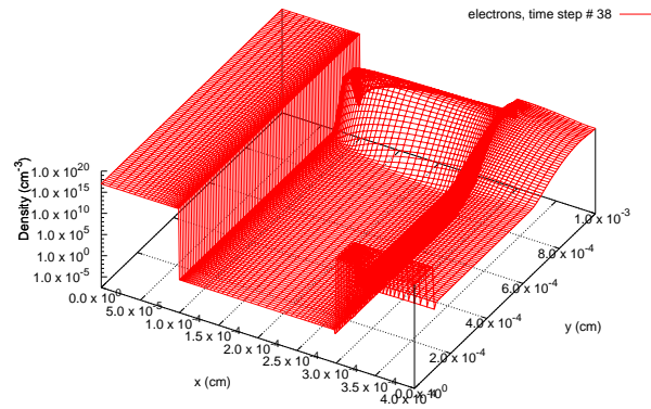
Figure 5. Shows the electron density at a later time. In this case, the space-charge limited current in the rutile region is very prominent.
