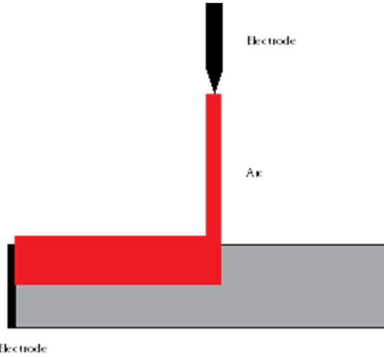
Figure 2. Schematic showing electrical breakdown involving a gas and a solid dielectric. At short times, the high permittivity of the dielectric makes the insulator conductive. The consequent gas breakdown produces a conductive filament. At later times, the space-charge limited current flows in the solid dielectric. At very long times, the Joule heating causes thermal breakdown along the surface.
