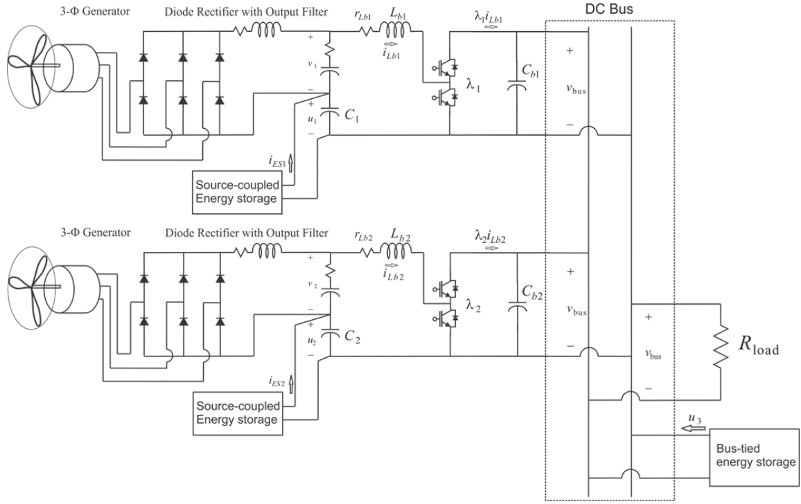
Figure 2: Schematic of example microgrid
