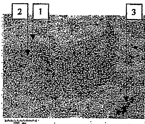
Figure 3. Irradiated \text{U}_3\text{Si}_2 Microphotograph. Miniplate RA321.
