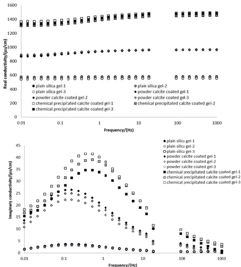
Figure 20: Influence of calcium carbonate coatings on the imaginary conductivity response of the silica gel. Note the influence of the source of the calcium carbonate coatings and the larger range of scale compared to Figure 1. Three replicate measurements from independent repacked columns are shown for each treatment.
