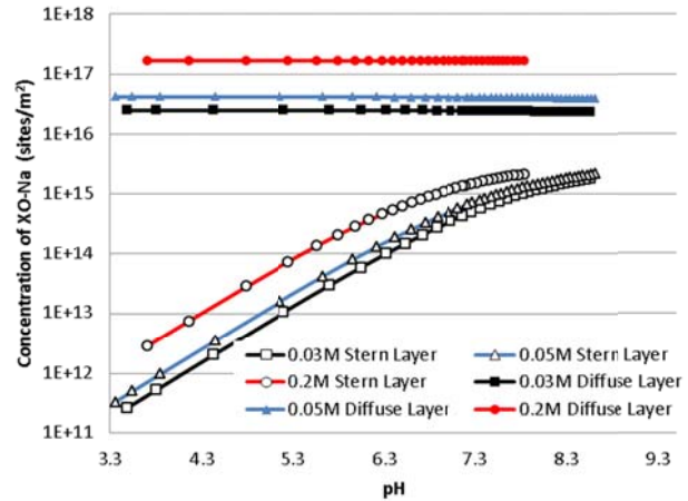
Figure 12: Surface site density as a function of pH for the Stern and diffuse layers based on fitting the triple layer model with the acid-base titration data using Fiteql.
