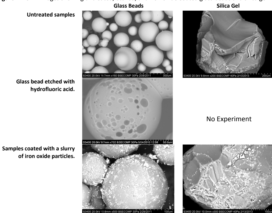
Figure 14: SEM images showing untreated, etched, and iron oxide coated glass beads and silica gel.
