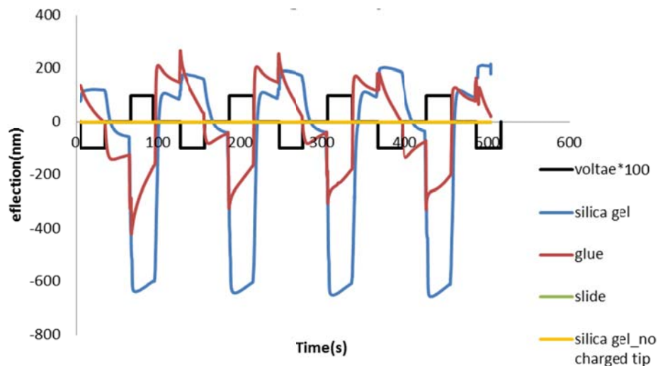
Figure 34: AFM tip deflection response observed in response to an applied voltage (black; actual value multiplied by 100 for scale) for silica gel (blue), background measurements on glue used to attach the silica gel to the sample holder (red). Control measurements on glass and when the AFM tip has no fixed charge show no response (green and yellow, respectively). Response shown is the average of 3 measurements.
