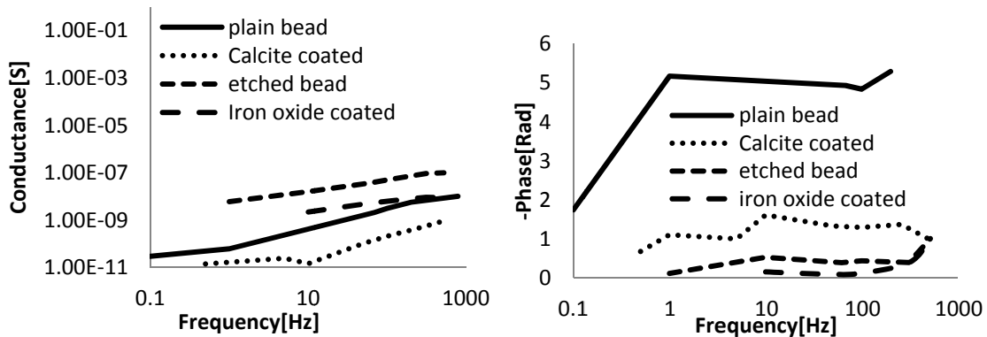
Figure 32: Comparison of conductance and phase measured for different glass bead treatments.
