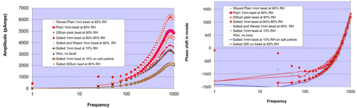
Figure 31: Amplitude and phase response measured for a variety of test scenarios and varying relative humidity.
