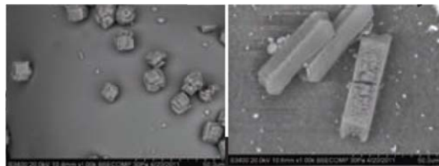
Figure 24: SEM images comparing calcium carbonate crystals formed during abiotic (left) and biologically mediated (right) precipitation.
