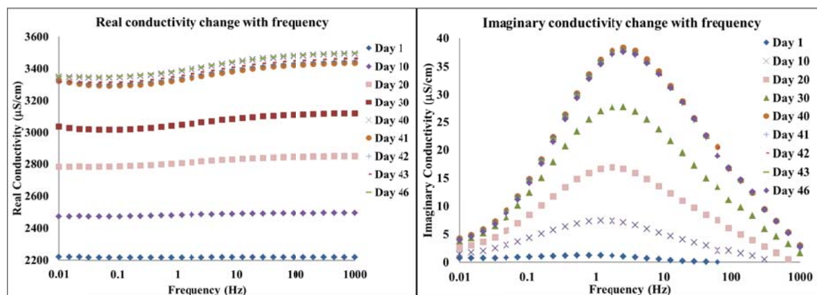
Figure 6: Real (left) and imaginary (right) conductivity measured as function of time during experiment SG2b, where the pH was increased from 7 to 10 over the course of 46 days.
