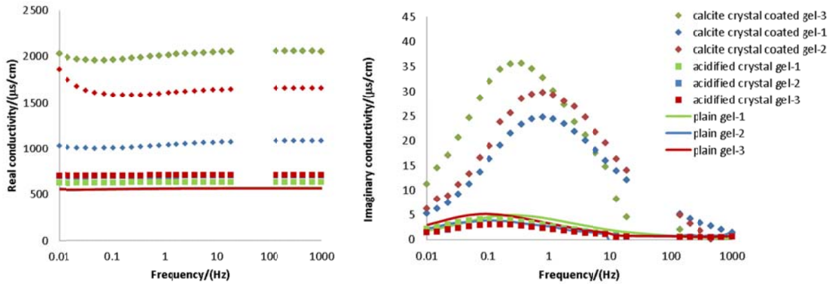
Figure 21: Complex conductivity of silica gel with a layer of calcium carbonate precipitate. After acidifying the sample, the response returns to similar values measured for control conditions.
