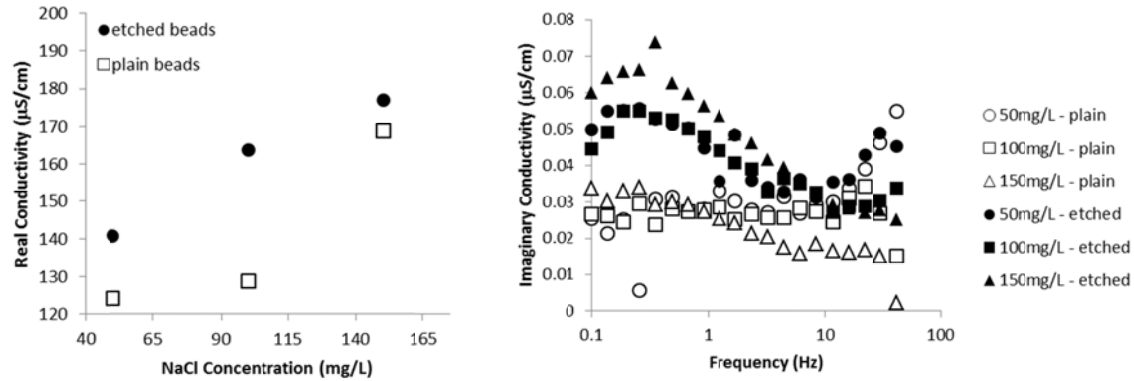
Figure 16: Initial experiments comparing etched glass beads to a control sample under different NaCl solution concentrations. The sample was prepared using dry packing methods. (Exp GB2a)
