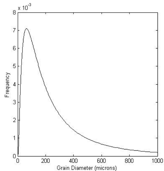
Figure 10: Grain (pore) size distribution of silica gel estimated from inversion of the SIP data.
