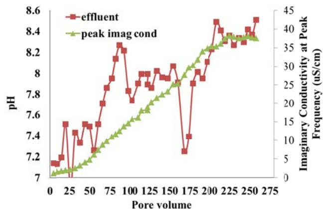
Figure 7: Correlation between changes in the pH of the column effluent and the maximum value of the measured imaginary conductivity spectrum over the course of experiment SG2b.
