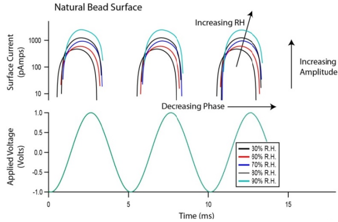
Figure 29: Example time-domain data illustrating the applied voltage and current response using CFM. The approach was successfully applied to measure changes in conductivity associated with successively increasing the thickness of water on a grain surface by manipulating relative humidity.
