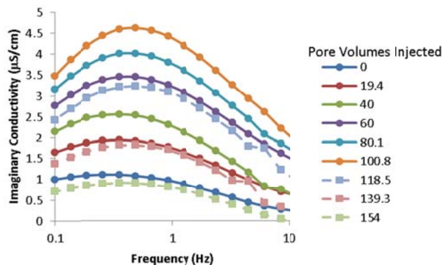
Figure 8: Evaluation of reversibility of pH influence on surface sorption (Exp SG2c). The magnitude of the imaginary conductivity spectrum increases and then decreases as the pH of the influent solution is similarly modified. A qualitative correlation is observed between the change in imaginary conductivity and effluent pH suggesting a close degree of control between pH and the imaginary conductivity response, likely through changes in the number of deprotonated silanol sites on the surface.
