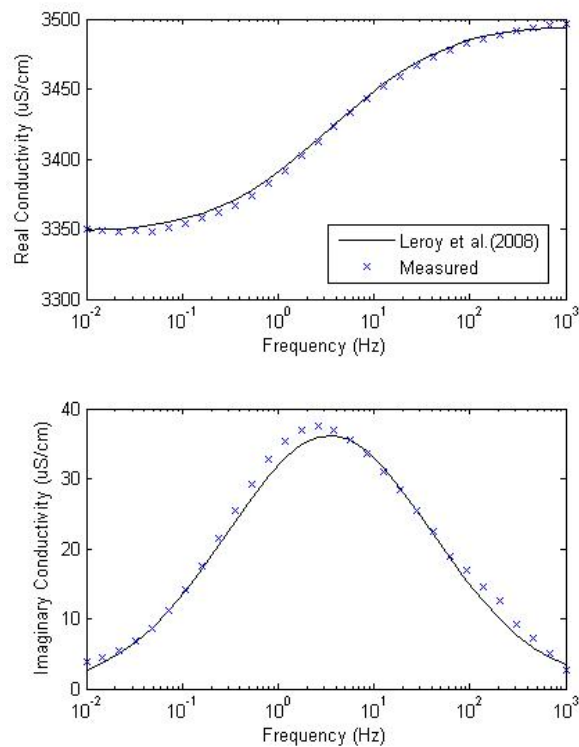
Figure 9: Example of initial fitting of SIP data by the Leroy et al. (2008) model. The data shown are from the final measurement in Experiment SG2b (pH=8.6).
