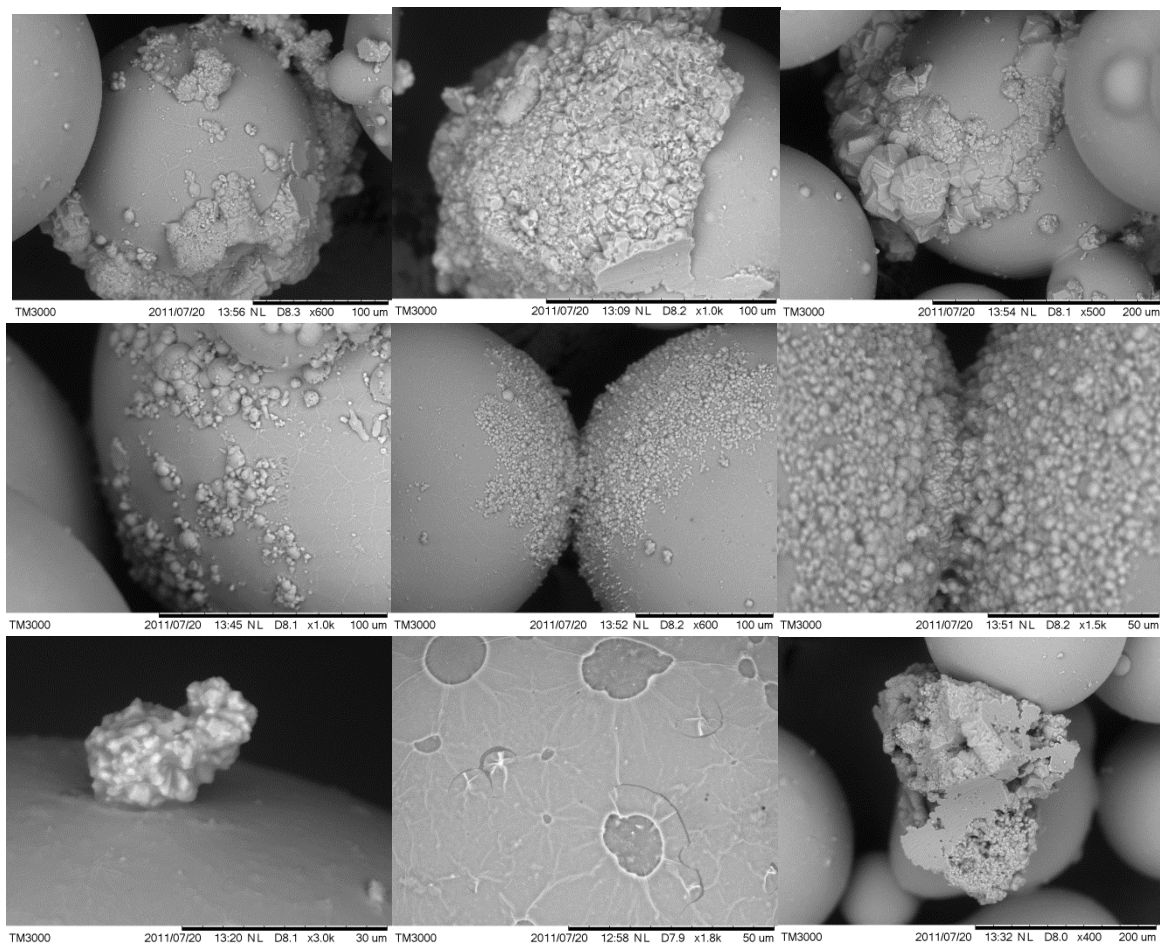
Figure 26: Examples calcium carbonate precipitates formed during the column flow experiment. Note the variety of morphologies formed, including cubic crystals, globular clusters, and sheets. Also featured are examples of precipitates at the contacts of grains and filling the interior pore volume (note flat areas on the precipitate cluster in the lower right and top center image).
