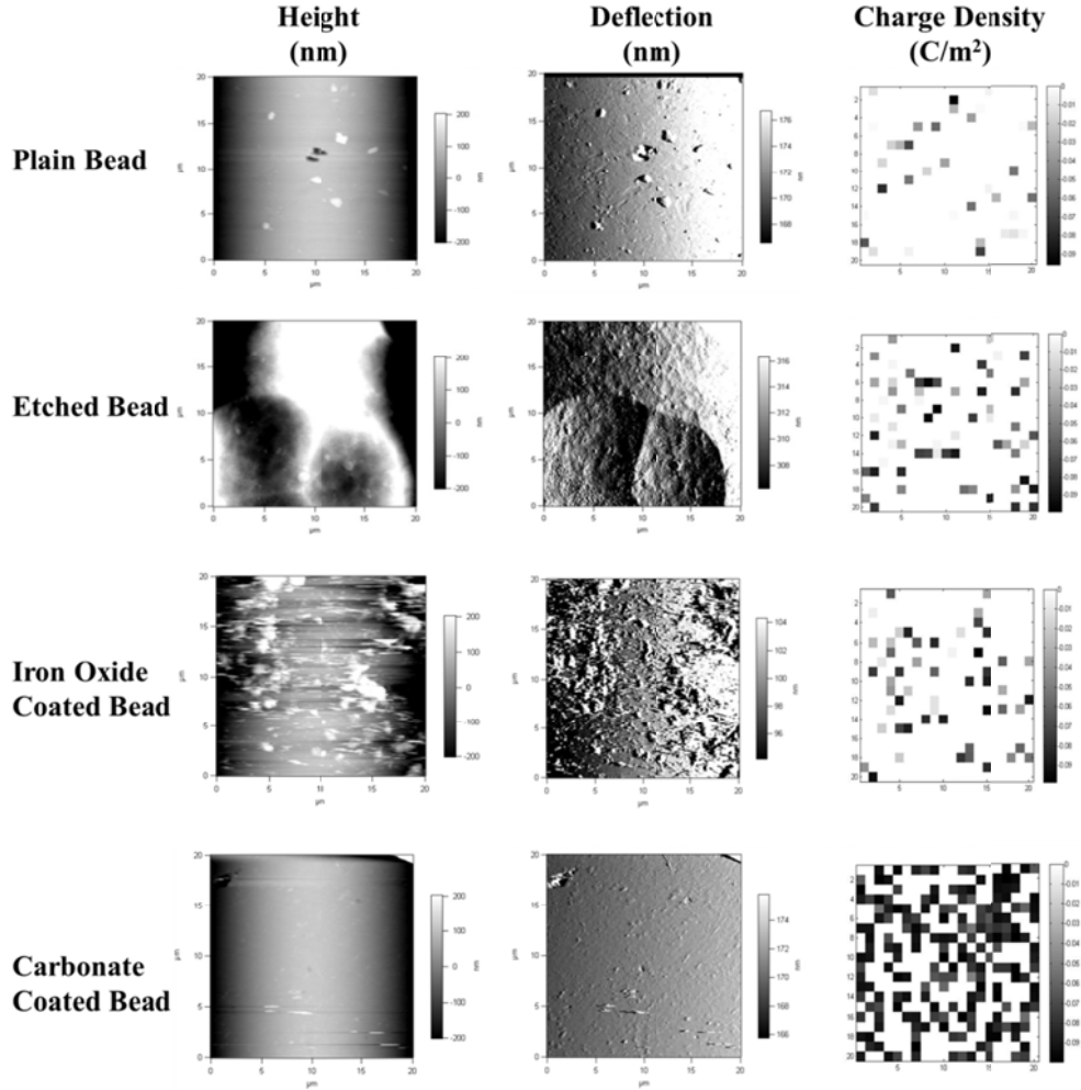
Figure 27: Height (left), Deflection (middle), and corresponding calculated surface charge density (right) of different bead surfaces as measured by AFM in 0.001M NaCl solution using a probe coated with a carboxyl terminated self-assembled monolayer. In solution, the carboxyl groups on the tip dissociate and the tip has a net negative surface charge \sim 0.02 \text{ C/m}^2 . The area of each image is 20 \times 20 \mu\text{m} .
