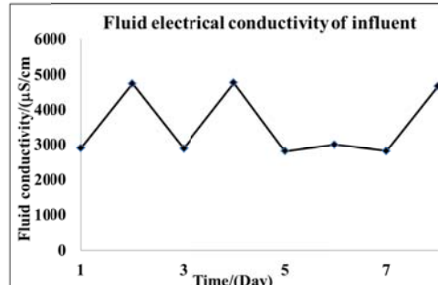
Figure 4: Electrical conductivity of the influent solution throughout the ion exchange experiment. Note the consistency relative to the real conductivity of the column.
