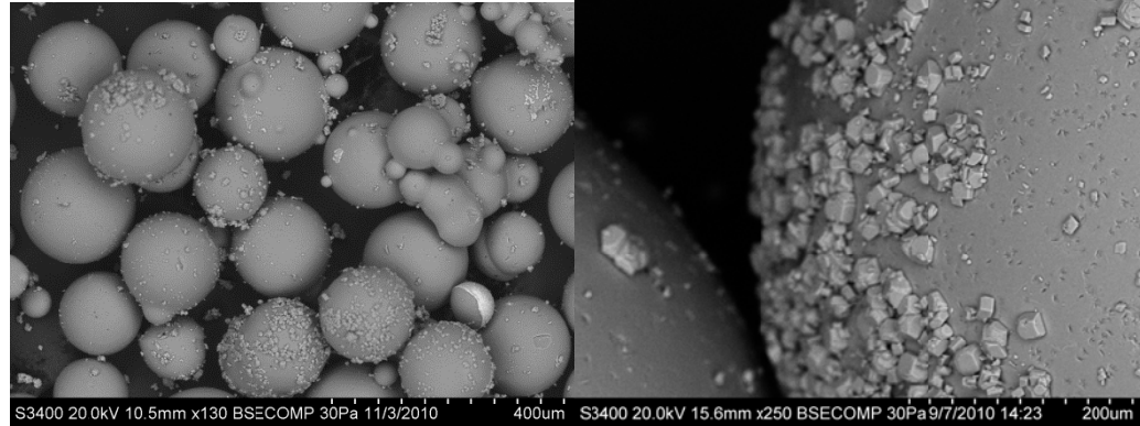
Figure 15: SEM images showing results of different carbonate treatments for glass beads and silica gel.
