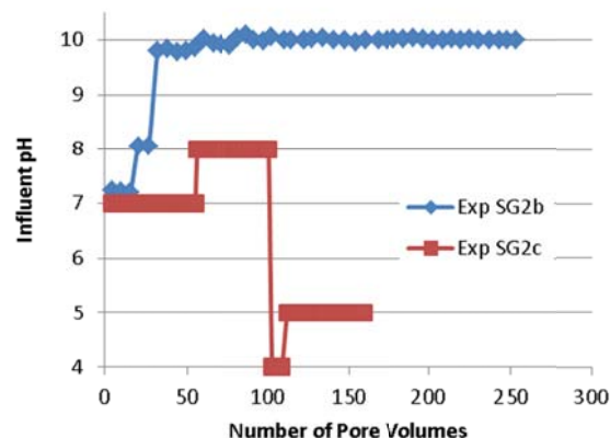
Figure 5: Record of influent pH to column for experiment SG2b and SG2c evaluating the impact of changes in pH on surface site density.
