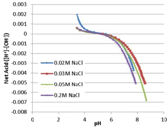
Figure 11: Results for base titration of silica gel at salt concentrations from 0.02-0.2M.
