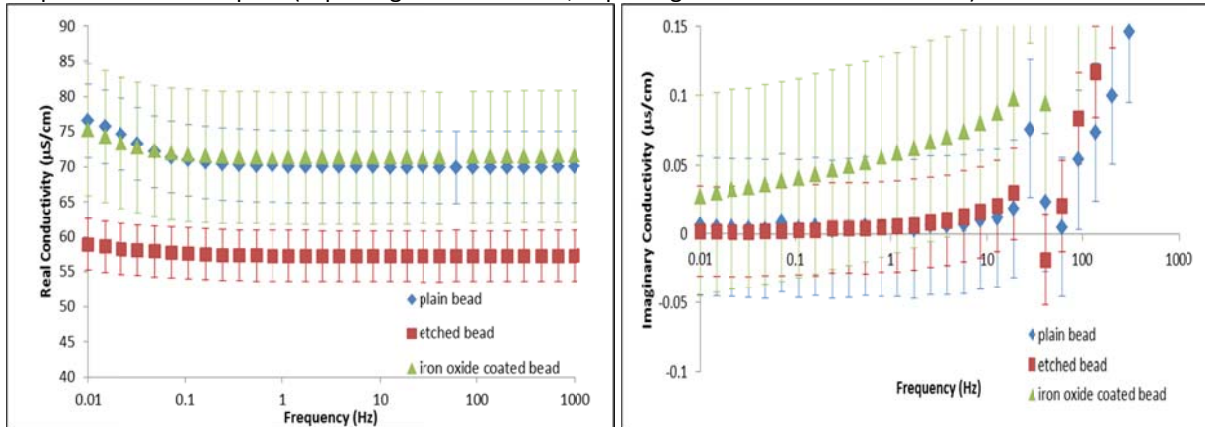
Figure 18: SIP results for glass beads. Note the minor change in real conductivity and lack of polarization response for the samples. (Exp GB2g - etched beads; Exp GB4g – iron oxide coated beads)
