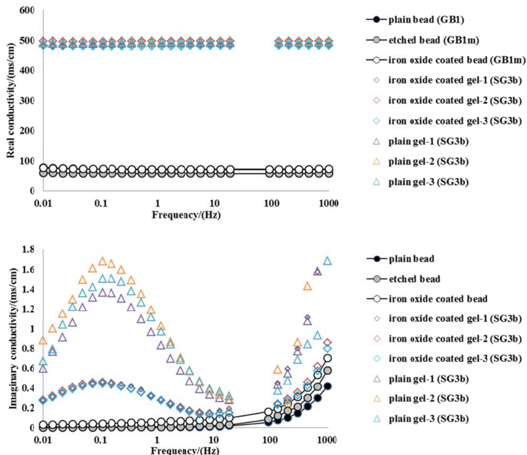
Figure 19: Influence of iron oxide coatings on the imaginary conductivity of glass beads and silica gel. Three replicate measurements from repacked columns are shown for the silica gel to illustrate the variability in the measurements, whereas the average of three independent replicate columns is shown for the glass beads to highlight the difference in the signals. (Note that the difference in real conductivity is because the glass bead measurements were performed with a 1mM NaCl pore filling solution, whereas the solution concentration was 10mM for the silica gel measurements. In other experiments not shown, the concentration did not significantly increase the imaginary response of the glass beads.)
