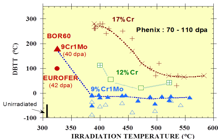
Figure 3: Ductile to brittle transition temperature for F/M steels with different Cr contents as a function of irradiation temperature [5]
