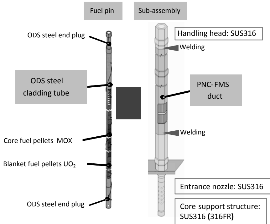
Figure 7: Material selection for fuel assemblies of the JSFR
