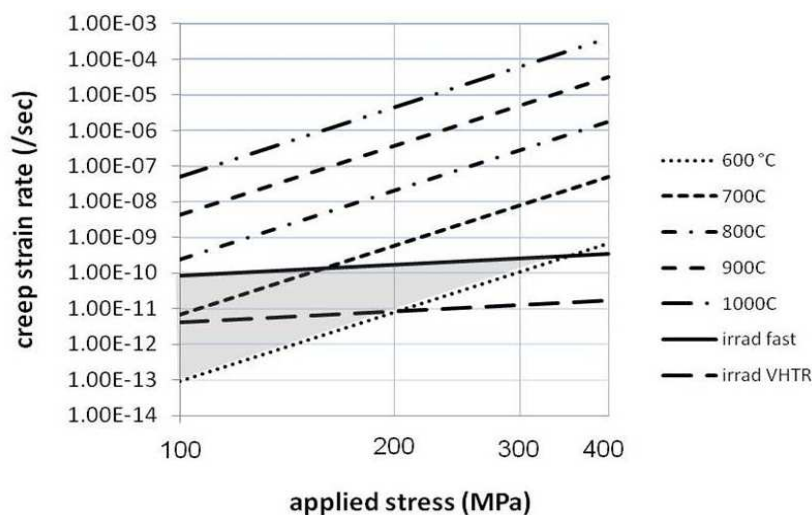
Figure 5: Thermal and irradiation creep rates of TiAl as a function of stress and temperature
