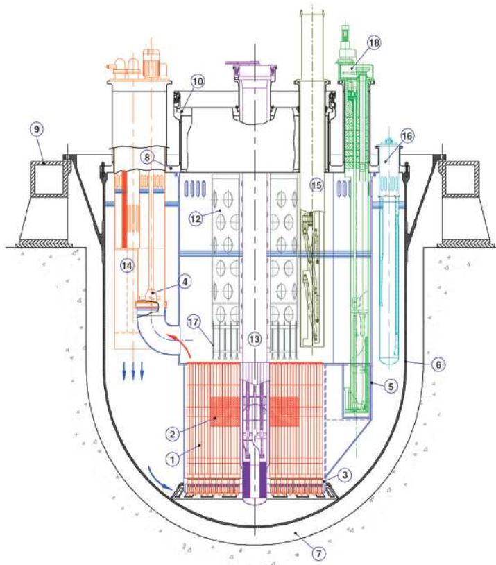
Figure 13: EFIT design and scheme of the primary system
