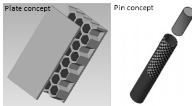
Figure 4: View of GFR fuel
