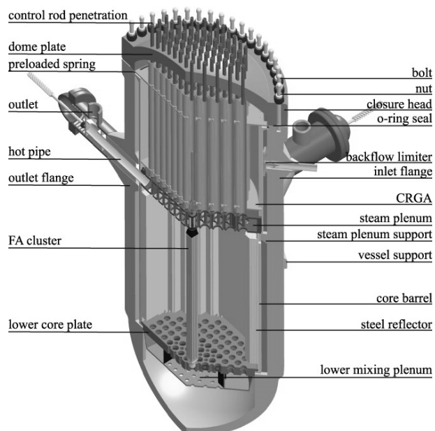
Figure 16: Design of the assembled RPV with internals [3]
