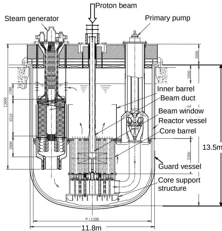
Figure 10: Conceptual design of JAEA's reference ADS
