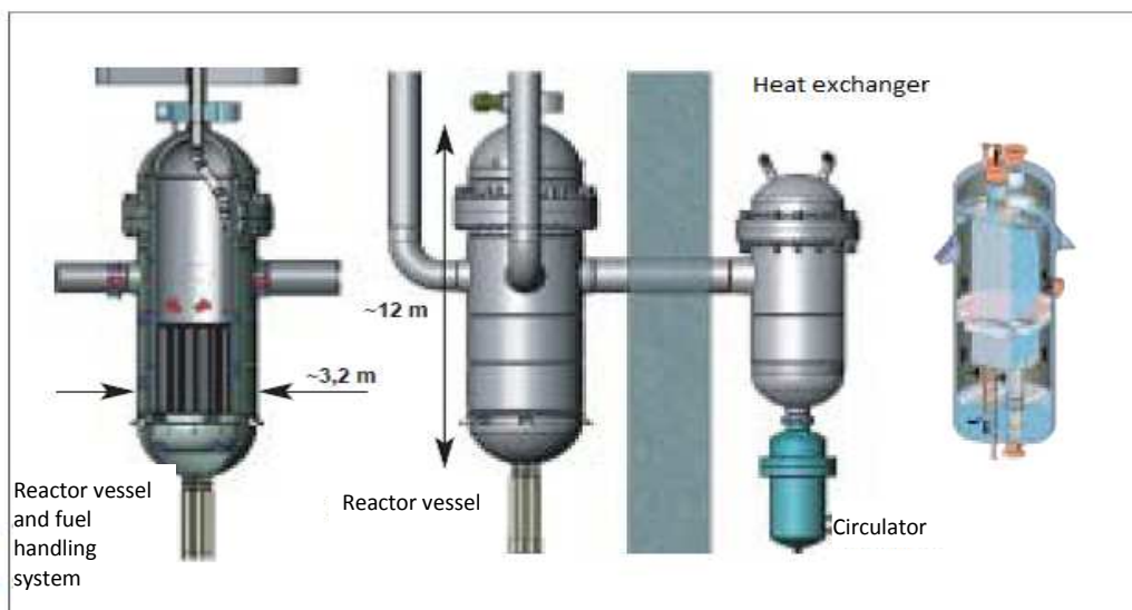
Figure 2: Gas-cooled fast reactor: The ALLEGRO primary system overview [7]
