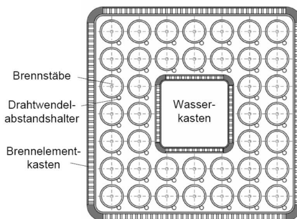
Figure 17: Fuel assembly box
