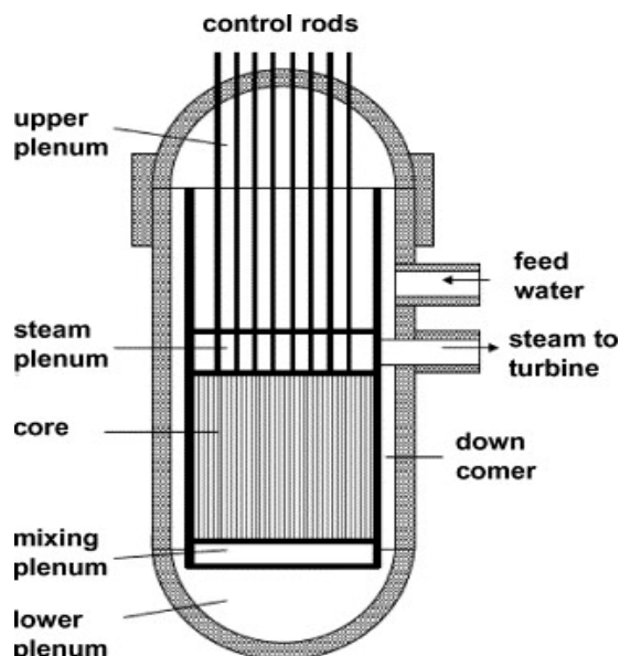
Figure 15: Scheme of the HPLWR [2]
