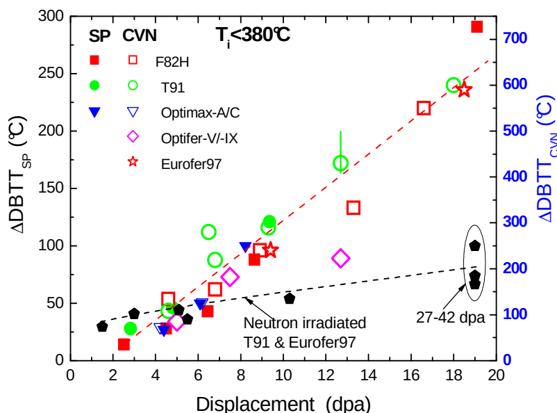
Figure 11: DBTT shift as a function of the irradiation dose for different F/M steels irradiated in the STIP
