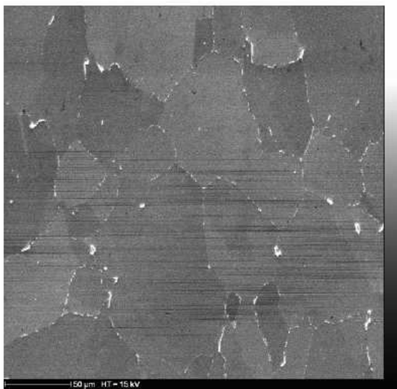
Figure 14: Re-crystallised microstructure of a Ni-W-Cr alloy tailored for usage in contact with fluoride salts (SEM-BSE)
