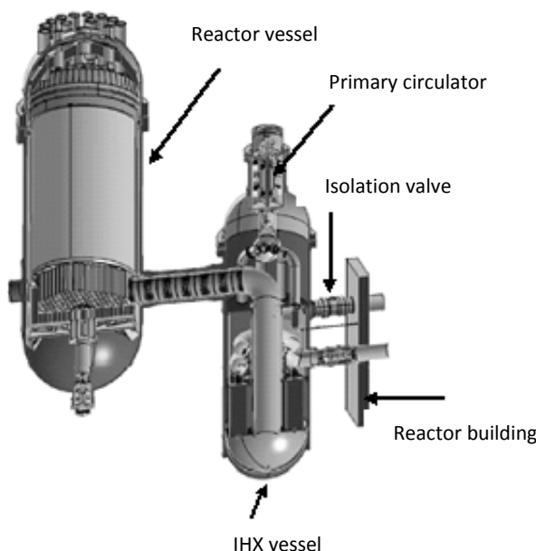
Figure 1: The ANTARES project – HTR (AREVA NP)
