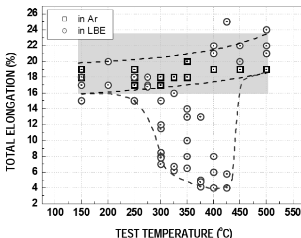
Figure 12: Total elongation versus test temperature for HT760 specimens tested either in Ar or LBE [4]
