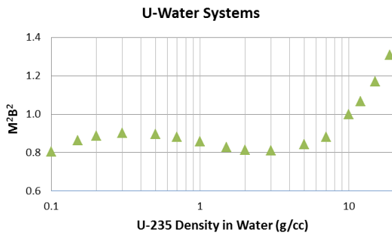
Figure 2. M^2B^2 as a function of the U-235 density in ^{235}\text{U} -Water Systems.
