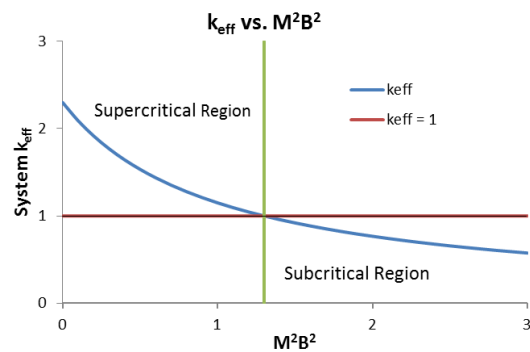
Figure 1. k_{eff} as a function of M^2B^2 .
